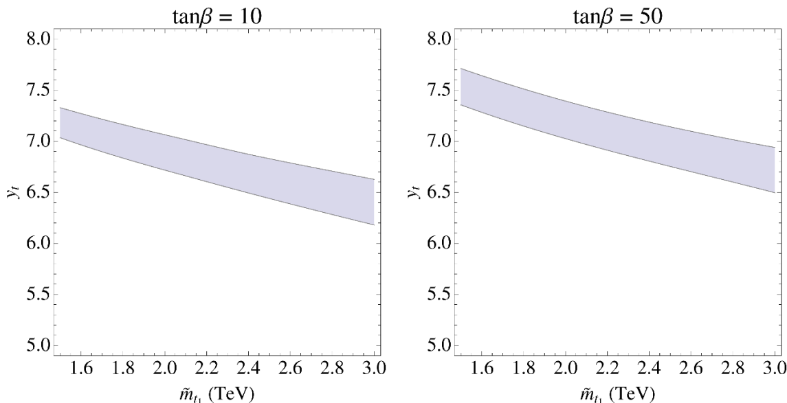
Figure 2. Range of values of y_t giving a stop A -term large enough to account for 124 \text{ GeV} < m_h < 126 \text{ GeV} , plotted as a function of the lightest stop mass \tilde{m}_t for \tan \beta = 10 and \tan \beta = 50 . The plots assume the specific realization of the model-dependent Higgs sector described in section 5.
