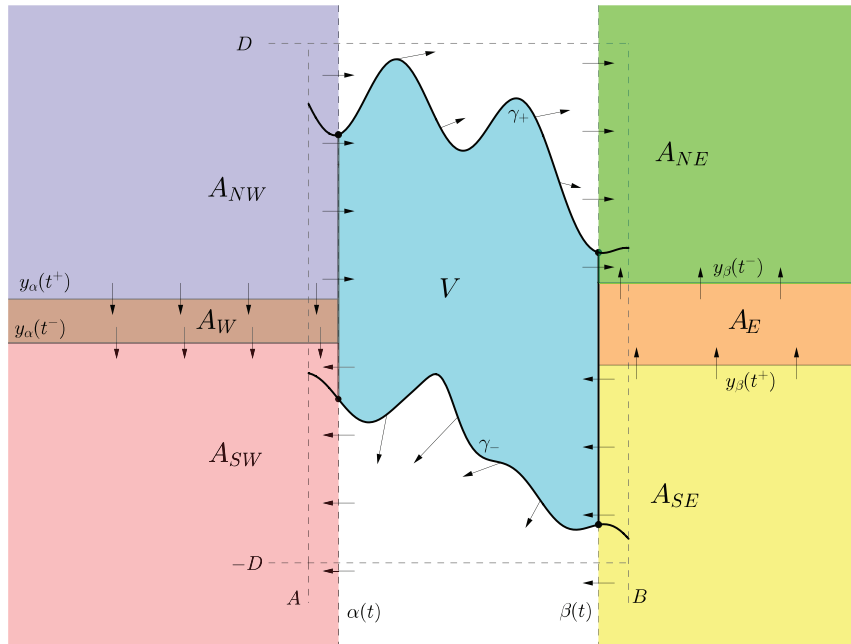
Figure 1: A sketch of the section at a fixed time t of the regions where to study the dynamics of u' = \tilde{\Phi}(t, u) . Notice that the vertical lines x = \alpha , x = \beta and the horizontal lines y = y_\alpha , y = y_\beta move in time, while the curves \gamma_\pm are fixed.
