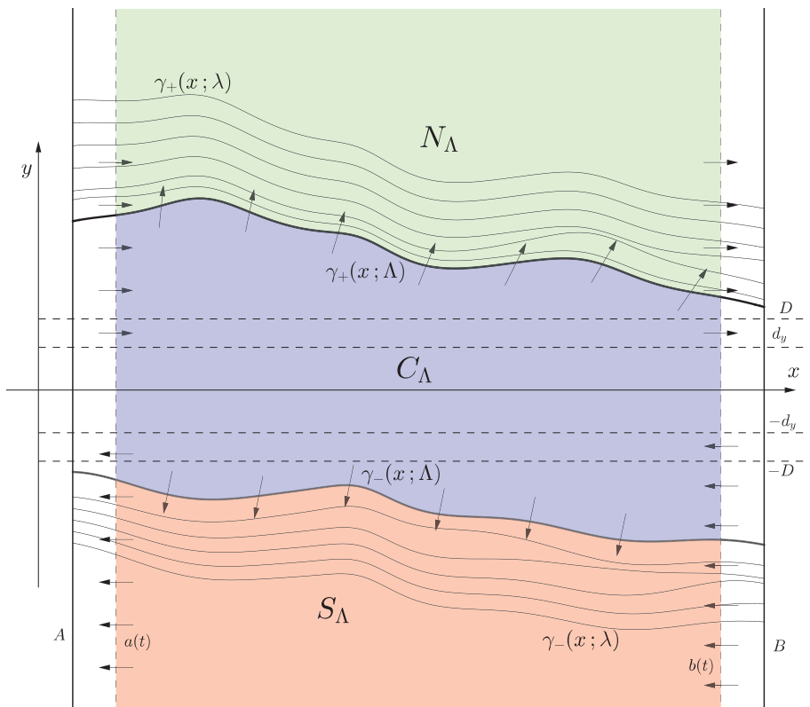
Figure 3: A sketch of the section at a fixed time t of the regions N_{\Lambda} , C_{\Lambda} , and S_{\Lambda} . Notice that the vertical lines x = a and x = b move in time, while the curves \gamma_{\pm}(\cdot, \Lambda) are fixed.
