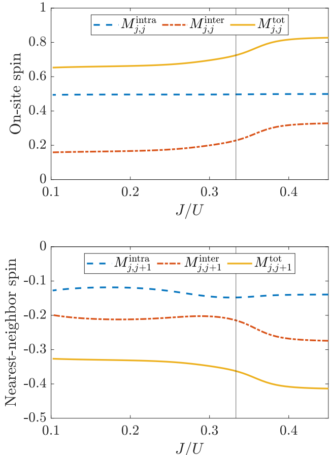
FIG. 7. On-site (upper panel) and first-neighbors (lower panel) magnetic correlations with respect to the control parameter J/U . Model parameters t = 1 , U = 22 , and 6 particles have been used. The vertical gray line corresponds to J/U = 1/3 .
