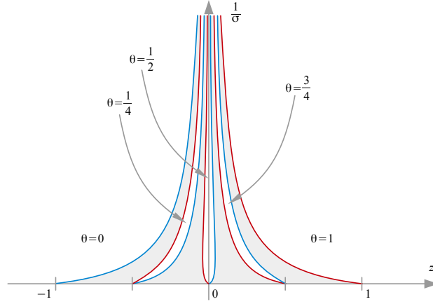
Figure 19: Representation of constancy sets of \theta in the z\text{-}\frac{1}{\sigma} plane
