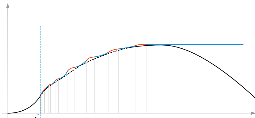
Figure 31: comparison between the graph of the function g_{\text{hom}} (below) and that of Q_{\text{mf}} after subtraction of the quadratic part
