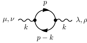
FIGURE 5.1: The relevant Feynman diagram for the computation.
