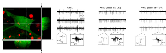
Fig. 7. Confocal fluorescence micrograph of cultured hippocampal neurons (14 DIV), exposed to 40 \mu g/ml FND for 2 days, and stained in green with the cytoplasmic labelling dye (CellTracker™ Green CMFDA). Red emission is from FNDs. The entire field and cross-sections (XZ and YZ) were shown. Representative traces of spontaneous firing at 18 DIV (data from 3 representative MEA channels) under control conditions (CTRL), without FNDs, with FNDs seeded at 7 DIV and at 14 DIV. Insets: higher magnification of single spikes and bursts. (Modified with the permission from Guarina et al., 2018 [176]). (A colour version of this figure can be viewed online.)
