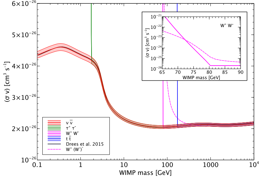
Figure 3. ‘Thermal’ annihilation rate \sigma v of a generic WIMP, as a function of its mass m_\chi , assuming that it only couples to the indicated standard model particles. The width of the band corresponds to the accuracy, at the 2\sigma level, with which the relic density is determined by Planck [1]. The dashed line shows the results for a model with virtual final state particles (see text for details). For comparison, we also show the results by Drees et al [50].
