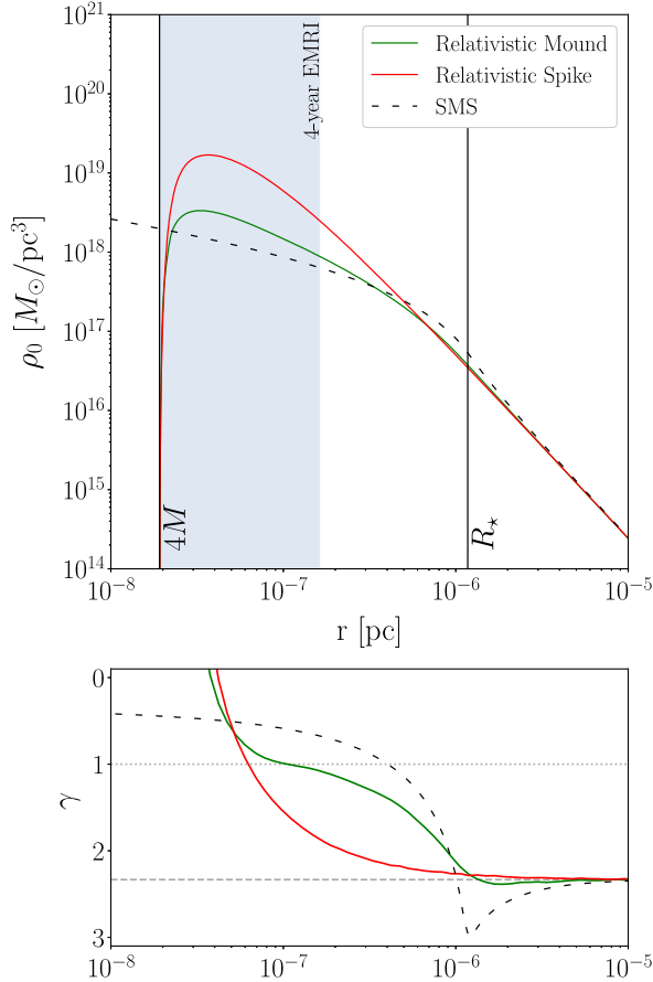
FIG. 1. Top panel: DM rest mass density profile pre- and post-SMS collapse; these are labeled, respectively, by SMS and Relativistic Mound. The case of a SMBH growing adiabatically from a light seed to a mass of 10^5 M_\odot is also shown for comparison and it is labeled Relativistic Spike. Bottom panel: Profile slope, \gamma \equiv -d \log \rho / dr , for each case.
