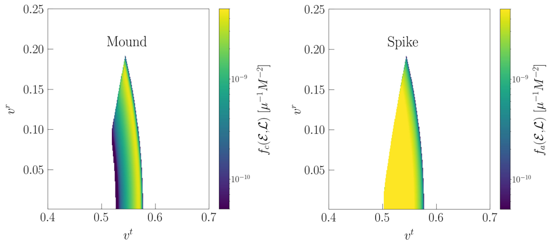
FIG. 3. Left: Distribution function of DM particles in the projected phase space of velocities (radial and tangential) as measured in the LIF at 6M for a spike following OS collapse. Right: Same quantity but for a spike grown adiabatically.
