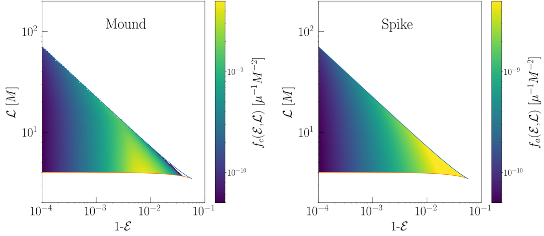
FIG. 2. Left: Coarse-grained distribution function of DM after OS collapse projected in the phase space (\mathcal{L}, 1 - \mathcal{E}) . Right: Same quantity but for a spike grown adiabatically. In both panels, the top blue curve corresponds to circular orbits and the bottom orange curve corresponds to the minimum angular momentum required to avoid capture by the BH for the given energy.
