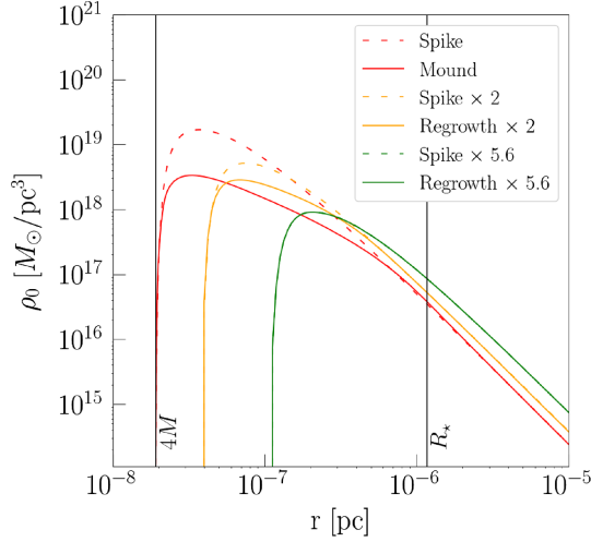
FIG. 4. DM rest mass density profiles after the SMS collapse (Mound) and various factors of regrowth n = M_f/M (Regrowth \times n ). The adiabatic equivalents for the initial BH mass (Spike) and each regrowth factor (Spike \times n ) are also shown as dotted lines.
