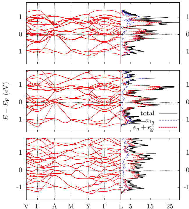
FIG. 4: (Color online) Band structure (left) and projected density of states (right) from GGA of paramagnetic corundum structure \text{V}_2\text{O}_3 with atomic positions determined experimentally for the paramagnetic metallic phase 28 (up), GGA-relaxed atomic positions in the corundum structure (middle) and GGA-relaxed atomic positions allowing for a monoclinic distortion (down).
