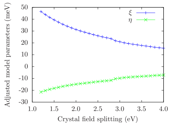
FIG. 18: (Color online) Fitted next-nearest neighbour in-plane hopping parameters \xi and \eta . See text for details.
