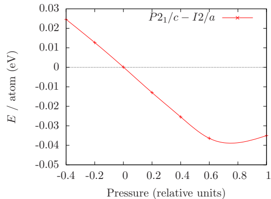
FIG. 5: (Color online) Total energy difference of the P2_1/c and I2/a phases of monoclinic \text{V}_2\text{O}_3 , as a function of the applied pressure. The relative units of the pressure axis correspond to the reported values in the corundum structure at ambient conditions 28 (0.0) and the experimentally reported values of the high-pressure phase transition from I2/a to P2_1/c 29 (1.0).
