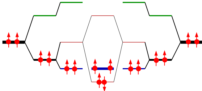
FIG. 2: (Color online) The "dimer" building block of Castellan, Natoli and Ranninger, with its electronic configuration.
