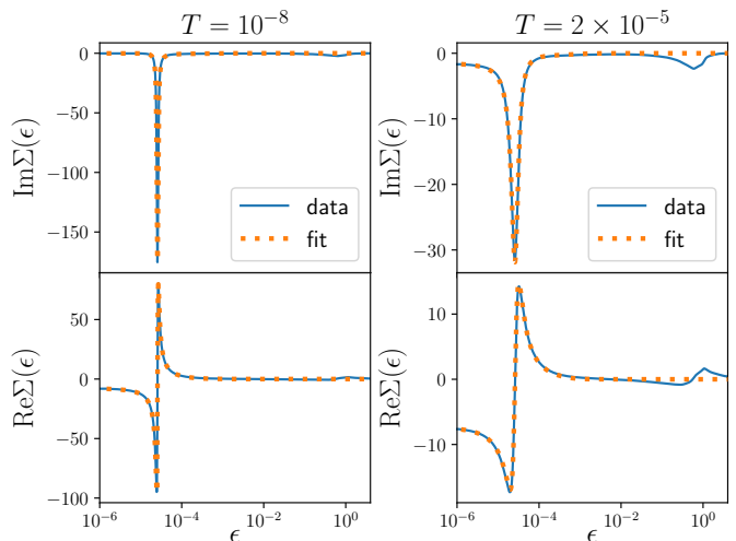
FIG. 7. Real and imaginary parts of the retarded self-energy at U = 2 , \epsilon_d = 0.1 and temperatures T = 10^{-8} , left panels, and T = 2 \times 10^{-5} , right panels, together with the ansatz (58) with fitted parameters (dotted lines).
