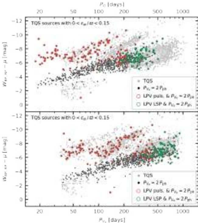
Fig. 32. Similar to the right-hand side panels in Fig. 30, but with the sources having P_{VR} \approx 2P_{ph} highlighted in black. The PLD constructed with P_C is shown in the top panel and the one constructed with P_{VR} in the bottom panel for the TQS sources with parallax errors better than 15% (gray symbols), and highlighting the sources with P_{VR} \approx 2P_{ph} . Red and green circles indicate LPVs showing pulsation and a LSP, respectively. Only five of them are identified as C-rich.
