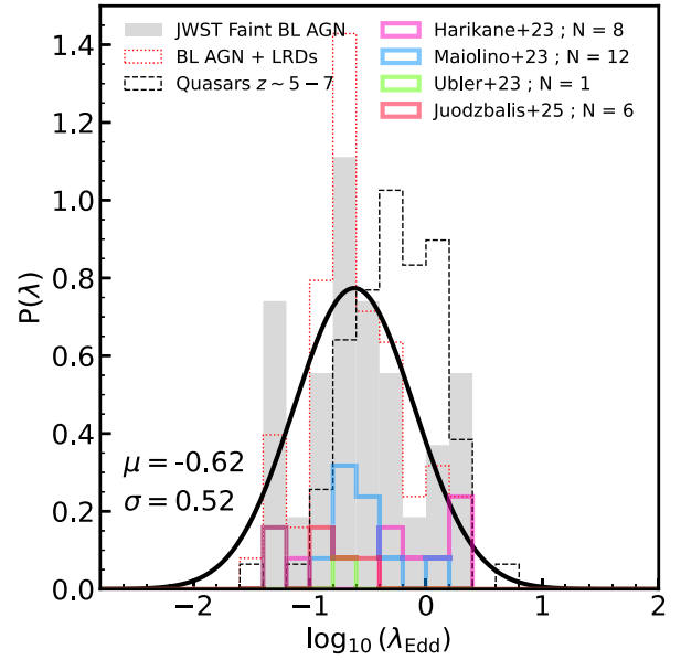
Figure A1. The distribution of Eddington ratios for our sample of faint BL AGNs observed by JWST (grey histogram), as well as the distributions of the sample broken down by source paper (coloured histograms), compared to a sample of quasars at z \sim 5 - 7 (black dashed histogram) obtained from C. J. Willott et al. (2010); B. Trakhtenbrot et al. (2011); Y. Matsuoka et al. (2019); M. Onoue et al. (2019); Y. Shen et al. (2019), as well as a BL AGN + LRD sample (with the LRDs from J. E. Greene et al. 2024; D. D. Kocevski et al. 2024; J. Matthee et al. 2024, red dotted histogram). The best-fitting Gaussian to our BL AGN sample is denoted by the solid black line which has a mean of \langle \log_{10}(\lambda_{\text{Edd}}) \rangle = -0.62 and a dispersion of \sigma_{\lambda_{\text{Edd}}} = 0.52 . Whereas, if we fit the combined BL AGN + quasar sample we find the best-fitting values \langle \log_{10}(\lambda_{\text{Edd}}) \rangle = -0.35 , \sigma_{\lambda_{\text{Edd}}} = 0.50 (broadly consistent with the mean \lambda_{\text{Edd}} values at z \sim 4 - 5 found by W. He et al. 2024; S. Lai et al. 2024). The ERDF assumed in Section 4.2 is chosen to agree with the BL AGN + quasar sample. We note that several papers derive both the black hole mass and bolometric luminosity from the broad component of the H\alpha line, which can lead to spurious correlations. However, the two properties have differing dependencies, with the BH mass primarily dependent on the width and not the luminosity.
