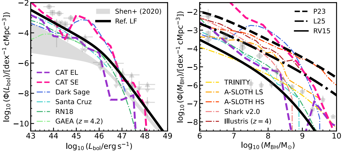
Figure E1. Left: A comparison of our reference LF (black solid line), the X. Shen et al. (2020) LF (grey shaded region), and the observational data from Fig. 1 with the CAT Eddington-limited model (dashed purple line), CAT super-Eddington model (dashed pink line) and several other theoretical models at z \sim 5 (dot-dashed lines). From this comparison, we see that our adopted reference luminosity function is broadly consistent with the predictions of semi analytic models. Right: A comparison of the BHMFs inferred from the P23, L25, and RV15 M_{\text{BH}} - M_{\star} relations (black lines) and the observational data shown in Fig. 5 with the CAT Eddington-limited and super-Eddington models, as well as several other theoretical models (dot-dashed lines). From this comparison, we observe that the predicted BHMFs from theoretical models span the region between the RV15 and P23-based BHMFs. The other theoretical models included are DARKSAGE (A. R. H. Stevens, D. J. Croton & S. J. Mutch 2016), the Santa Cruz SAM (R. S. Somerville & J. R. Primack 1999; A. Gabrielpillai et al. 2022), the SAM of A. Ricarte & P. Natarajan (2018, RN18), GAEA (F. Fontanot et al. 2020), TRINITY (H. Zhang et al. 2023), the A-SLOTH light and heavy-seeding models (J. Jeon et al. 2025b), SHARK v2.0 (C. d. P. Lagos et al. 2018, 2024), and the Illustris simulation (D. Nelson et al. 2015; D. Sijacki et al. 2015).
