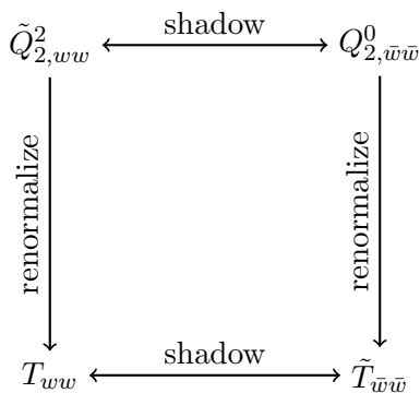
Figure 3. The shadow [59] and renormalization [29] procedures commute. The renormalized quantities \{T_{ww}, \tilde{T}_{\bar{w}\bar{w}}\} correspond to soft charges appearing in [8] and [32], respectively.
