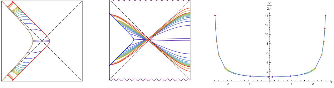
FIG. 26. Left and central panels: extremal surfaces in the dS and in the AdS portion of the Penrose diagram, respectively. Right panel: plot of the volume as a function of boundary time t_b . We set \alpha_t = 1 , see eq. (V.3), and we choose \kappa = 0.2 , \lambda = 1.5 , \mu = 0.4 , and \epsilon = 0.06 .
