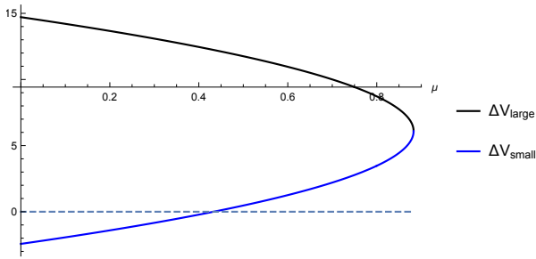
FIG. 25. Plot of \Delta\mathcal{V}_{\text{small}} and \Delta\mathcal{V}_{\text{large}} in eqs. (IV.28) and (IV.29) as functions of \mu , for \lambda = 1 and \kappa = 0.5 .
