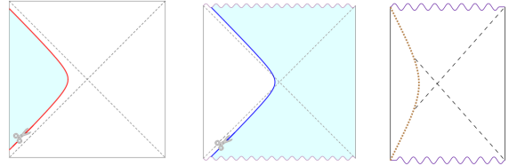
FIG. 3. Penrose diagrams for a not so small bubble \mu_s < \mu < \mu_0 .
