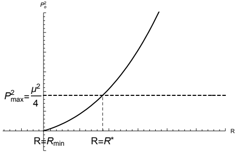
FIG. 18. Behavior of P_o^2(R) in eq. (IV.5) for large bubbles.
