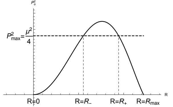
FIG. 11. Behavior of P_o^2(R) in eq. (IV.5) for small bubbles.
