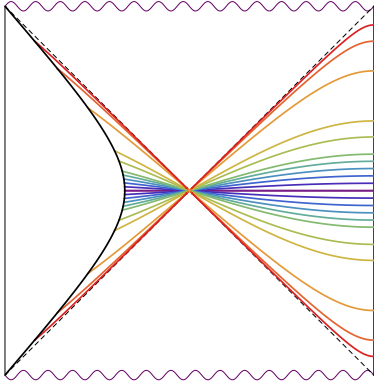
FIG. 22. AdS portion of the extremal solution for the static bubble (which is shown in the black solid line). These surfaces have all P_o = 0 and never enter the black and white hole regions of the geometry.
