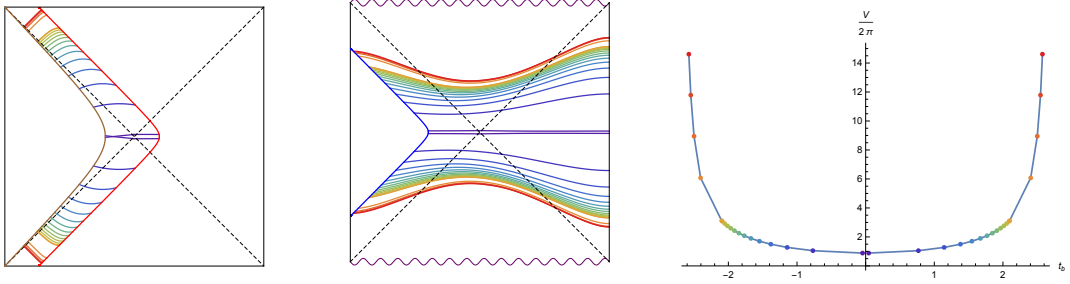
FIG. 27. Plots of the same quantities as in figure 26, with the choice \alpha_t = -1 .
