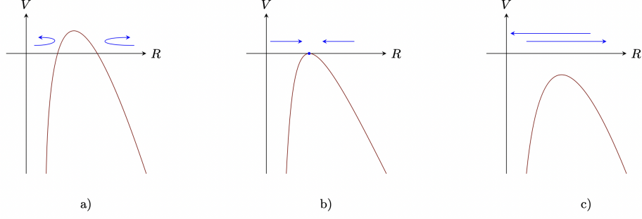
FIG. 7. Qualitative plots of the effective potential V(R) in eq. (II.14) with positive (plot a), vanishing (plot b) and negative (plot c) maximum. Blue arrows represent the possible evolution of the bubble radius R(\tau) .
