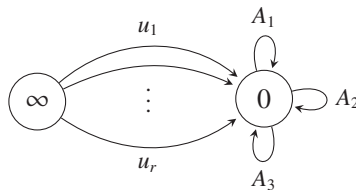
Figure 1. The r -framed 3-loop quiver \widetilde{\mathbb{L}}_3 .
