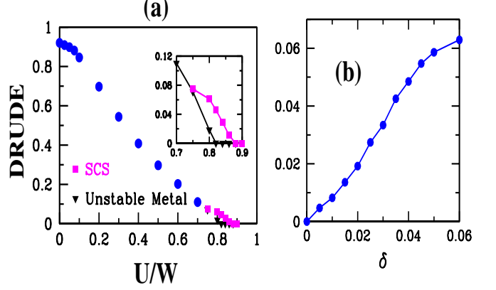
FIG. 4: (Color online) (a) Drude weight at half-filling as function of U/W . In the SCS region is also shown the Drude weight of the metastable normal solution, zoomed in the inset; (b) Drude weight at U = 0.92 W as function of doping.
