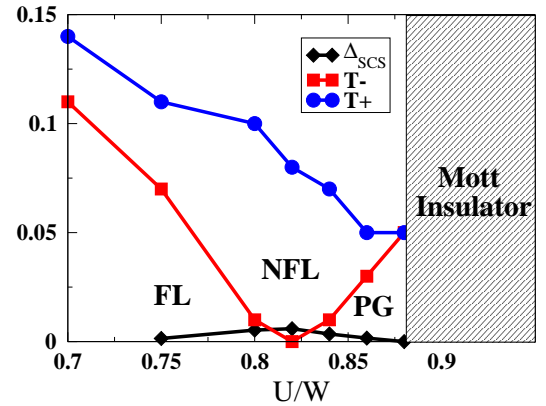
FIG. 7: (Color online) Fitting parameters T_+ and T_- of the DMFT normal self-energy with the expression Eq. (ansatz-DMFT-Sigma) using for the impurity Green's function Eq. (19). We also draw the DMFT superconducting gap when gauge symmetry breaking is allowed.
