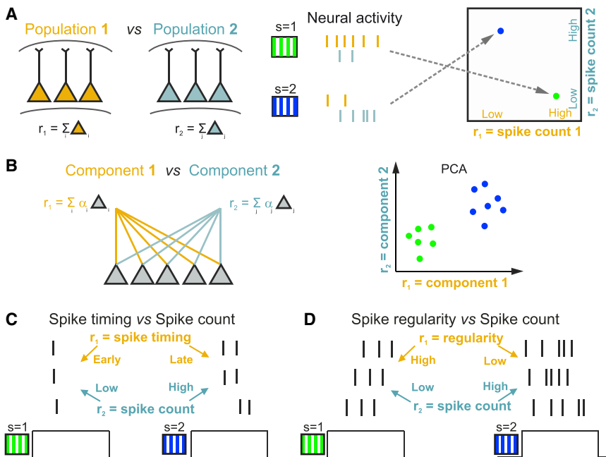
Figure 2. Schematic of Possible Pairs of Neural Population Features Involved in Sensory Perception
