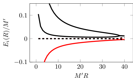
(a) First three energy levels in the theory for (\zeta', \zeta) = (0, 3.67) . The solid lines represent the real part of the energy while the dashed lines represent the imaginary part. The ground state is highlighted in red.
