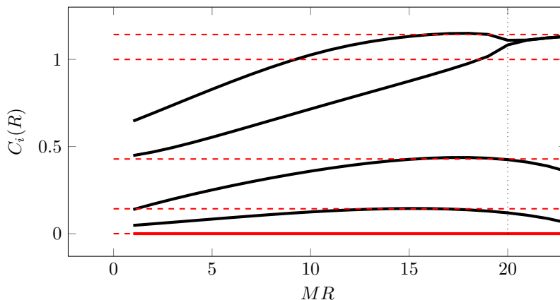
Figure 17. Solid lines show the scaling functions C_i(R) = (E_i(R) - E_0(R))R/4\pi corresponding to the real parts of the first five energy levels at the couplings in eq. (5.10), while the red dashed lines are the predictions from the minimal model \mathcal{M}(2, 7) .
