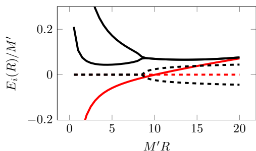
(a) First three energy levels in the theory for (\zeta', \zeta) = (-31.62, 1.90) . The solid lines represent the real part of the energy while the dashed lines represent the imaginary part. The ground state is highlighted in red.
