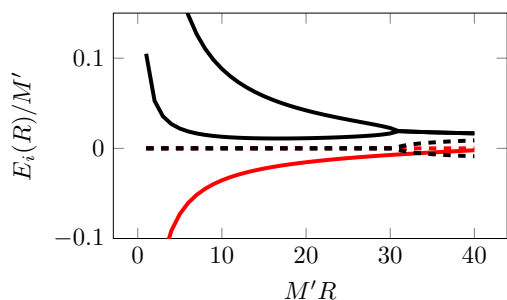
(a) First three energy levels in the theory for (\zeta', \zeta) = (3.17, 0) . The solid lines represent the real part of the energy while the dashed lines represent the imaginary part. The ground state is highlighted in red.
