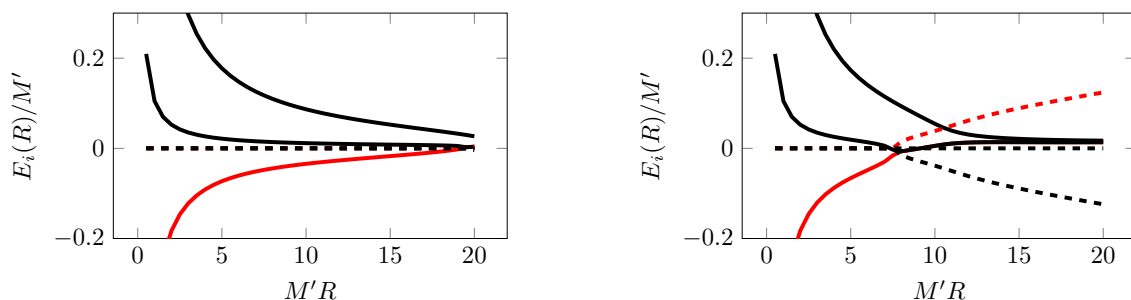
(a) First three energy levels in the theory for (\zeta', \zeta) = (3.16, 18.60) . The solid lines represent the real part of the energy while the dashed lines represent the imaginary part. The ground state is highlighted in red.
