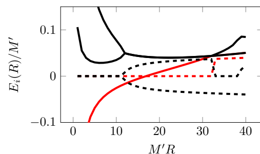
(b) First three energy levels in the theory for (\zeta', \zeta) = (7.93, 0) . The solid lines represent the real part of the energy while the dashed lines represent the imaginary part. The ground state is highlighted in red.
