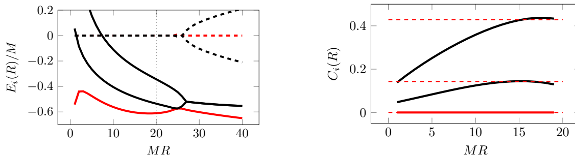
(a) Solid/dashed lines depict the real/imaginary parts of the first three energy levels as a function of the volume at the couplings (5.10), with the ground state highlighted in red. The dotted vertical line indicates the end of the physical window.
