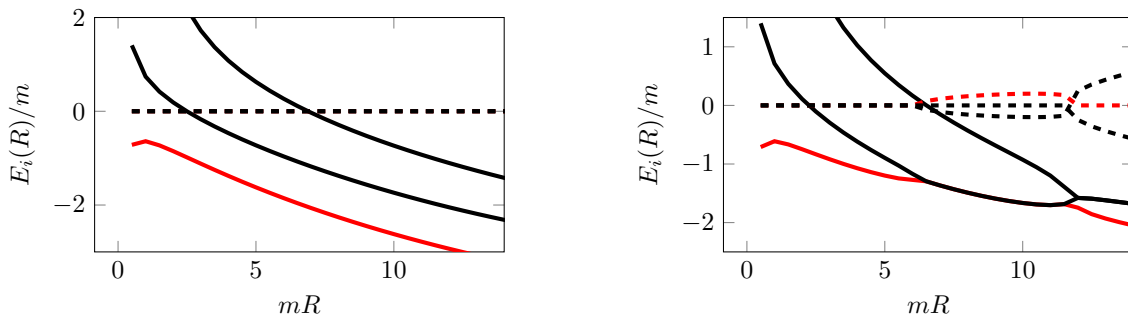
(a) First three energy levels in the theory for \xi = 0.1 < \xi_c at level cut-off N_{\max} = 18 . The solid lines represent the real part of the energy while the dashed lines represent the imaginary part, with the ground state highlighted in red.
