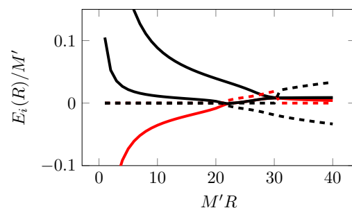
(b) First three energy levels in the theory for (\zeta', \zeta) = (0, 9.17) . The solid lines represent the real part of the energy while the dashed lines represent the imaginary part. The ground state is highlighted in red.
