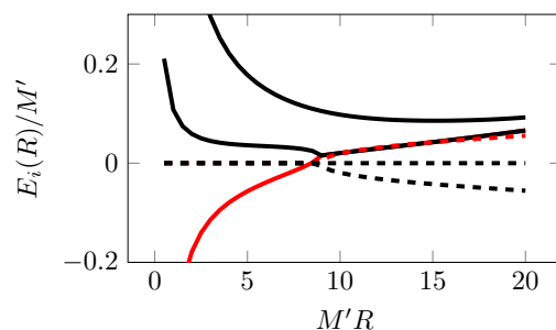
(b) First three energy levels in the theory for (\zeta', \zeta) = (-31.62, 5.69) . The solid lines represent the real part of the energy while the dashed lines represent the imaginary part. The ground state is highlighted in red.
