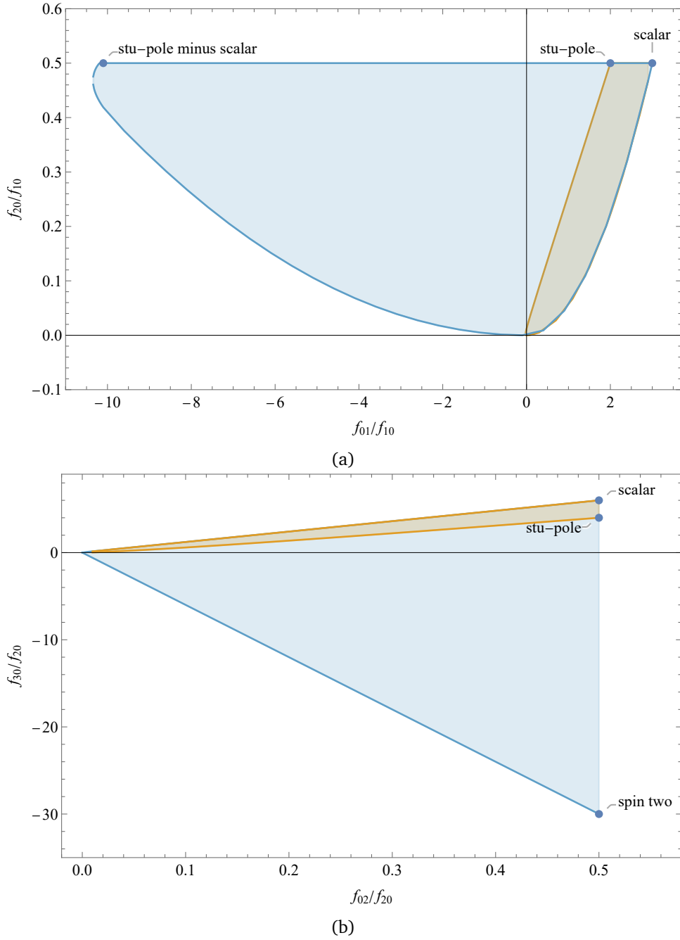
Figure 1: Allowed regions for the real scalar theory for d = 4 . We see that zero-subtracted dispersion relations (orange/smaller) give stronger bounds and a smaller allowed region than doubly-subtracted (blue/larger).
