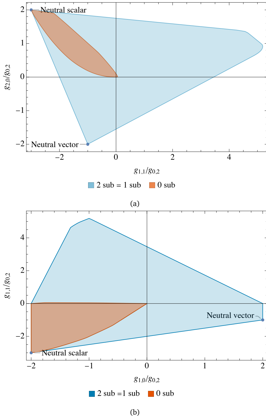
Figure 2: Allowed regions from forward-limit bounds for d = 4 . We can see that the bounds obtained for one and two subtractions are almost identical. The bounds obtained from zero-subtracted dispersion relations are much stronger, however.
