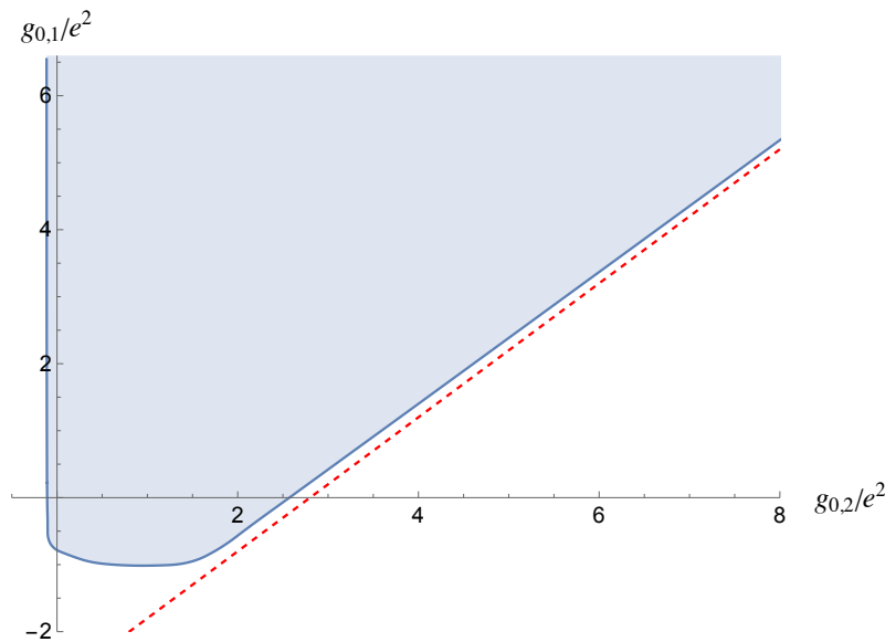
Figure 10: Allowed values for the coefficients g_{0,2} , g_{0,1} normalized to the gauge constant e^2 in d = 5 dimensions. The shaded region is allowed, assuming 1SDR and t -channel dominance.
