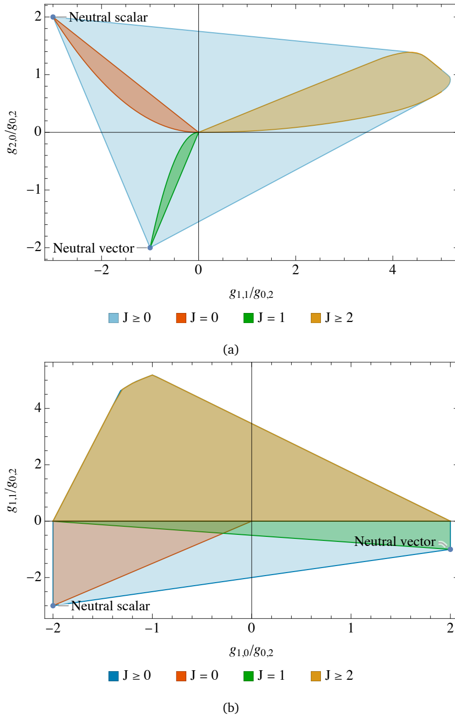
Figure 3: Allowed regions from forward-limit bounds for d = 4 (assuming 2SDR) requiring positivity only on a subset of spins. The full allowed region is the convex hull of solutions obtained using only scalars, only spin-1 or J \geq 2 .
