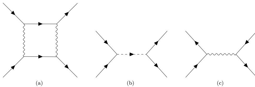
Figure 4: Contributions to \rho^{(2)} can include (a) exchange of neutral states through loops or (b) exchange of a charge-two state. The t -channel dominance assumption is that these are suppressed relative to \rho^{(0,\pm)} , which can be generated by neutral states at tree level (c).
