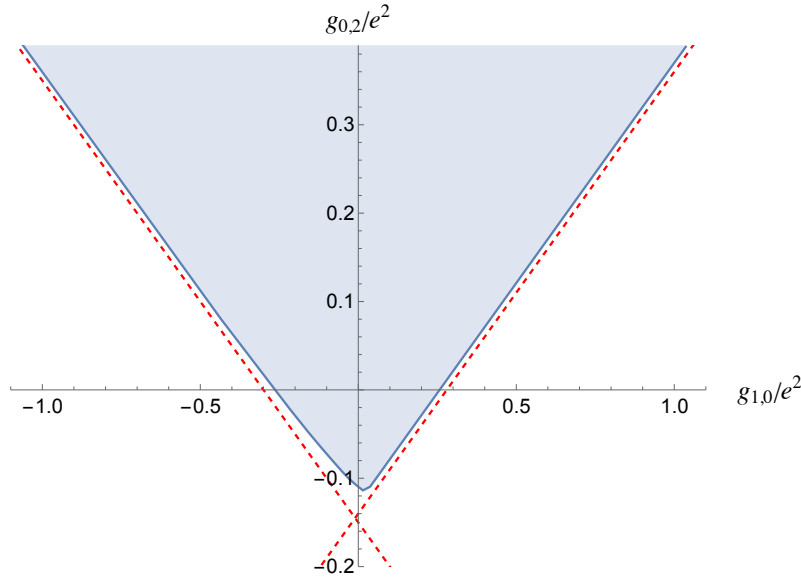
Figure 9: Allowed values for the coefficients g_{1,0} , g_{0,2} normalized to the gauge constant e^2 in d = 5 dimensions. The shaded region is allowed, assuming 1SDR and t -channel dominance.
