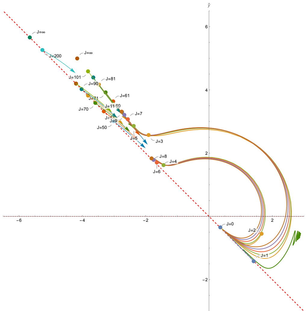
Figure 11: Curves in the plane (\hat{x}, \hat{y}) defined in (109). This is essentially a two-dimensional projection of the functionals defined in (104). The fact that all points lie in the same half of the plane implies that their sum is positive (when dotted with an appropriate vector), which in turn implies that a corresponding low-energy combination is positive via the sum-rules. This leads to the bound (97). See the text for a full description.
