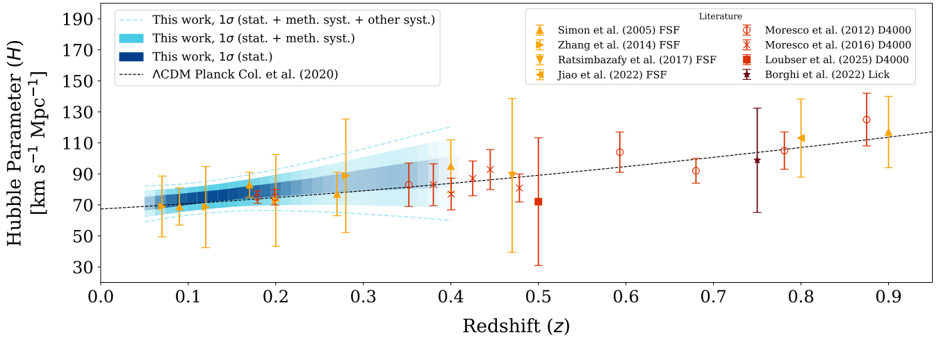
Fig. 9. Reconstruction of the Hubble parameter. Our sampling is shown in shades of blue, corresponding to the posterior distribution obtained for H_0 , q_0 , and j_0 from Fig. 6. The width of the tendency represents the range between the 16th and 84th percentiles of our posterior sampling. The opacity of the colour shade represents the reliability of the H(z) measurement, which we based on the amount of sources (individual galaxies) at each z . The dashed black line represents the H(z) evolution according to Planck Collaboration VI (2020). The plot is extended up to z = 0.9 in order to show the result at the lowest redshift obtained through the Lick indices fit (dark red), by Borghi et al. (2022b). Other measurements from the available literature are represented in yellow (obtained through FSF) and orange (obtained through the measurement of D4000 of its narrow counterpart D4000 n ).
