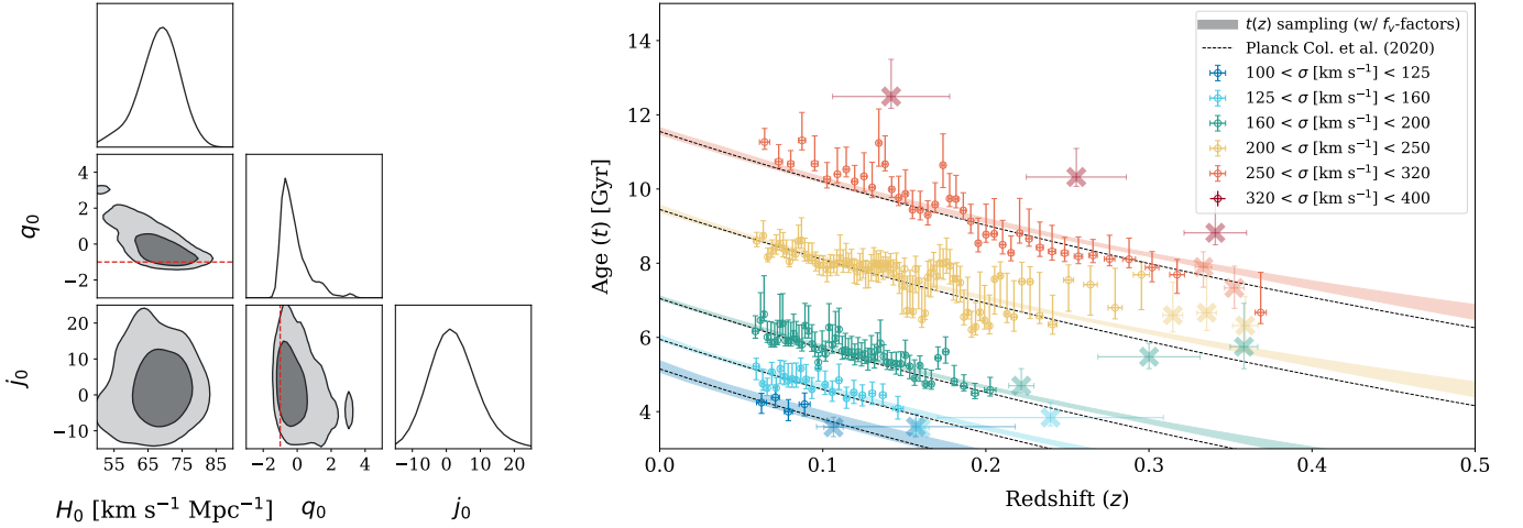
Fig. 6. Joint cosmographic fit of t(z) with ages estimated using the TMJ model. On the left, the corner-plot for the posterior probability distributions of H_0 , q_0 , and j_0 is shown, displaying 1\sigma and 2\sigma contour levels. On the right, the t - z dispersion is shown. The empty circles in strong colour represent the data points we used for the fit, while the faded crosses represent the points, resulting from a set of galaxies with average dispersion in redshift greater than 0.01. The shaded regions in the same colour as the data points are the 1\sigma of the sampling of the posterior distribution coming from the parameters on the left. The zero-ages of the velocity dispersion groups are not shown here, but we refer to the corner plot in Fig. B.2; however, they are used for the sampling and to set a zero-age for the Planck Collaboration VI (2020) evolution of t(z) , shown as dashed black lines. The dashed q_0 = -1 lines in the corner plots for the planes q_0 - H_0 and j_0 - q_0 represent the natural limit imposed by dH/dz > 0 . This is the baseline t - z relation referred to in this work.
