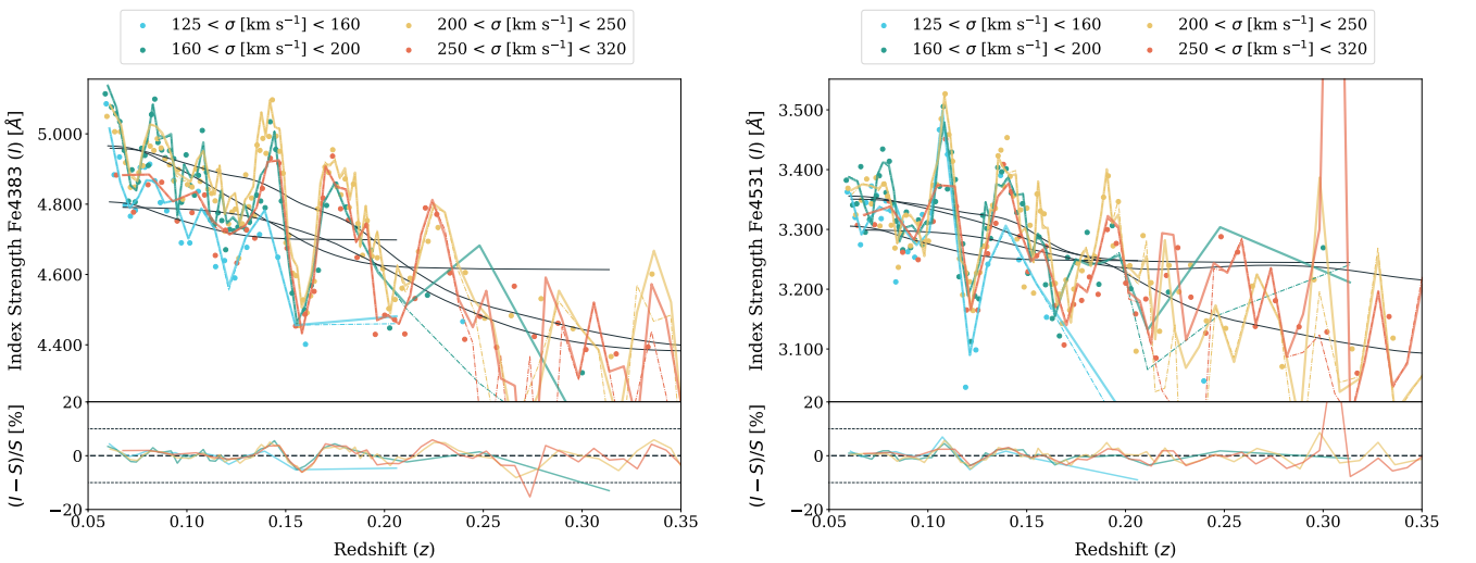
Fig. D.2. Index-redshift relation for Iron lines Fe4383 (left) and Fe4531 (right). The structure of each panel is equivalent to Fig. 13.
