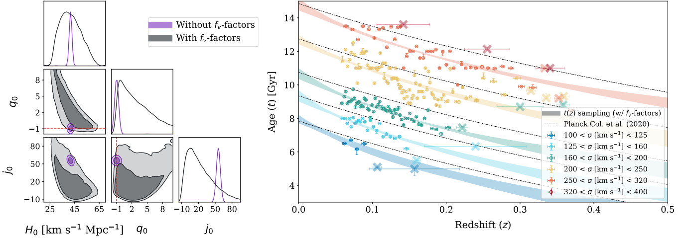
Fig. 8. t - z relations for the ages estimated using the Knowles model. The structure of this figure is the same as that in Fig. 6. The grey contours represent the case with f_v factors included, to account for the possible underestimation of age uncertainties. The t - z samplings on the right panel refer to this case. The contours in purple represent the case where these factors were not taken into account. The sampling of the associated posterior for t - z is not represented on the right panel for this case.
