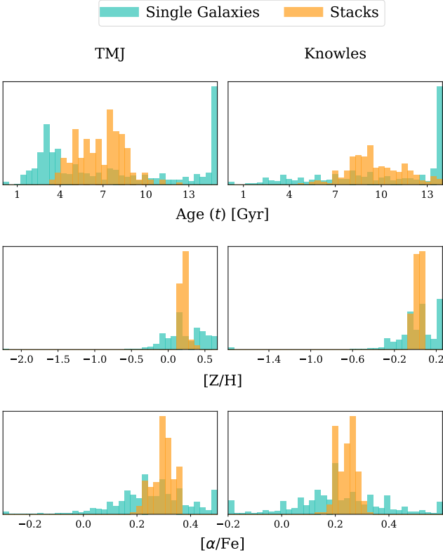
Fig. 5. Age, metallicity, and \alpha -enhancement distributions for the TMJ (left panels) and Knowles (right panels) models, interpolated to a grid of 50 points in each parameter within the original ranges. Results are shown for the Lick index fitted to both single galaxies (in blue) and stacks (in yellow) of the final cosmic chronometer sample.
