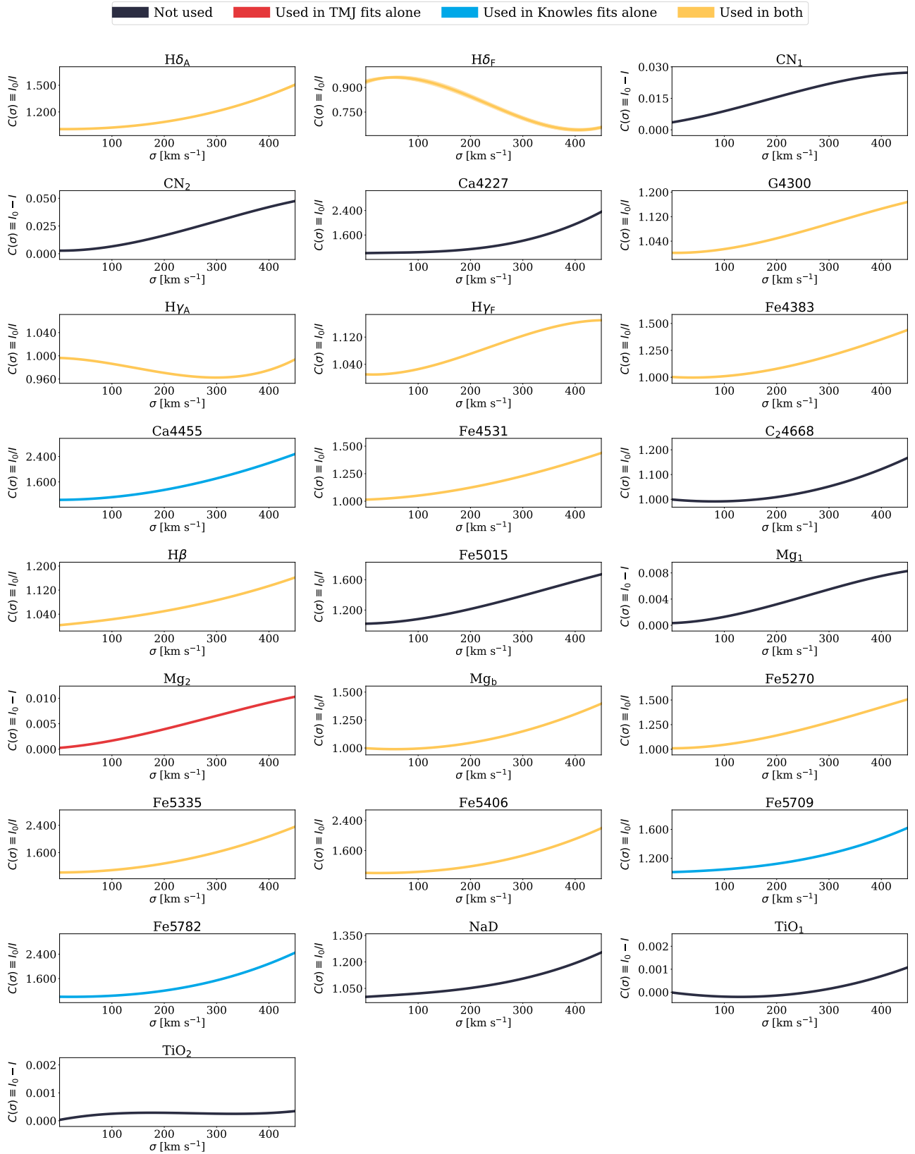
Fig. A.3. Velocity dispersion correction functions C(\sigma, \sigma_{\text{IR}}) for the 25 Lick indices. Yellow lines were chosen to represent the indices that were used for the fit with the two SPS models, while blue and red indicate those that were used only with one of them (Knowles and TMJ, respectively). Grey tendencies represent the corrections for the indices that were not used with any of the models.
