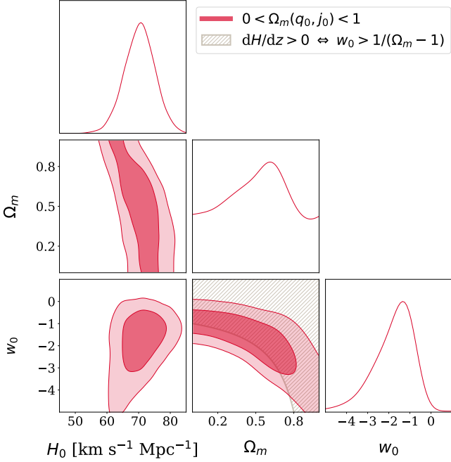
Fig. 7. Posterior probability distribution for H_0 , \Omega_m , and w_0 . The sampled parameters were q_0 and j_0 , then converted to w_0 CDM parameters through Equations (18) and (19). The sampling was run under the \Lambda CDM-model condition of 0 < \Omega_m(q_0, j_0) < 1 . The brown hatched region in the \Omega_m - w_0 plane represents the region allowed by dH/dz > 0 \Leftrightarrow w_0 > 1/(\Omega_m - 1) .
