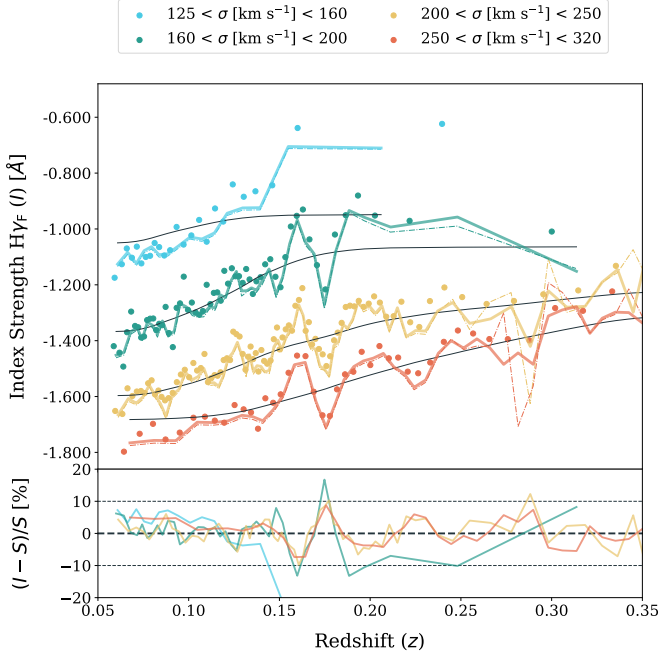
Fig. 13. H\gamma_F trend with redshift. The measurements from the stacks are shown as data points, coloured by the corresponding velocity dispersion bin according to the colour code used in previous figures. The solid black lines represent the global trend via smoothed moving means, while the solid coloured lines are our measurements for single galaxies. The results from the SDSS database are depicted with coloured dashed lines.
