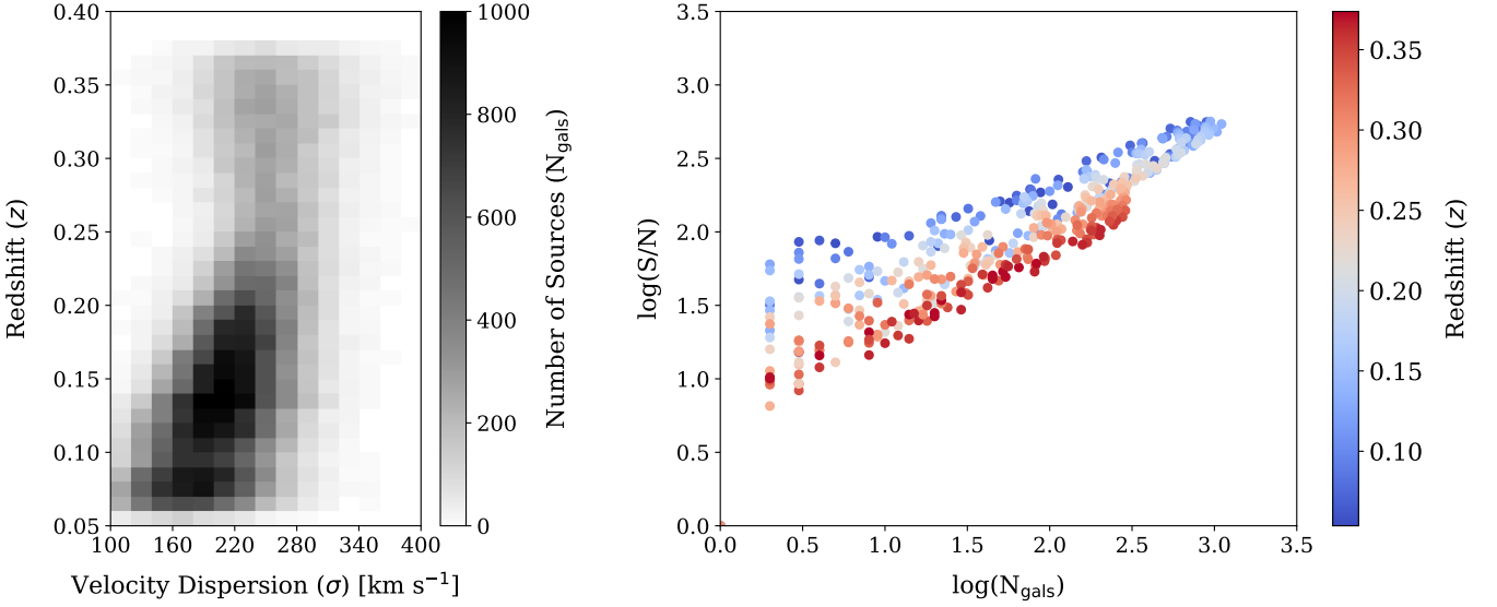
Fig. 3. Properties of the ancillary stacks. Left panel: Distribution of the number of galaxies included in the ancillary stacks defined by a linear constant spacing in both \sigma and z . Right panel: Relation between the S/N and the number of galaxies in each ancillary stack as a function of redshift.
