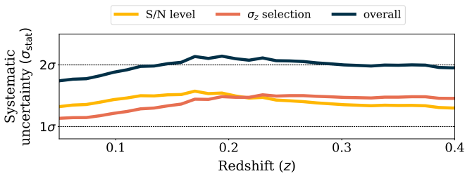
Fig. 10. Systematic uncertainties arising from the methodology directly accounted for in this work. They are presented in units of 1\sigma of the statistical uncertainty \sigma_{\text{stat}} at each redshift. The individual contributions of the level of S/N selected in the stacking procedure and the limit to the dispersion of sources in redshift in each stack are presented in yellow and dark orange, respectively. In dark blue, we present the overall systematic uncertainty.
