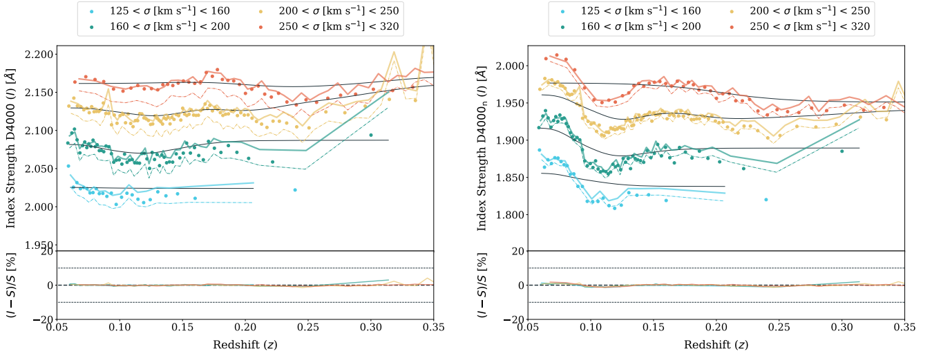
Fig. D.3. Index-redshift relation for the discontinuity features, D4000 (left) and D4000 n (right). The structure of each panel is equivalent to Fig. 13.
