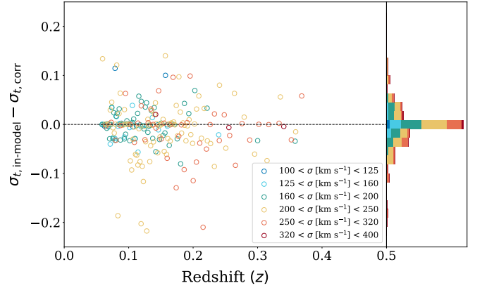
Fig. A.2. Comparison of the uncertainties derived from Knowles-modelled age resulting from the two possible treatments of the velocity dispersion effect.
