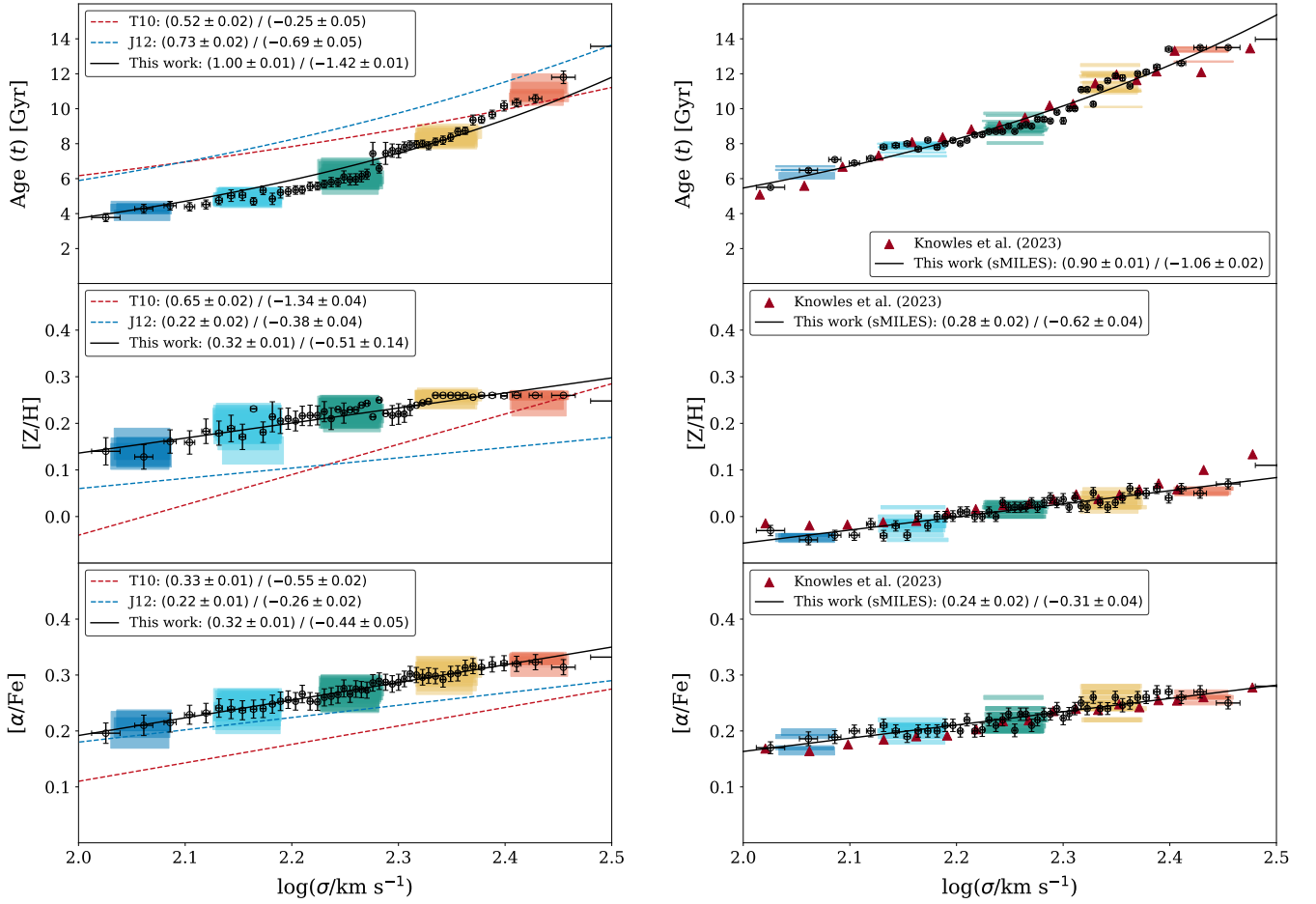
Fig. 11. Left panel: Age, metallicity, and \alpha -enhancement trends with velocity dispersion at low redshift ( 0.05 < z < 0.10 ). The black data points represent the results from stacks of 400 galaxies. The dashed red and blue tendencies represent the Thomas et al. (2010) and Johansson et al. (2012) results (central values). The best log-log fit is plotted as a solid black line. We also depict the results from the ‘default’ stacks as coloured rectangles representing the different velocity dispersion groups from dark blue ( 100 < \sigma [\text{km s}^{-1}] < 125 ) to orange ( 250 < \sigma [\text{km s}^{-1}] < 320 ). Note that the colour code of the velocity dispersion groups corresponds to the one used in Figs. 6 and 8. Right panel: Same as the left panel but with the Knowles model. Red triangles are the results by Knowles et al. (2023) for stacks of massive ETGs, which were previously constructed by La Barbera et al. (2013) using the same model.
