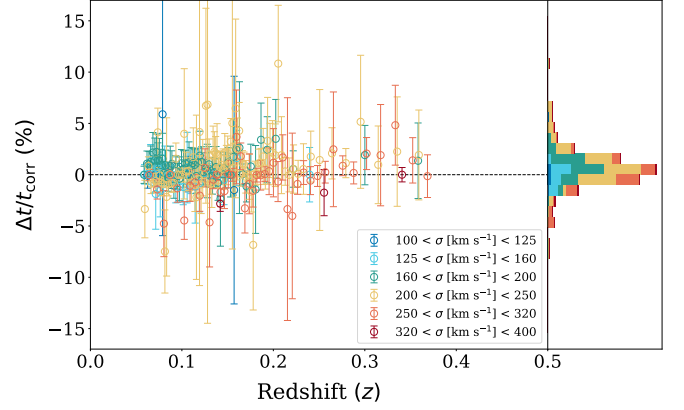
Fig. A.1. Effect on the modelled age (Knowles model) of varying the methodology to account for the velocity dispersion effect. Colours are chosen to represent the velocity dispersion groups in Fig. 8.
