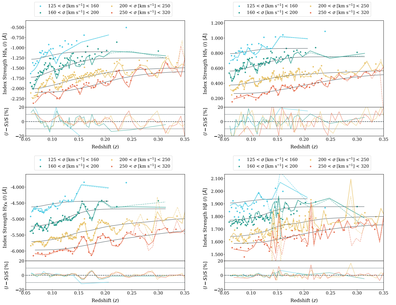
Fig. D.1. Index-redshift relation for Balmer lines. On top H\delta_A (left) and H\delta_F (right). Below H\gamma_A and H\beta . The structure of each panel is equivalent to Fig. 13.
