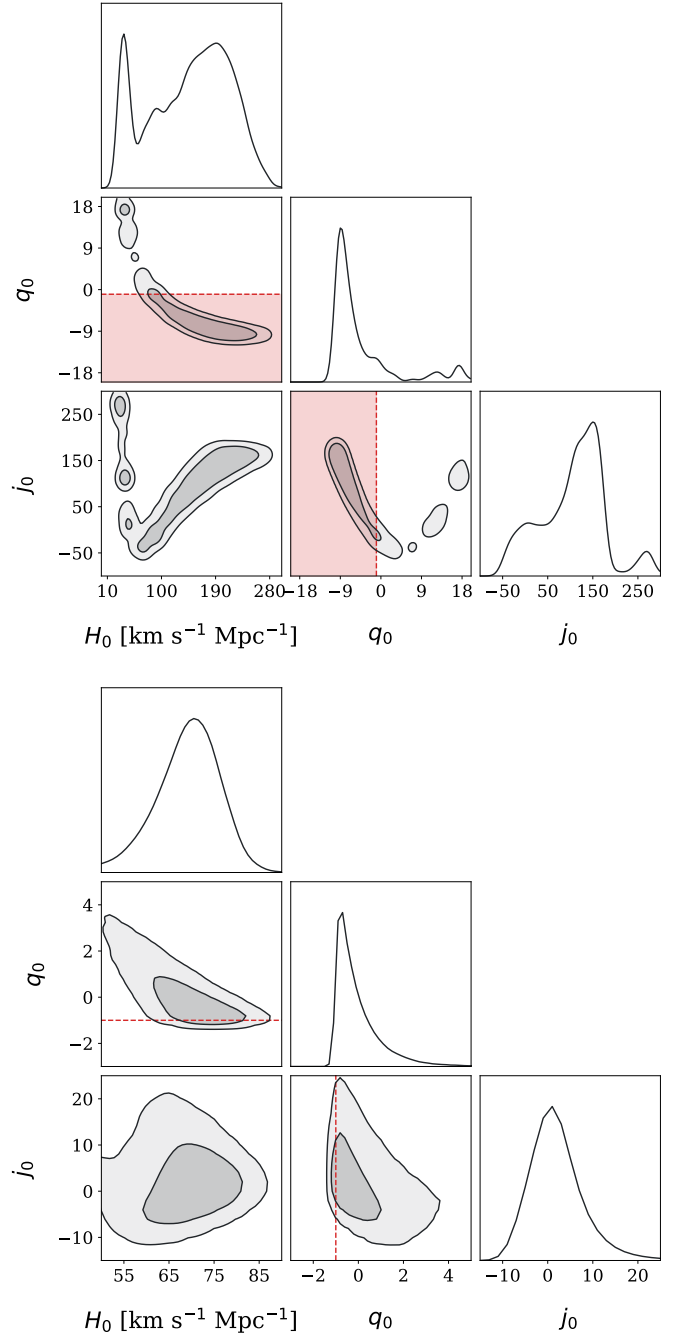
Fig. B.1. Sampling of the parameter space relative to the cosmographic parameters. On top, the general case in which the dH/dz > 0 condition was removed; for clarity, not only is q_0 = -1 shown but also the entire q_0 < -1 region. On the bottom, the baseline case is shown with the exclusion of the data in the range 0.15 < z < 0.20 .
