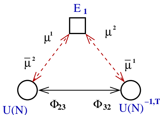
Figure 6: The extended \mathbf{Z}_3 orientifold theory with (0, N) fractional D3-branes and (1, 0) instanton number. The upper node (which would represent the \text{USp}(N_1) gauge group and disappears when we set N_1 = 0 as in the case under consideration) is where the instanton sits. The lower nodes denote only one gauge group. The charged fermionic zero-modes follow eq. (5.11). For simplicity we have not drawn the lines denoting the adjoint.
