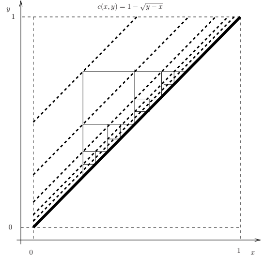
(d) A set of uniqueness with no optimal pair and well posed quotient problem (Ex. 6.4).
