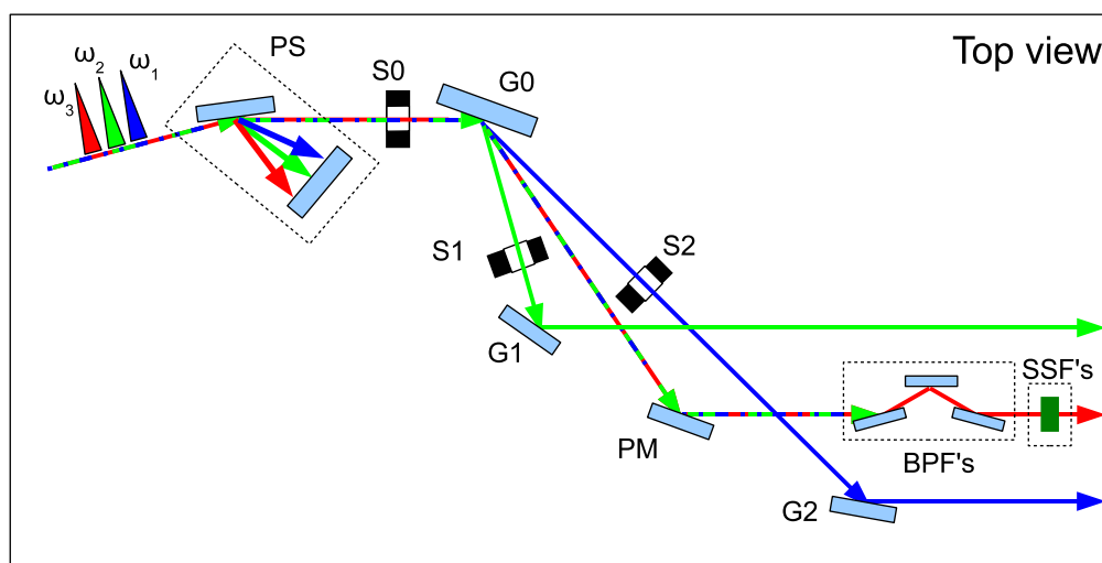
Figure 5. Sketch of the proposed layout to select and spatially separate the three-color FEL pulses (top-view, all reflection angles are enlarged for clarity). PS is the PADReS VUV spectrometer, presently available at FERMI@Elettra, (G 0 ,G 1 ,G 2 ) are diffraction gratings, (S 0 ,S 1 ,S 2 ) are slits, PM is a plane mirror, while BPFs and SSFs are multilayer-based bandpass and solid state filters (SSF), respectively.
