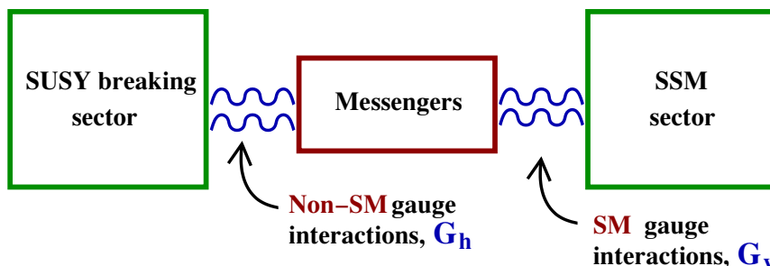
Figure 1. A cartoon of semi-direct gauge mediation. The gauge group G_h is singled-out within the hidden sector as the subgroup to which the messenger fields couple. G_v is the gauge group of the visible sector.
