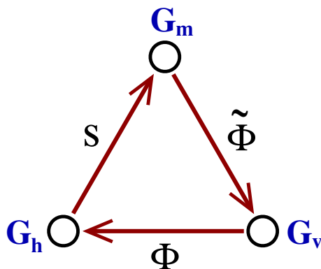
Figure 3. The quiver gauge theory arising at a dP_3 Calabi-Yau singularity describing the messenger sector and its interactions. Visible matter fields are attached to the group G_v , and can be engineered in terms of flavor D7-branes at the singularity. The SUSY breaking dynamics couples instead only to G_h .
