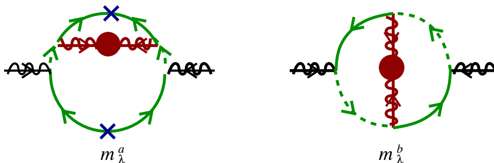
Figure 2. The diagrams contributing to the gaugino mass. The external line corresponds to the visible gaugino \lambda , the internal line with the blob attached corresponds to the propagator of the hidden gaugino (the blob encodes the exact hidden sector non-supersymmetric correction to the propagator), while all other internal lines correspond to messenger fields. The left diagram has two (supersymmetric) mass insertions, each one represented by a cross on the corresponding messenger fermionic line.
