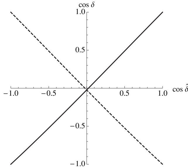
Figure 2: Dependence of \cos \delta on \cos \hat{\delta} in the case of G_f = S_4 or A_5 with \sin^2 \theta_{12}^\circ = 1/4 . The mixing parameters \sin^2 \theta_{23} and \sin^2 \theta_{13} have been fixed to their best fit values for the NO neutrino mass spectrum quoted in eqs. (7) and (8). The solid (dashed) line is for the case when \sin 2\hat{\theta}_{23}^e \sin 2\hat{\theta}_{13}^\nu is positive (negative).
