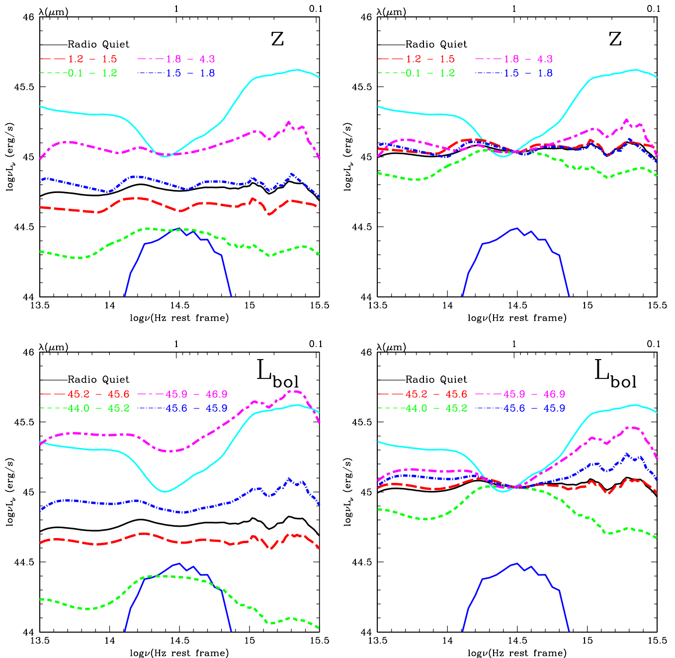
Figure 4. The mean SED for XCRQ407 in bins of z , L_{\text{bol}} before (left) and after (right) normalization at 1 \mu\text{m} compared to the E94 mean radio-quiet SED (cyan solid line). The black lines show the mean SED for all the radio-quiet type 1 AGN in the XMM-COSMOS sample (XCRQ407). A host galaxy template [an elliptical (5 Gyr), E5, blue solid line] is normalized to L_* from the UKIDSS Ultra Deep Survey (Cirasuolo et al. 2007).
