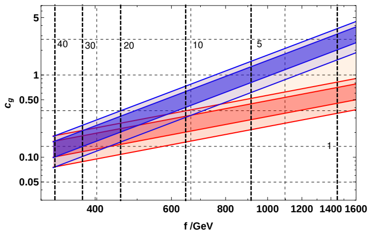
Figure 2. 1, 2\sigma contours on the parameters of the axion model fit to the ATLAS excess for the cases where Red : the invisible decay width is set to zero, and Blue : the total decay width is set to 40 GeV (due to invisible decay channels). Black vertical lines indicate the partial decay width into two axions in GeV.
