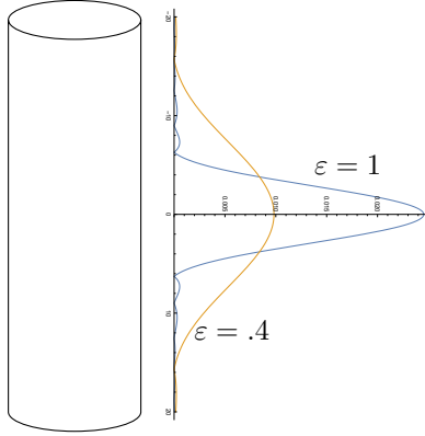
FIGURE 3. Measures on \square for c = 1 in the Heisenberg group \mathbb{H}_3 for the original construction. Each zero corresponds to a conjugate point.
