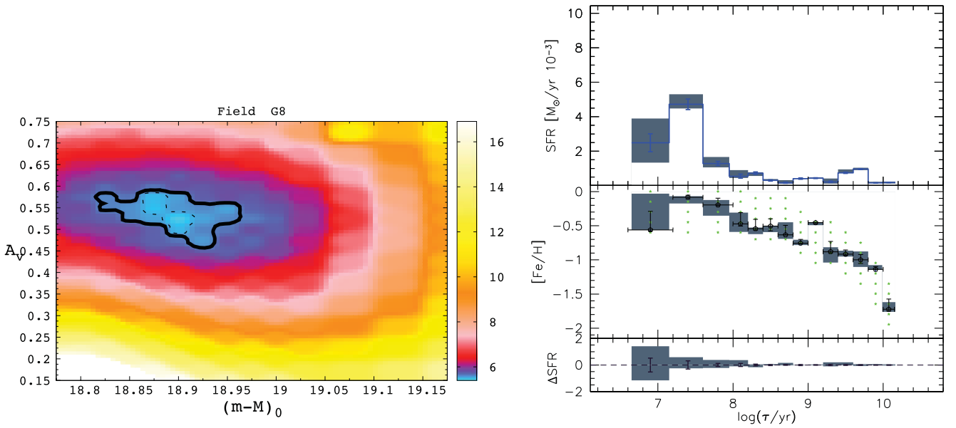
Figure 4. The SFH results for subregion G8 of tile SMC 5_4, which corresponds to a relatively dense region of the SMC bar. The left-hand panel shows the map of \chi_{\min}^2 derived from STARFISH over a wide range of distance moduli and extinctions. The continuous line delimits the 3\sigma (99.7 per cent) confidence level area of the best-fitting solution, while the dashed line delimits the 1\sigma (68 per cent) confidence level. The right-hand panels shows the best fitting solution in the form of the SFR in units of M_{\odot} \text{yr}^{-1} as a function of the logarithm of age (blue histogram, top panel), for all age bins represented in the partial models, together with the averaged metallicity (black dots, middle panel). In the middle panel, the small green dots mark the central [\text{Fe}/\text{H}] and \log(t/\text{yr}) values for which partial models are defined. In both panels, the vertical error bars mark the random errors in the \text{SFR}(t) and [\text{Fe}/\text{H}](t) relations, while the grey-shaded areas delimit the systematic errors.
