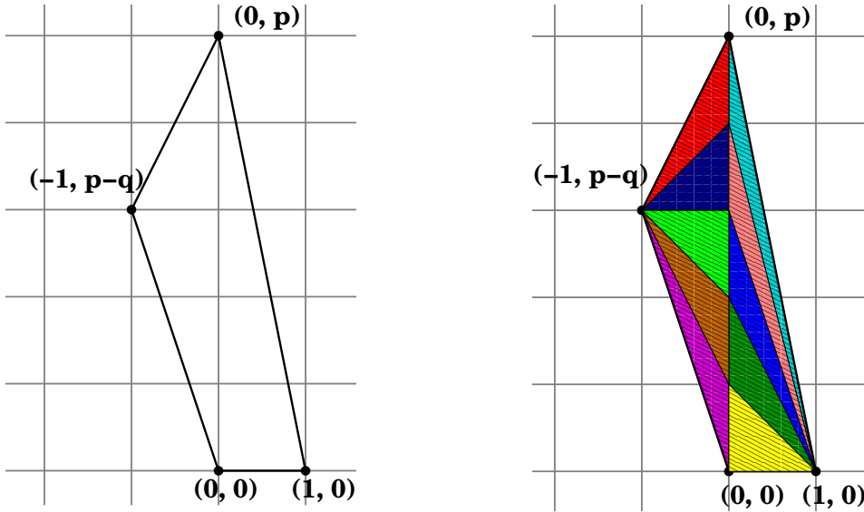
Figure 3.1: The toric diagram of C(Y^{p,q}) for p = 5, q = 2 . Figure 3.2: The toric diagram of C(\widetilde{Y^{p,q}}) for p = 5, q = 2 .
