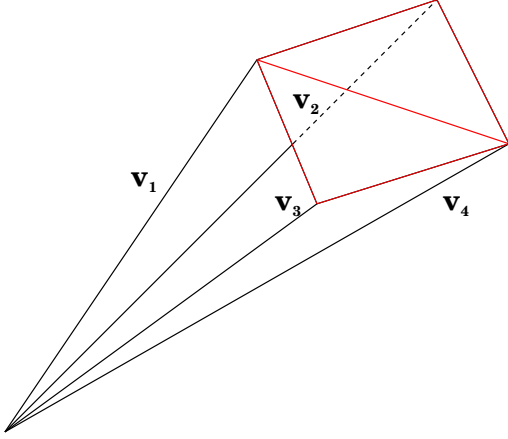
Figure 2.1: The fan of the resolved conifold, \mathcal{O}_{\mathbb{P}}(-1) \oplus \mathcal{O}_{\mathbb{P}}(-1) .
