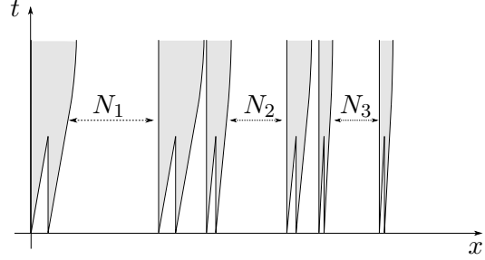
FIGURE 3.7. Solution with \text{TV}(f' \circ u) = +\infty .
