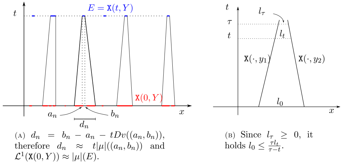
FIGURE 4.7. SBV regularity of f' \circ u
