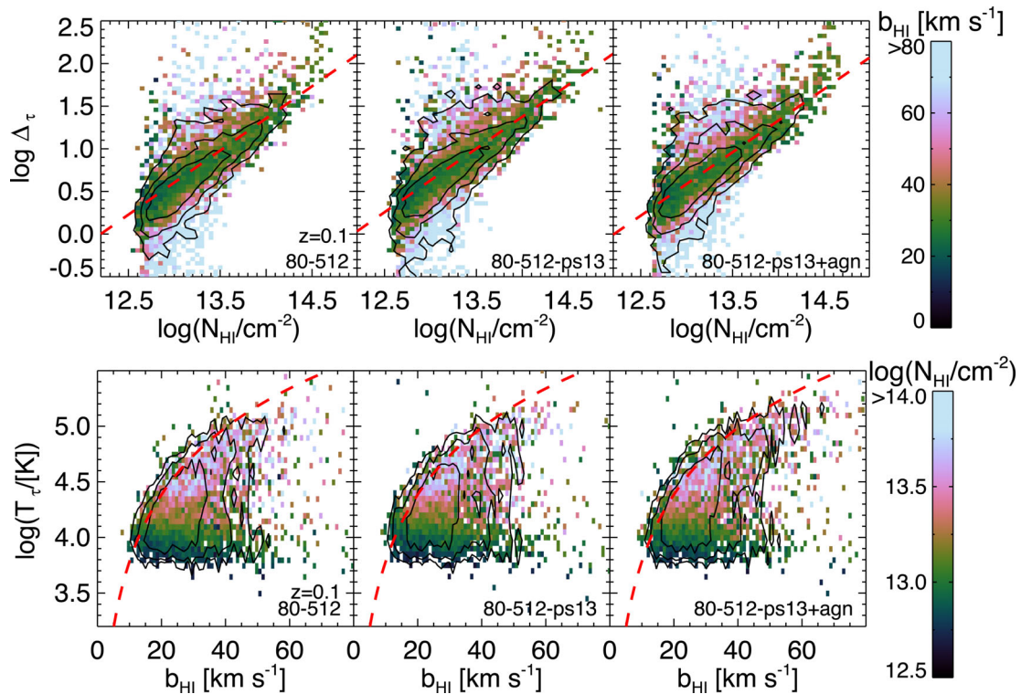
Figure 8. Upper panel: The optical depth weighted normalized gas density against the H I column density for simulations with different prescriptions for feedback at z=0.1 (from left to right, QUICKLYA, stellar feedback and stellar+agn feedback). The colours display the median velocity widths of the absorbers in each cell, and the black contours enclose 50, 75 and 90 per cent of total number of absorbers. Only data points with relative errors on the velocity widths and H I column densities less than 50 per cent are shown. The red dashed line shows the analytical model of Schaye (2001), evaluated at the gas temperature and H I photoionization rate used in the simulation (see equation 1). Lower panel: The optical depth weighted gas temperature against the Ly \alpha velocity widths, b_{\text{HI}} . The colours now correspond to the median H I column density in each cell and the red dashed line shows the relationship between T and b_{\text{HI}} for pure thermal broadening, given by equation (2).
