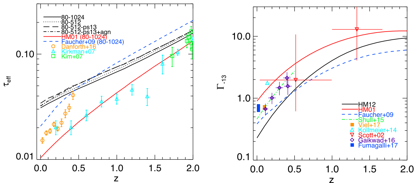
Figure 2. Left: The redshift evolution of the effective optical depth, \tau_{\text{eff}} , predicted by the hydrodynamical simulations. The evolution using the HM01 (red triple-dot dashed line) and Faucher-Giguère et al. (2009) (blue dashed line) UVB models for emission from star-forming galaxies and quasars are also shown for the rescaled 80-1024 model. The Ly \alpha forest observations are from Kirkman et al. (2007), Kim et al. (2013) and Danforth et al. (2016). Right: The H I photoionization rate, \Gamma_{-13} = \Gamma_{\text{H I}}/10^{-13}\text{s}^{-1} , evolution with redshift for the HM12 (black solid line), HM01 (red triple-dot dashed line) and Faucher-Giguère et al. (2009) (blue dashed line) UVB models. The observational measurements are from Scott et al. (2002), Kollmeier et al. (2014), Gaikwad et al. (2017a), Viel et al. (2017) and Fumagalli et al. (2017). The green dot-dashed line is the best fit from Shull et al. (2015).
