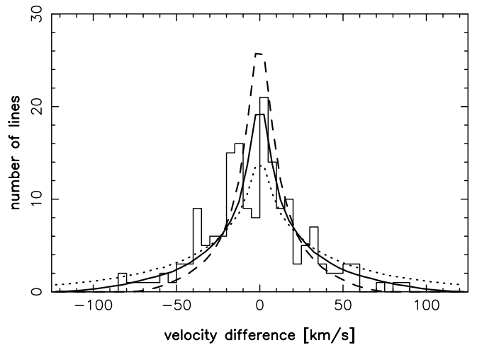
FIG. 12.—Velocity shear between the lines of sight for Ly \alpha forest lines in the spectra of Q1439–0034AB and the pair Q1422+2309A/Q1424+2255. The histogram gives the combined observed distributions of the two pairs. The solid line is the best-fit expanding pancake model with v = 0.65v_{\text{Hubble}} . For comparison, the dashed and dotted lines show the distribution for v = 0.4v_{\text{Hubble}} and 1.2v_{\text{Hubble}} , respectively.
