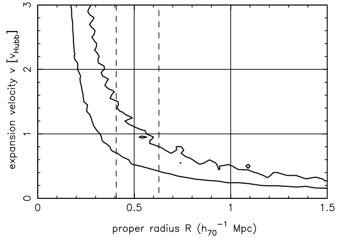
FIG. 16.—Solid lines are the \chi^2 contours ( \pm 3 \sigma ) for the maximum likelihood fit of the expanding pancake model to the velocity shear distribution at z \approx 2 (see Fig. 11), with the expansion velocity in units of the Hubble velocity and the proper radius of the pancakes as free parameters. The vertical dashed lines give the \pm 3 \sigma limits for the radii of the absorbing structures from D’Odorico et al. (1998). According to this plot, the average expansion of the Ly \alpha forest at mean redshift ( z = 2.04548 ) is v = (0.8 \pm 0.3)v_{\text{Hubble}} ( \sim 3 \sigma ).
