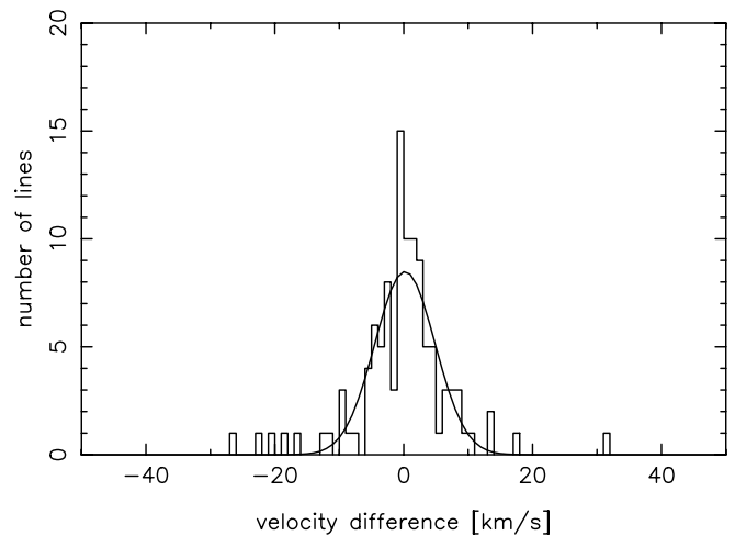
FIG. 5.—Observed histogram of the velocity differences \Delta v (= v_B - v_A) for pairs of absorption components toward RX J0911.04+0551AB. The solid curve is the expected Gaussian distribution, if the width were entirely caused by the mean measurement error \sigma(v_B - v_A) = 4.7 \text{ km s}^{-1} and there were no intrinsic differences between the lines of sight. There are a few outliers with 3\sigma significant velocity differences that are shown individually in Fig. 6.
