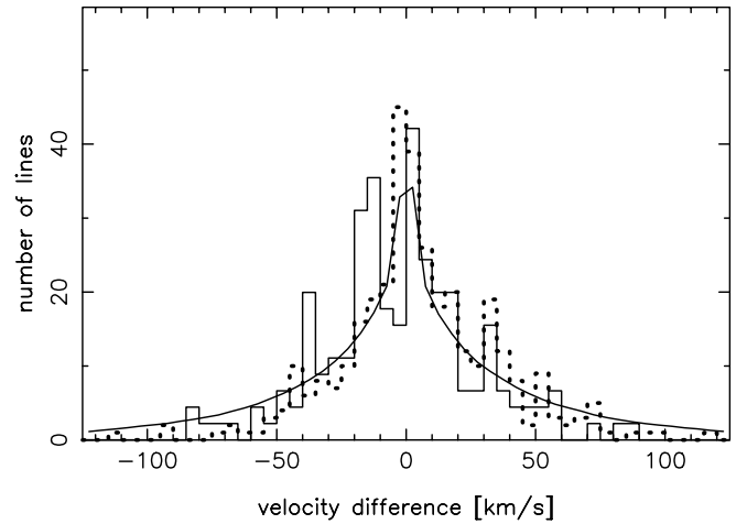
FIG. 20.—Same as Fig. 19, but with the solid histogram now showing the \Delta v measurements for the higher redshift ( z \approx 3.6 ) combined sample from the Q1439–0034AB pair and the Q1422+2309A/Q1422+2255 pair. Again the dotted line is from the simulation for mean redshift \langle z \rangle = 3.6 , and the solid curve is the expanding pancake model for the same redshift with a Hubble ratio r = 1.0 .
