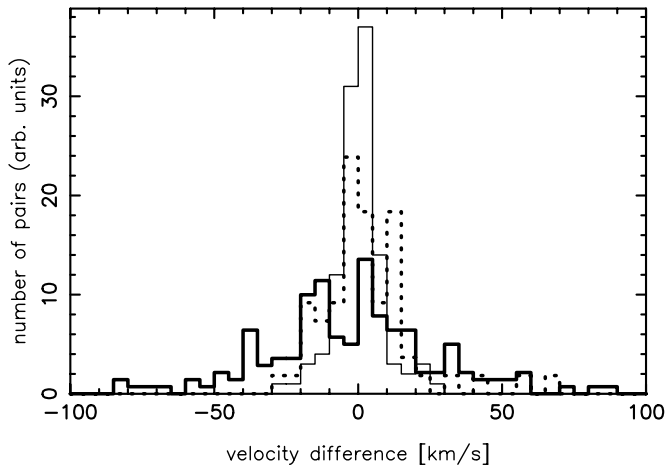
FIG. 13.—Observed distributions of velocity shear with the histograms from Figs. 5, 11, and 12 normalized to the same integral (arbitrary units) and overplotted on top of each other. The RX J0911.4+055 sample is represented by the thin-lined histogram, the Q2345+007AB sample by the dotted one, and the high-redshift combined Q1422+2309A/Q1424+2255 and Q1439–0034AB samples by a thick solid histogram.
