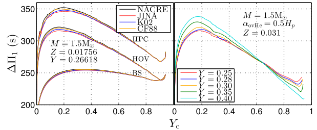
Figure 4. Left-hand panel: RC- \Delta\Pi_1 evolution as a function of central helium mass of an M = 1.50 M_{\odot} solar metallicity star with three different mixing schemes and four different ^{12}\text{C}(\alpha, \gamma)^{16}\text{O} reaction rates. Right-hand panel: RC- \Delta\Pi_1 evolution as a function of central helium mass fraction of an M = 1.50 M_{\odot} star computed assuming three different combinations of Z and Y .
