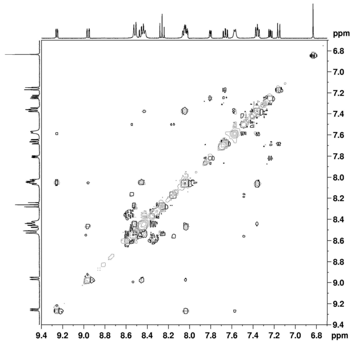
Supporting information Figure 2. Aromatic region of the ^1\text{H} - ^1\text{H} NOESY spectrum of 1d in \text{MeOH-}d_4 at 328 K
