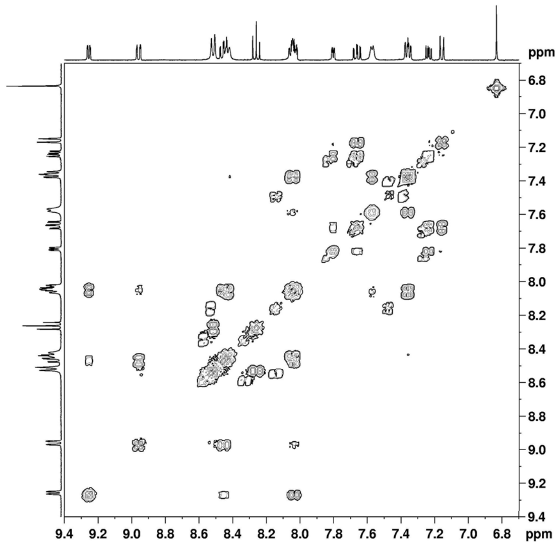
Supporting information Figure 1. Aromatic region of the ^1\text{H} - ^1\text{H} COSY spectrum of 1d in \text{MeOH-}d_4 at 328 K
