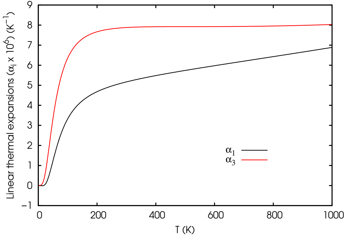
Figure 9. Calculated LDA linear thermal tensor ( \alpha_1 = \alpha_2 and \alpha_3 ) for Re h.c.p. These results were obtained using the full grid (a, c/a) , minimizing the Helmholtz energy to obtain a(T) and c/a(T) and eqs. 12, 13.
