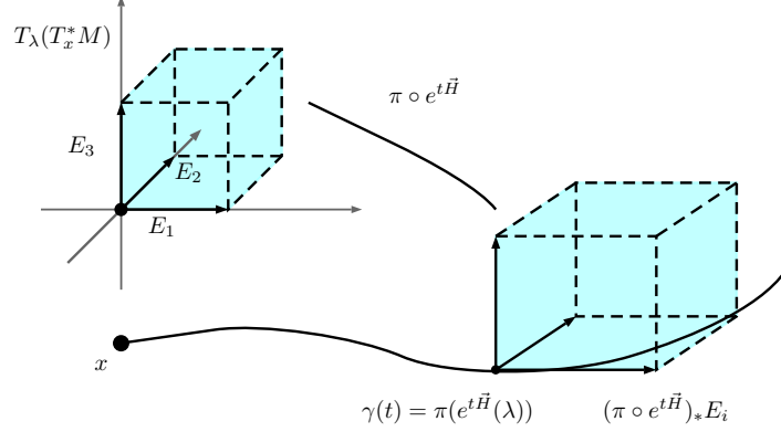
FIGURE 2. Volume distortion under the Hamiltonian flow
