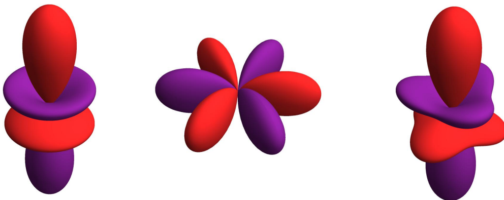
Figure 2.1: Plots of the absolute values on the sphere S^2 of a zonal harmonic Z_{3,3} (left), a function \hat{M}_{3,2} with 6 critical points on the circle (middle) and a perturbation of Z_{3,3} by \hat{M}_{3,2} with 14 = 2 + 2 \cdot 6 non-degenerate critical points (right).
