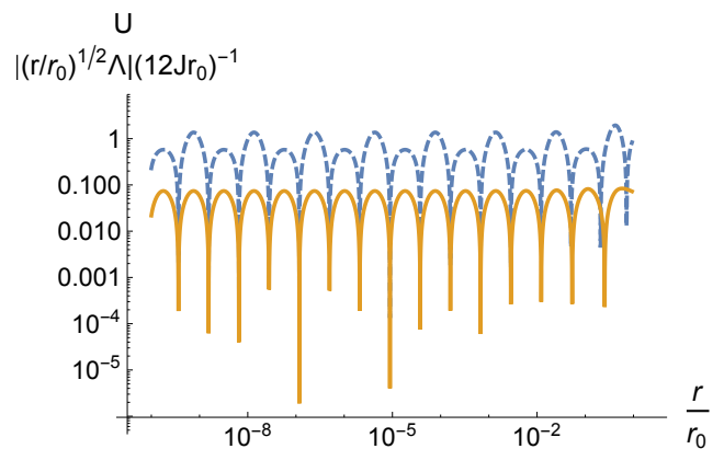
FIG. 4. (Color online). Numerical solutions for U (dashed blue) and r^{1/2}\Lambda (solid orange) in the small-coupling limit, and for s_0^2 \approx 1.87 and s_1^2 \approx 1.95 .
