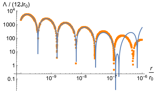
FIG. 3. (Color online) Same as in Fig. 2, but for \Lambda(r) .
