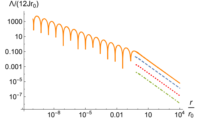
FIG. 1. (Color online) Plots of \Lambda/(12J) for different spin-1 mode speeds (solid orange: s_1^2 = 2 ; dashed blue: s_1^2 = 10 , dotted red: s_1^2 = 100 ; dash-dotted green: s_1^2 = 1000 ) and fixed spin-0 mode speed s_0^2 = 3/2 . The solution for s_1^2 = 2 can be extended down to arbitrarily short distances from the central singularity at r = 0 , because no multiple spin-1 horizons are present. The other solutions, however, present multiple spin-1 horizons, all of which are singular with the exception of the outermost one. Hence, we only plot those solutions outside the outermost spin-1 horizon.
