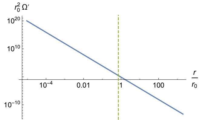
FIG. 6. (Color online) Plot (log-log scale) of our numerical solution for \Omega'(r) for c_\theta = c_a \approx -0.00305 , c_\sigma = 0.01 , c_\omega = 0.0018 . The green vertical line marks the universal horizon of the static spherically symmetric seed solution. Note that unlike in Fig. 5, we have not shown the corresponding small coupling limit solution because it would be indistinguishable by eye.
