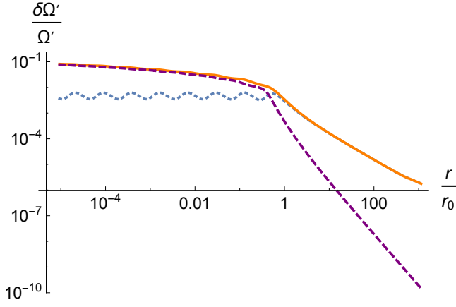
FIG. 7. (Color online) Fractional differences (in log-log scale) between the frame-dragging, \Omega' , in \text{ae} -theory/Hořava gravity (for c_\theta = c_a \approx -0.00305 , c_\sigma = 0.01 , c_\omega = 0.0018 ) and GR. In dotted blue is the difference between \text{ae} -theory and Hořava gravity; in solid orange is the difference between \text{ae} -theory and GR; and in dashed purple the difference between Hořava gravity and GR.
