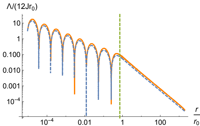
FIG. 5. (Color online) Solutions for \Lambda(r) for finite values of the coupling constants ( c_\theta = c_a \approx -0.00305 , c_\sigma = 0.01 , c_\omega = 0.0018 ; dashed blue), together with the corresponding small coupling limit solution (solid orange; with s_0^2 \approx 1.87 and s_1^2 \approx 1.95 ). The green vertical line marks the universal horizon of the static spherically symmetric seed solution.
