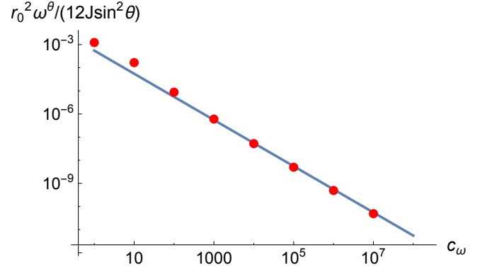
FIG. 9. (Color online) Behavior of \omega^\theta / \sin^2 \theta evaluated at r = 4\mu as a function of c_\omega (for fixed c_a = 1/2 and c_\sigma = 3/4 ) from our numerical solutions (red dots) vs a simple 1/c_\omega scaling (solid blue line).
