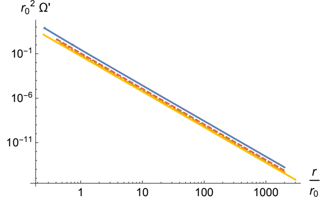
FIG. 10. (Color online) Derivative of frame dragging, \Omega'(r) , for various values of c_\omega following the same color scheme of Fig. 8. The additional yellow curve below all other curves is the GR result, which also coincides with the Hořava gravity result for c_a + 2c_\sigma = 0 . We see again that as c_\omega \rightarrow \infty , the frame dragging in \mathfrak{a} -theory solutions approaches that of Hořava gravity.
