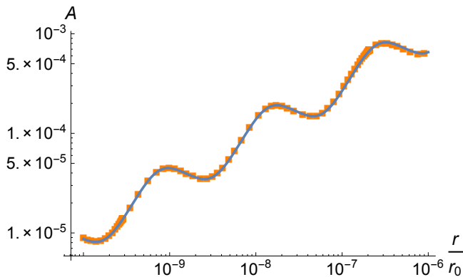
FIG. 2. (Color online) Comparing the numerical solution for A(r) (in the small-coupling limit and for s_0^2 \approx 1.87 and s_1^2 \approx 1.95 ; orange dots) to a perturbative approximate solution valid at sufficiently small radii (solid blue curve).
