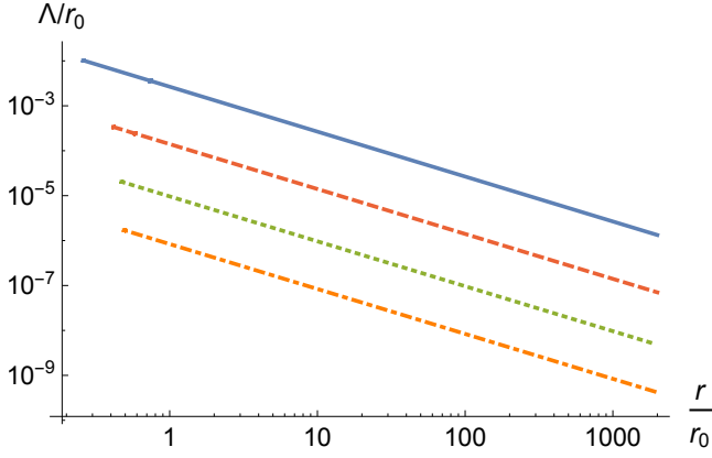
FIG. 8. (Color online) \Lambda(r) for selected values of c_\omega (and fixed c_a = 1/2 and c_\sigma = 3/4 ). The solid blue is for c_\omega = 10 , the dashed red one for c_\omega = 100 , the dotted green one for c_\omega = 1000 , and the dot-dashed orange one for c_\omega = 10^4 . Note that for each of these cases, a second spin-1 horizon resides within the universal horizon of the spherically symmetric static seed solution. This horizon is singular (i.e. it is the location of a finite-area curvature singularity), and therefore the curves displayed here are terminated right before reaching it. Still, outside this finite-area singularity, \Lambda(r) approaches zero at all radii as c_\omega \rightarrow \infty .
