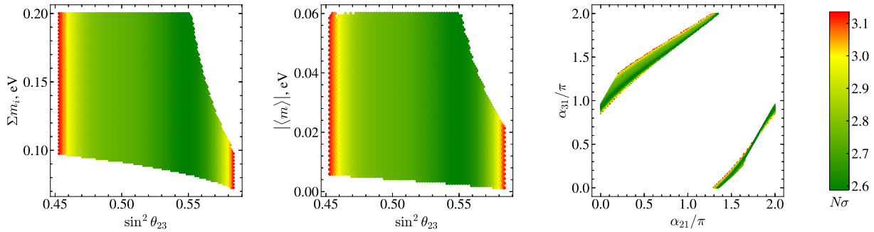
Fig. 1. Correlations between \sin^2 \theta_{23} and the sum of neutrino masses \sum m_i , between \sin^2 \theta_{23} and the effective Majorana mass |\langle m \rangle| , and between the Majorana phases \alpha_{31} and \alpha_{21} in the case of NO neutrino mass spectrum. See text for further details.
