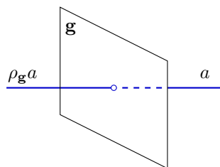
Figure 2. When a symmetry operator of type a \in \mathcal{A} crosses a codimension-1 symmetry operator of type \mathbf{g} \in G , it emerges transformed by an automorphism \rho_{\mathbf{g}} of \mathcal{A} .
