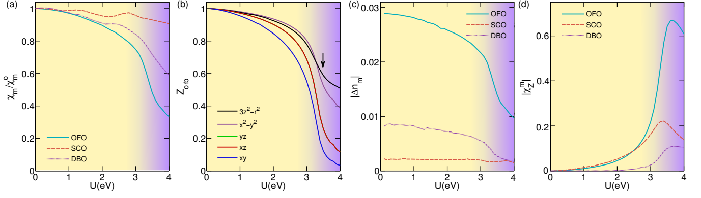
FIG. 1: (Color online) (a) Orbital nematic susceptibilities \chi_m(U) normalized to their respective U = 0 value, for J_H/U = 0.20 and electronic filling n = 6 [27]. The OFO is strongly suppressed by interactions while the SCO is only weakly affected. (b) Orbital-dependent quasiparticle weight Z_{\gamma} as a function of U in the absence of a nematic perturbation. The sharp drop around U \sim 3.2 eV signals the entrance into the strongly correlated Hund's metal region where the atoms become spin polarized. The shading colors in the panels differentiate the weakly correlated and the Hund's metal regime. The arrow signals the interaction value U = 3.5 eV at which the orbital-dependent mass enhancements equal those observed in ARPES and Quantum Oscillations experiments in FeSe [28–30]. (c) Occupation imbalance between xz and yz orbitals for the three orders taking 2h_m = 75\text{meV} . The larger is the imbalance produced by an order, the stronger is the \chi_m(U) suppression of this order by interactions. (d) Absolute value of the Z-response functions \chi_Z^m(U) .
