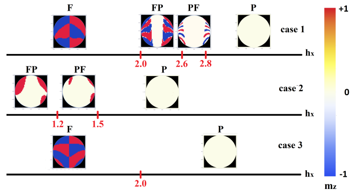
FIG. 5. Same as Fig. 4 including the Liouvillian. Note that apparently disconnected regions with the same colour are actually connected along the y -direction.
