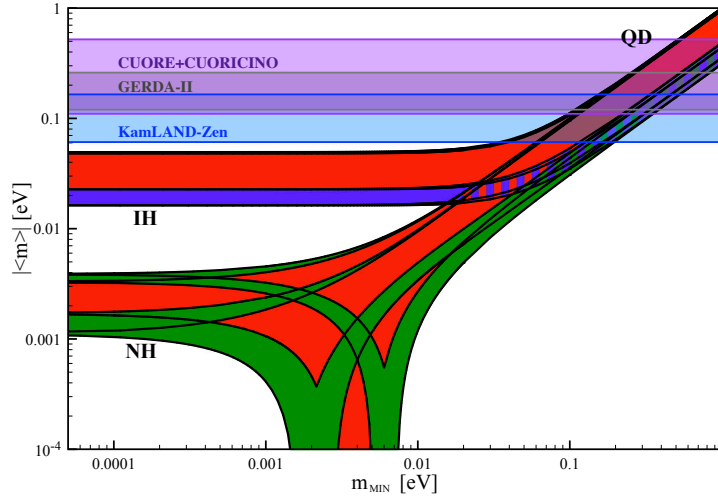
Figure 5 – The effective Majorana mass |\langle m \rangle| (including a 2\sigma uncertainty), as a function of \min(m_j) . The figure is obtained using the best fit values and the 1\sigma ranges of allowed values of \Delta m_{21}^2 , \sin^2 \theta_{12} , \sin^2 \theta_{13} and |\Delta m_{31(32)}^2| from 105 (propagated to |\langle m \rangle| and then taking a 2\sigma uncertainty). The phases \alpha_{21} and (\alpha_{31} - 2\delta) are varied in the interval [0, 2\pi] . The predictions for the NH, IH and QD spectra as well as the GERDA-II 107 , KamLAND-Zen 106 and the combined CUORE+CUORICINO 108 limits (Eqs. (23), (25) and (24)), are indicated. The black lines determine the ranges of values of |\langle m \rangle| for the different pairs of CP conserving values of \alpha_{21} and (\alpha_{31} - 2\delta) : (0, 0) , (0, \pi) , (\pi, 0) and (\pi, \pi) . The red regions correspond to at least one of the phases \alpha_{21} and (\alpha_{31} - 2\delta) having a CP violating value, while the blue and green areas correspond to \alpha_{21} and (\alpha_{31} - 2\delta) possessing CP conserving values (Update by S. Pascoli in 3 of a figure from 109 .)
