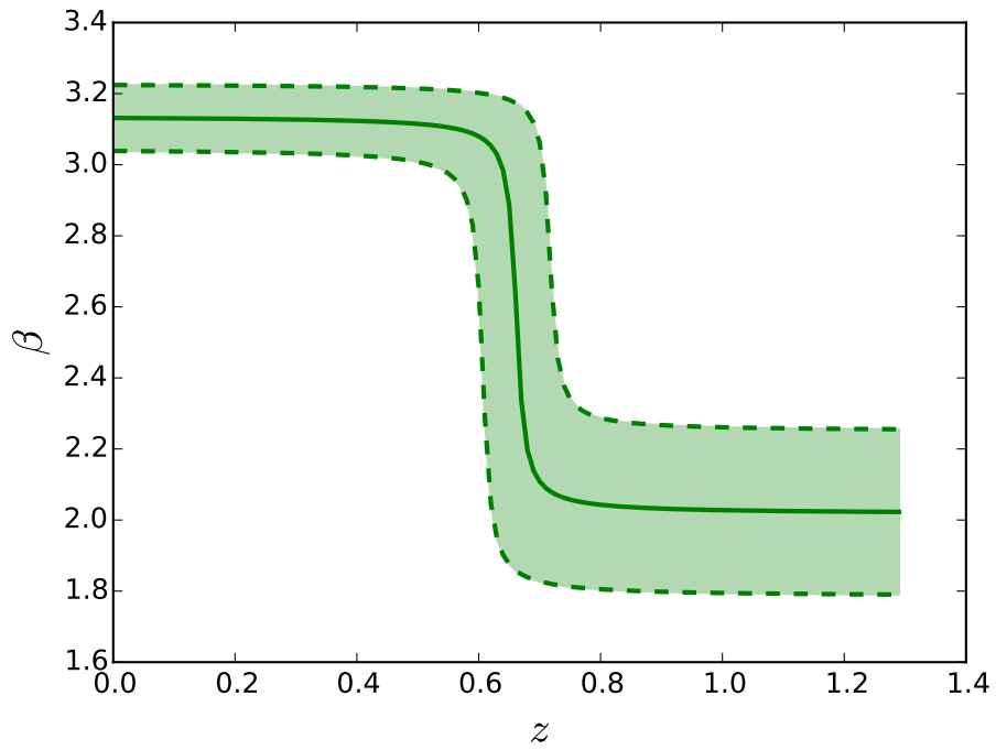
Fig. 12.— Redshift evolution of the color correction parameter \beta , assuming the z -Jump color Correction model. The green line is the posterior mean, while the shaded region represents the 1\sigma credible region. ( \Lambda CDM case).
