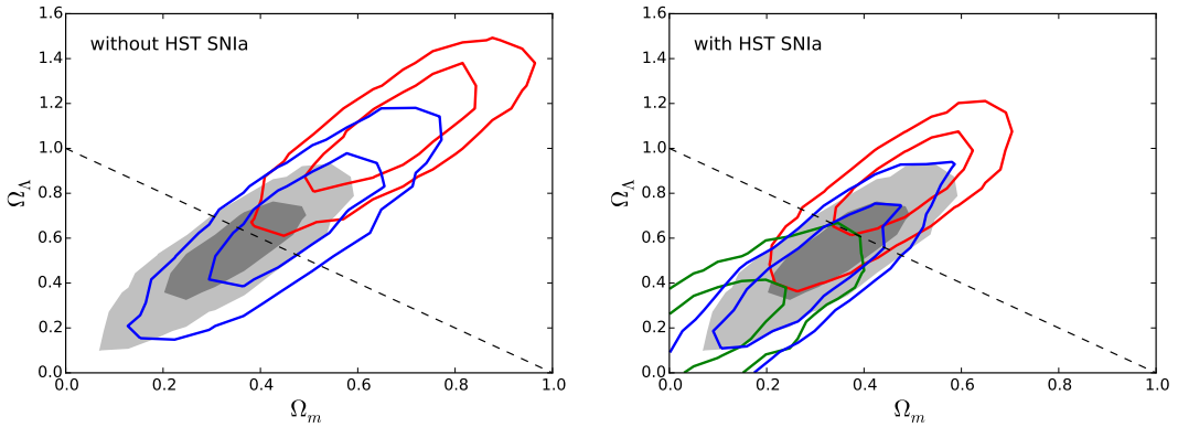
Fig. 16.— Comparison of posterior distributions for the cosmological parameters in the \Lambda CDM case when using different sub-samples of the JLA data, as compared with the result for the entire JLA data set (black/filled). Blue: SDSS+SNLS (613 SNIa, 0.04 < z < 1.06 ), Red: low- z +SNLS (357 SNIa, 0.01 < z < 0.08 \cup 0.13 < z < 1.06 ) and Green: low- z +SDSS (492 SNIa, 0.01 < z < 0.40 ). The left plot does not include the HST SNIa (9 SNIa, 0.84 < z < 1.30 ) while the right one does.
