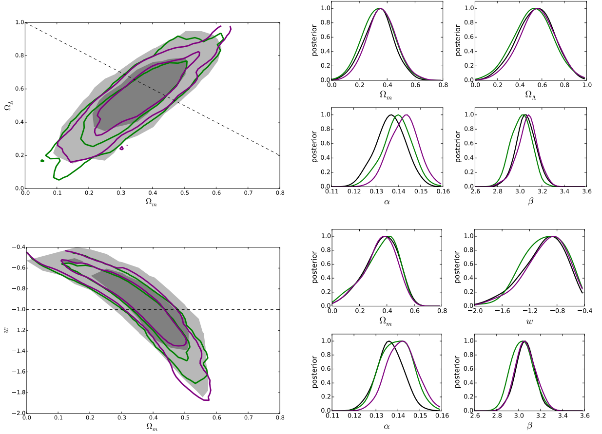
Fig. 5.— Comparison of cosmological parameters and standardization parameters with and without host galaxy mass correction (black/shaded: Baseline Model; green: Soft Classification Model; purple: Covariate Adjustment Model). The result of the Hard Classification Model is similar to that of the Soft Classification Model and is not shown. Top panels are fit under the \Lambda CDM, while the bottom panels are fit under the w CDM. We do not find a significant difference in cosmology when mass information is included in the fit.
