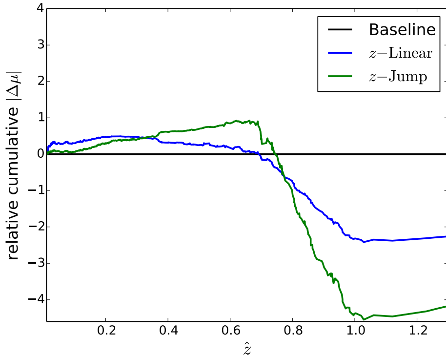
Fig. 14.— Cumulative Hubble residuals relative to the Baseline Model for the two \beta(z) models considered. For z \gtrsim 0.8 , both the redshift-dependent models improve the fit with respect to the Baseline Model, which has \beta = \text{constant} . The z -Jump color Correction model shows the largest improvement in the fit. This plot is for \Lambda\text{CDM} , but the w\text{CDM} case is qualitatively similar.
