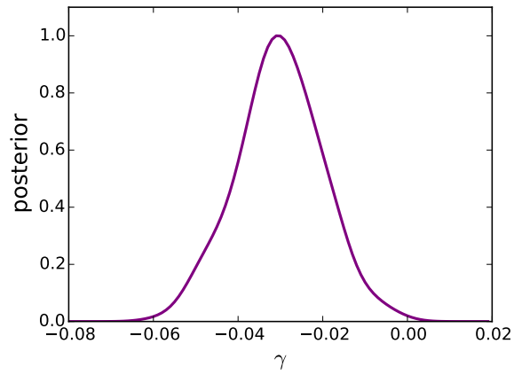
Fig. 9.— Marginal posterior distribution for \gamma , the regression coefficient for M_{g_i} in the Covariate Adjustment Model. (The model is fit assuming a \Lambda CDM universe.) The probability that \gamma is less than zero is 99%.
