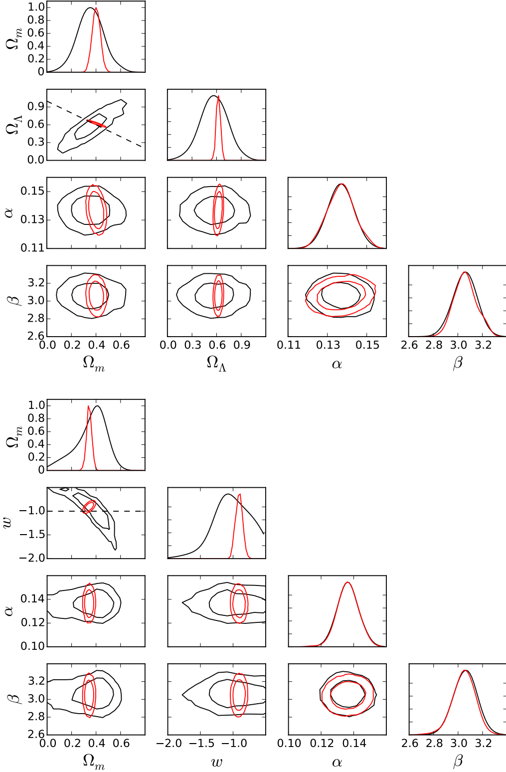
Fig. 2.— 1D and 2D marginal posterior distributions for the cosmological parameters, and the color and stretch correction parameters. Black (red) contours show 68% and 95% highest posterior density regions for JLA SNIa data only (JLA combined with Planck ). The top (bottom) panels display results for the \Lambda CDM ( w CDM) model.
