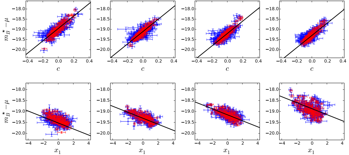
Fig. 4.— Shrinkage of posterior estimates in BAHAMAS : Intrinsic magnitude plug-in estimates (blue) and posterior mean (red). The four panels in the first row correspond to quartiles of \hat{x}_1 ; we plot the regression line as a function of the color parameter in each. The horizontal axis plots \hat{c}_i (blue) and the posterior mean of c_i (red). The four panels in the bottom row correspond to quartiles of \hat{c} ; we plot the regression as a function of the stretch parameter \hat{x}_1 in each. The horizontal axis plots \hat{x}_{1i} (blue) and the posterior mean of x_{1i} (red). The regression lines use the posterior means of the parameters and the mean of the observed covariates in each quartile. The posterior estimates shrink from the plug-in estimates toward the regression line and thus reduce scatter around the regression plane. This is a consequence of the hierarchical regression in the model (this plot is for the \Lambda CDM case).
