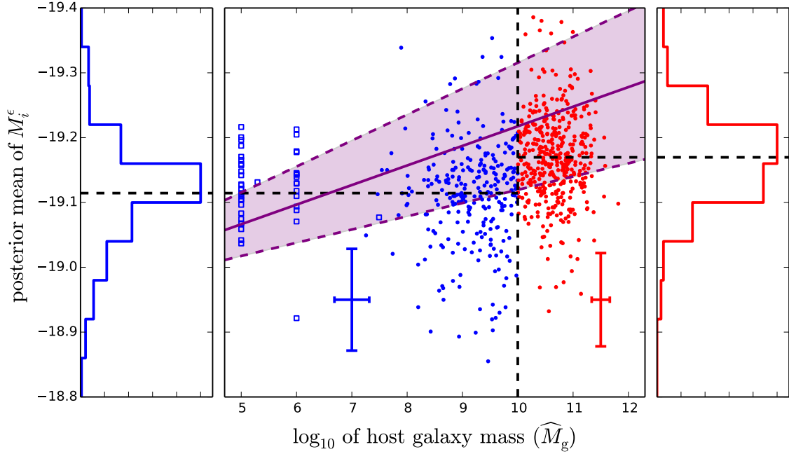
Fig. 7.— Posterior means and standard deviations for the empirically corrected intrinsic magnitudes of SNIa’s in the JLA sample versus measured host galaxy mass. The sample has been divided into two populations, with M_{g_i} smaller (larger) than 10, depicted in blue (red). A hollow square represents SNIa whose nominal measurement error on M_{g_i} is equal to or larger than 5. The population means of the intrinsic magnitudes are M_0^{\text{lo}} = -19.114 \pm 0.023 and M_0^{\text{hi}} = -19.169 \pm 0.022 (horizontal dashed lines) respectively for the low- and high-host mass classes. The blue and red vertical errorbars represent the average posterior standard deviations of the intrinsic magnitudes in the low- and high-host mass classes, respectively. The horizontal errorbars represent the average measurement errors of M_{g_i} in the two classes. The average errorbars exclude the SNIa’s represented by hollow squares. The slope of the purple regression line is the posterior mean of \gamma under the Covariate Adjustment Model, while the purple shaded area represents the 1\sigma credible region for \gamma . (The regression line is computed under \Lambda CDM.)
