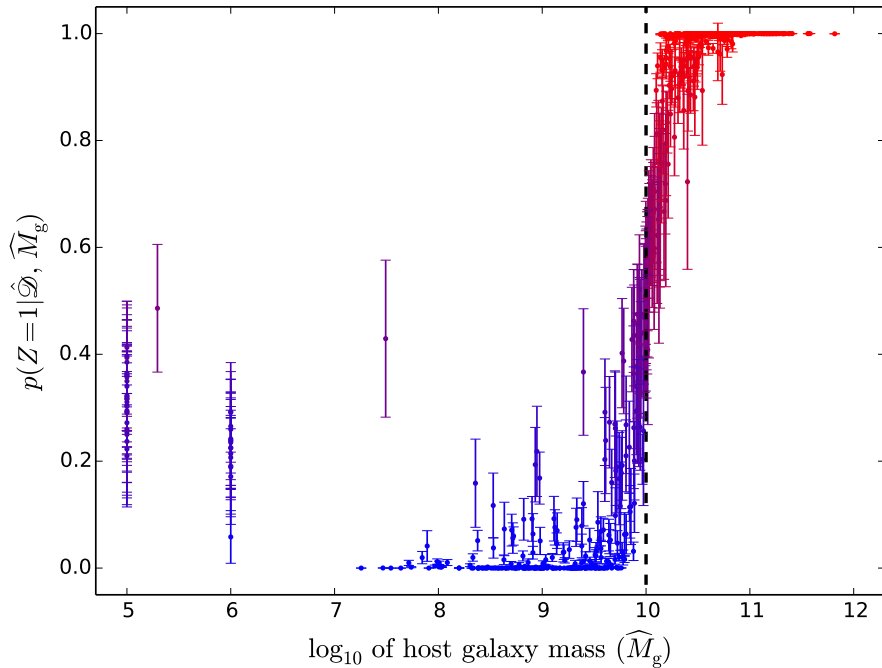
Fig. 8.— Posterior means and standard deviations of the Z_i , the indicator variables for each SNIa belonging to the high-mass host class ( Z_i = 1 , red) versus measured host galaxy mass. If Z_i = 0 (blue), SNIa belongs to the low-mass host class. The posterior mean of Z_i is the posterior probability that SNIa belongs to the high-mass host class. Although the horizontal error bars are suppressed for clarity, the model fully accounts for measurement errors in the host galaxy mass. (This plot assumes the \Lambda CDM.)
