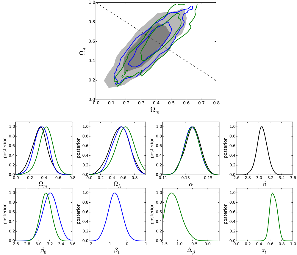
Fig. 10.— Comparisons of the posterior distributions for the cosmological parameters and the standardization parameters under different models for the color correction parameter: Black: Baseline Model (no evolution); blue: z -Linear color Correction model; green: z -Jump color Correction model. Posterior are normalized to the peak. (All models are fit assuming a \Lambda CDM universe).
