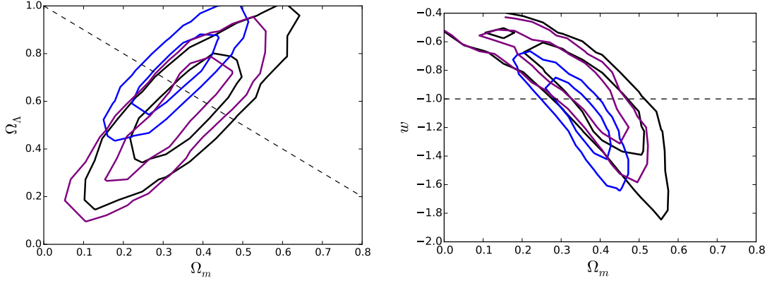
Fig. 15.— Comparison of posterior distributions when including both statistical and systematic errors (black) to the case when the systematics covariance matrix is neglected (blue). Purple: statistics covariance matrix with diagonal errors on m_B^* inflated by the average m_B^* variance from the systematics covariance matrix. Left: \Lambda CDM; Right: w CDM.
