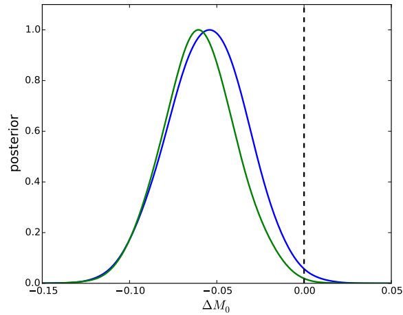
Fig. 6.— Posterior distribution of \Delta M_0 , the difference between mean intrinsic magnitudes of SNIa’s in high-mass host galaxies ( M_{gi} > 10 ) and low-mass hosts ( M_{gi} < 10 ). The blue and green curves correspond to the Hard Classification and Soft Classification models, respectively. Under both models, the posterior probability that \Delta M_0 < 0 is greater than 95%, meaning SNIa’s in more massive hosts are most probably intrinsically brighter ( \Delta M_0 < 0 ). (This plot assumes a \Lambda CDM universe.)
