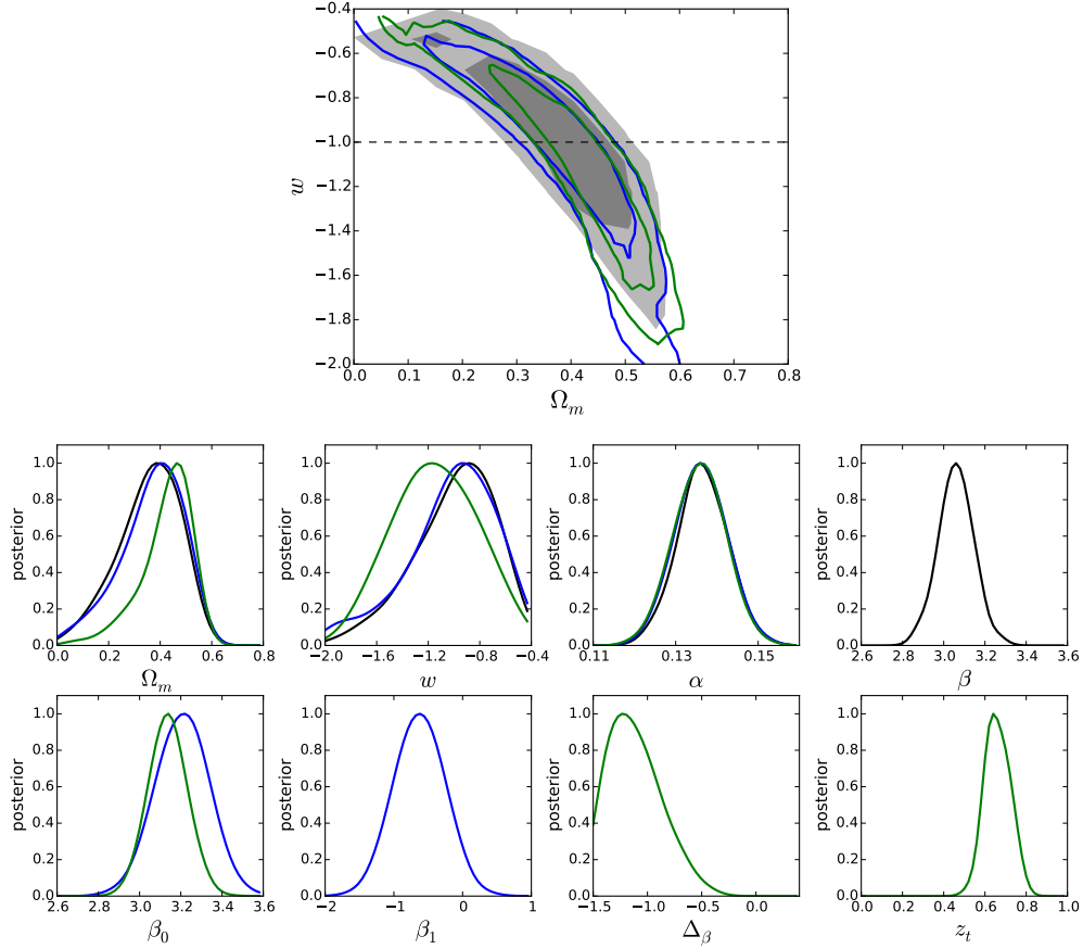
Fig. 11.— Comparisons of the posterior distributions for the cosmological parameters and the standardization parameters under different models for the color correction parameter: Black: Baseline Model (no evolution); blue: z -Linear color Correction model; green: z -Jump color Correction model. Posterior are normalized to the peak. (All models are fit assuming a w CDM universe.)
