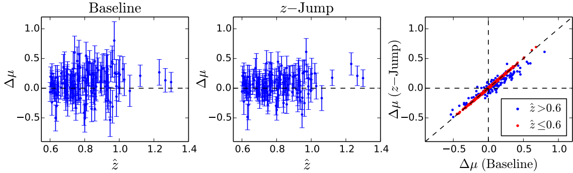
Fig. 13.— Hubble residuals of the Baseline Model (left, \beta = \text{constant} with redshift), z -Jump color Correction model (centre) and comparison between the two (right). In the left and central panels, only SNIa’s with \hat{z} > 0.6 are plotted to highlight the difference between the two cases. Errorbars are the posterior standard deviations of \Delta\mu_i . In the right panel, SNIa’s with \hat{z} \leq 0.6 are plotted in red. This panel shows that the z -Jump color Correction model reduces the scatter around the Hubble diagram noticeably for \hat{z} > 0.6 , while its Hubble residuals are similar to the Baseline Model for \hat{z} \leq 0.6 (this plot is for \Lambda CDM, and the w CDM case is similar).
