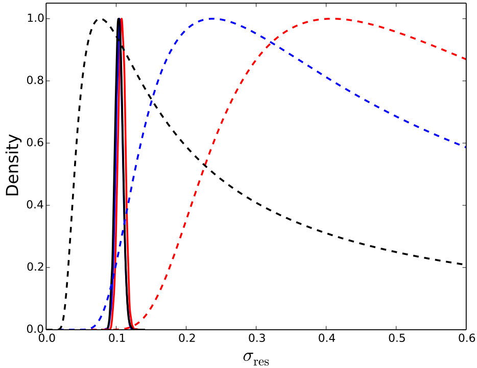
Fig. 3.— Robustness of the posterior distribution for \sigma_{\text{res}} (solid lines) with respect to three different prior specifications (dashed lines) Black: \sigma_{\text{res}}^2 \sim \text{INVGAMMA}(0.003, 0.003) ; blue: \sigma_{\text{res}}^2 \sim \text{INVGAMMA}(0.03, 0.03) ; red: \sigma_{\text{res}}^2 \sim \text{INVGAMMA}(0.1, 0.1) . Since the three posterior distributions are very similar, we conclude that the posterior distribution of \sigma_{\text{res}} is largely insensitive to its prior specification (assuming \Lambda\text{CDM} ). Densities have been normalized to their peak for ease of comparison. In the rest of this paper, we use \sigma_{\text{res}}^2 \sim \text{INVGAMMA}(0.003, 0.003) .
