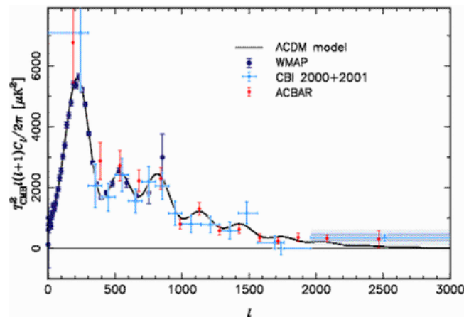
Figure 5.2: The small scale temperature angular power spectrum observed by CBI “mosaic” during two years and by ACBAR. The shaded region shows the excess power at small scale, compatible with the SZ effect. Reprinted from Readhead et al. (2004).
