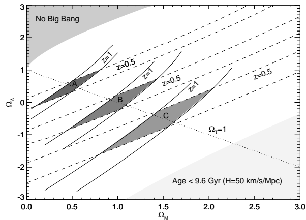
Figure 1.1: Illustration of the determination of (\Omega_m, \Omega_\Lambda) using supernovæ data: the dashed (solid) curves are lines of constant D_L for the given measured apparent magnitude of a standard candle at a redshift z = 0.5 ( z = 1.0 ). If the apparent magnitude m can be measured with accuracy \Delta m = 0.05 combining the two observations gives the dark shaded allowed region for (\Omega_m, \Omega_\Lambda) . Figure reprinted from Goobar & Perlmutter (1995).
