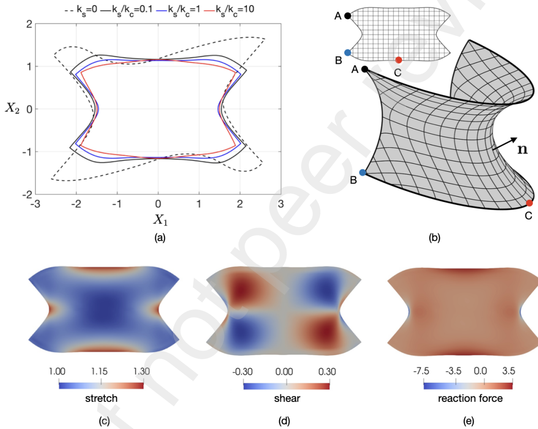
Figure 8: Clothing the hemicatenoid with an elastic fabric. (a) Optimal patch shape resulting for different values of the ratio k_s/k_c . (b) Deformed shape of the optimal textile patch onto the target surface in the case of k_s/k_c = 1 . (c)-(d)-(e) Spatial distribution of the resulting stretch \lambda_1 , shear angle \gamma , and non-dimensional normal reaction force \tau/k_c in the case of k_s/k_c = 1 . For the initial condition we set \psi(0) = \{0.5\theta_1, 0.5\theta_2\} .
