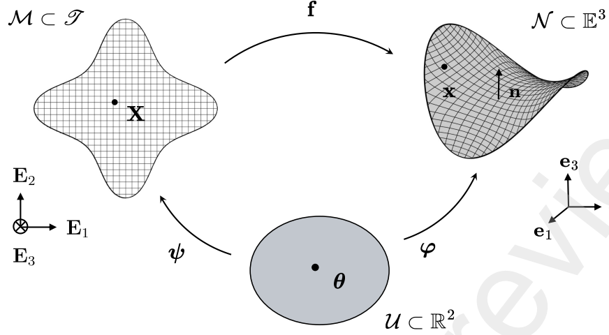
Figure 2: Commutative diagram relating the parameter set \mathcal{U} , the material manifold \mathcal{M} , and the target surface \mathcal{N}
