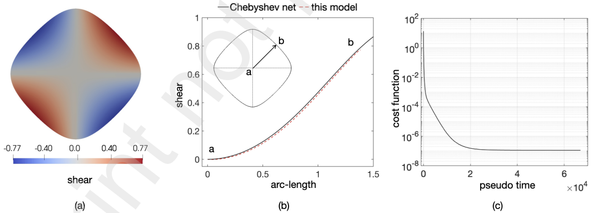
Figure 5: Clothing a unit-hemisphere with a Chebyshev net. (a) Spatial distribution of the shear angle \gamma for the optimal patch shape. (b) Plot of the shear deformation \gamma along the reference line ab and comparison with the Chebyshev net model Eq. (27). (c) Evolution of the non-dimensional cost function of \mathcal{C}/(2\pi k_c) versus the pseudo-time.
