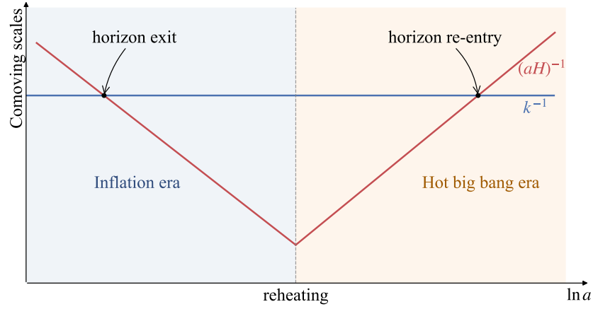
Figure 2.2. Comoving scales evolution during and after the inflationary period. Scales are initially into the horizon and thus in casual connection. Inflation stretches the scales and make them exit the horizon, where they are not casually connected any more, and remain frozen. Finally, scales re-enter the horizon during the hot Big Bang era. Figure from [177].
