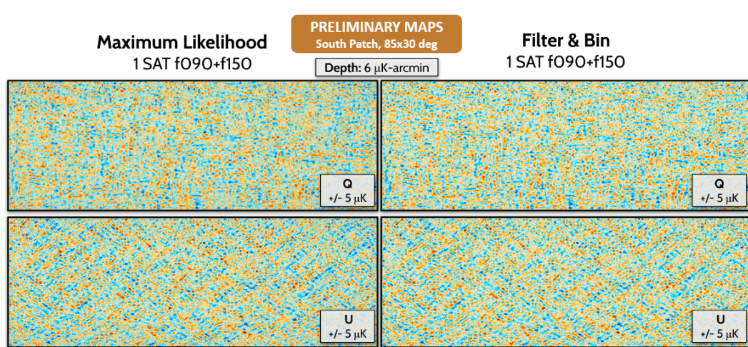
Figure 5.3. Small cutout of the preliminary SO CMB maps in polarisation, as observed by one of the SAT, co-added from the 90 and 150 GHz bands, and including data from \sim 14 months of observations. Left and right columns show the maps produced with two different, independent map-making algorithms, namely maximum likelihood and filter and bin, giving consistent results. Figure credit: SO Collaboration.
