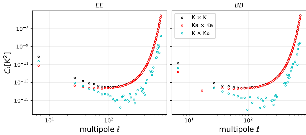
Figure 6.10. EE (left) and BB (right) auto- (black and red) and cross-frequency (cyan) angular power spectra of WMAP data, evaluated adopting the mask covering the Galactic plane, point sources, and other polarised structures (right panel of figure 6.5).
