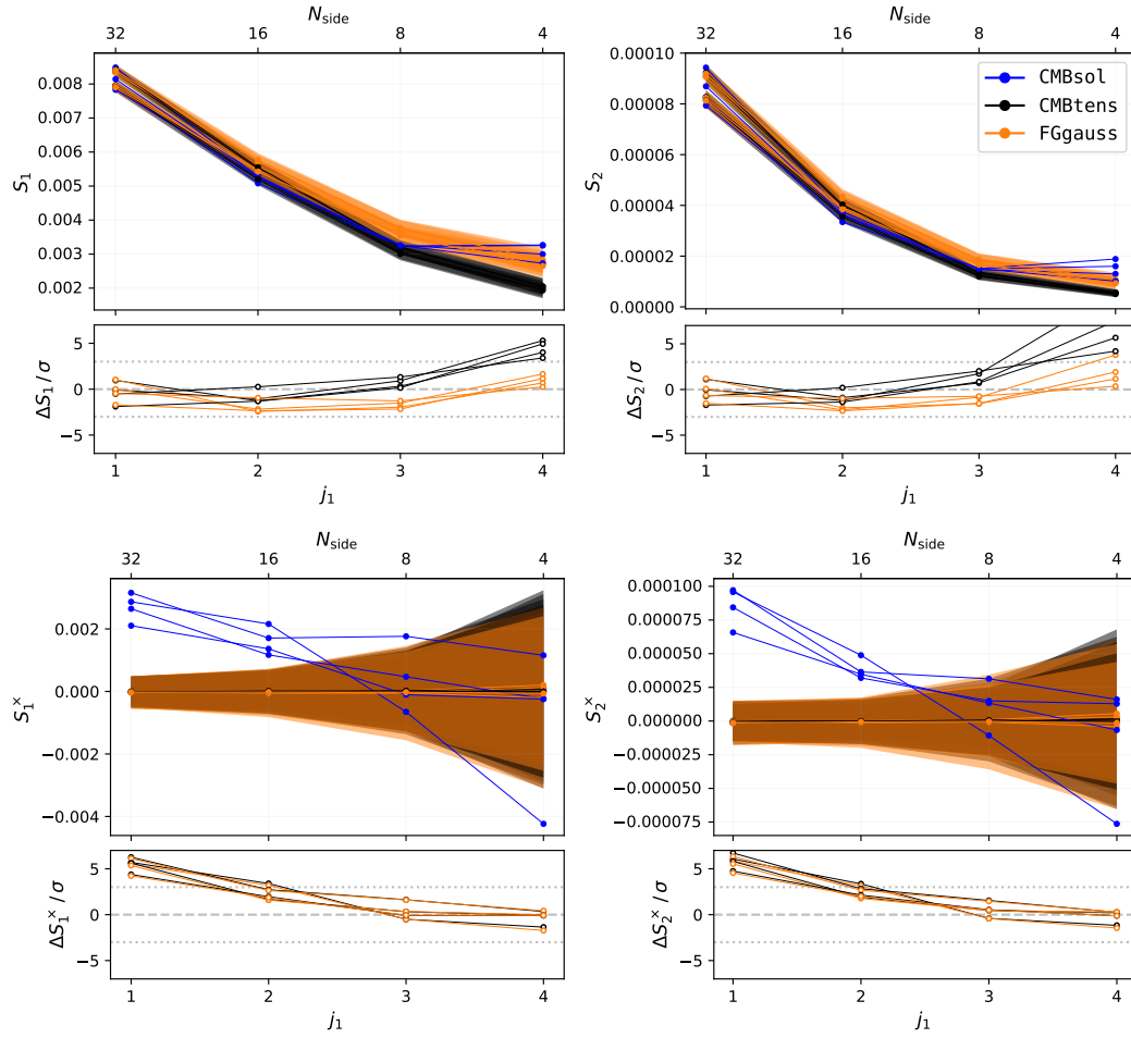
Figure 9.15. Scattering coefficients for the d10s5 model with r_{\text{in}} = 0 , one simulation. Same-coloured lines represent different orientations. Coefficients of the component-separated CMB map are in blue, while black (orange) stands for the average coefficients of the CMBtens (FGgauss) Gaussian simulations. The secondary x -axis shows the N_{\text{side}} of the maps for scale j . Upper figure: auto-coefficients, using NILC. Lower figure: cross-coefficients, correlating with 40 GHz data, using MC-NILC. Top panels: coefficients, with the shaded areas indicating the standard deviation of the Gaussian simulations \sigma . Bottom panels: normalised difference between coefficients of CMBso1 and of Gaussian maps, with the dotted lines indicating the \pm 3\sigma region.
