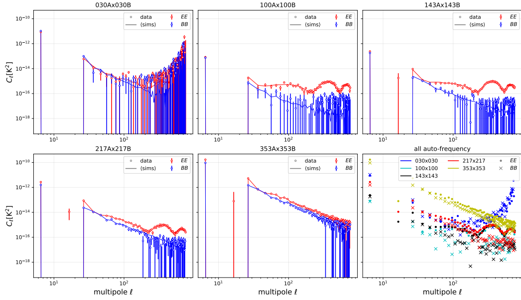
Figure 6.7. Same as figure 6.6, but here spectra are evaluated on the SO SATs sky patch of figure 6.3.
