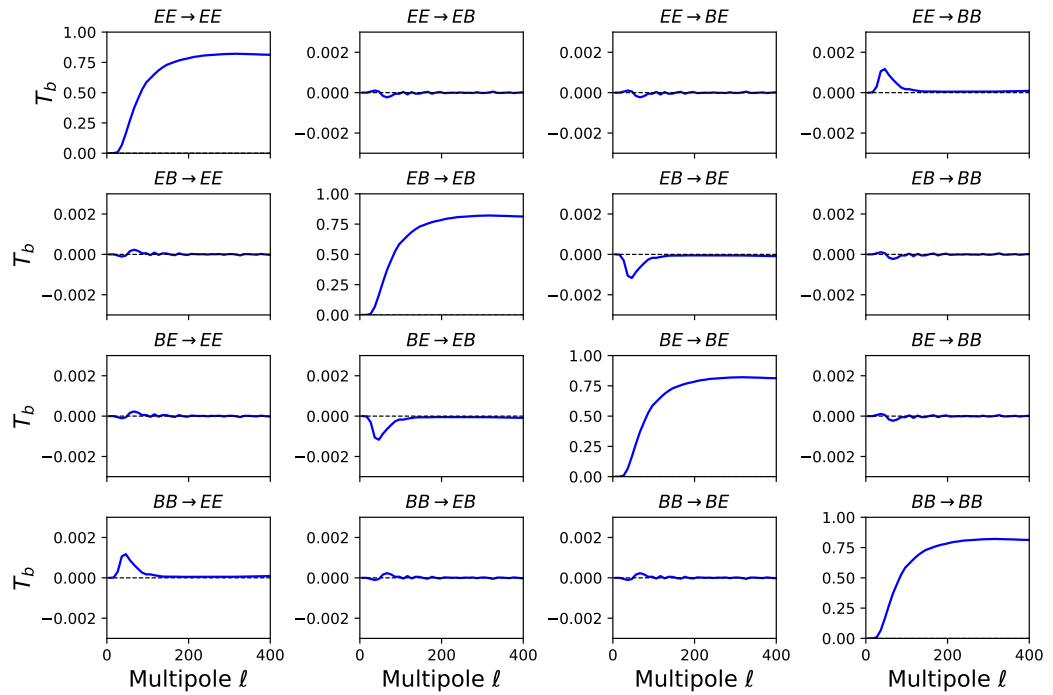
Figure 7.3. An example of transfer function for a 90 GHz SATs-like channel, showing the 16 X'Y' \rightarrow XY polarisations, averaged over N = 100 realisations of the power-law simulations shown in figure 7.2. The (very thin) shaded area represents the standard deviation divided by \sqrt{N} . This transfer function is estimated using more aggressive filtering than what expected in the real SO data analysis. Figure from [101].
