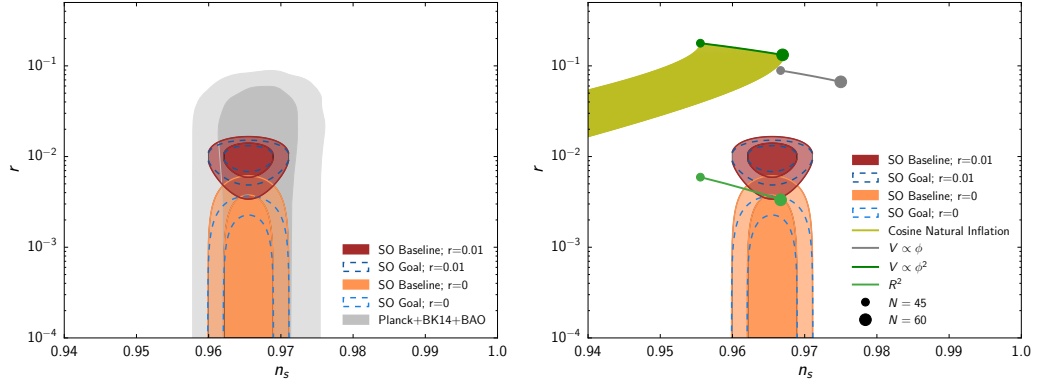
Figure 5.2. Left: summary of SO forecasts for the primordial power spectrum parameters n_s and r for two example cases: vanishingly small primordial tensor modes and primordial perturbations with r = 0.01 . The contours correspond to 68% and 95% confidence levels. The SO baseline (goal) forecasts are shown as filled (dashed) contours. Constraint in this parameter space from Planck , BICEP2/Keck , and BAO are shown in grey. Right: same as above, with predictions for n_s and r from some inflationary models.
