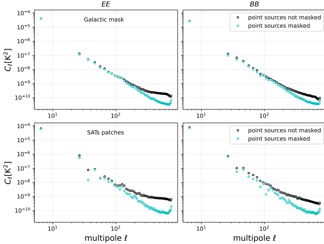
Figure 6.11. EE (left column) and BB (right column) auto-angular power spectra of S-PASS data. Spectra in top panels are evaluated on the mask covering the Galactic plane, while the ones in the lower panels are computed on the SO SATs sky patches. For black circles, point sources are included in the analysis, while for cyan circles point sources are masked out. The improvement in removing the flattening due to polarised point sources is evident.
