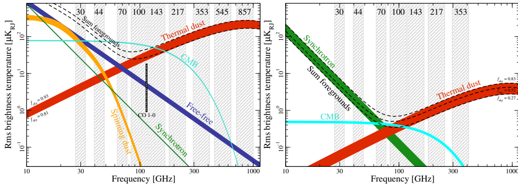
Figure 4.1. Frequency dependence of the main components of the sub-millimetre sky in temperature ( left ) and polarisation ( right , shown in P ). The vertical grey bands indicate the Planck channels, while the coloured bands show the major signal and foreground components. For temperature, the widths of the bands show the range for sky masks with 81-93% sky coverage. For polarisation, the range is 73-93%. Figure from [168].
