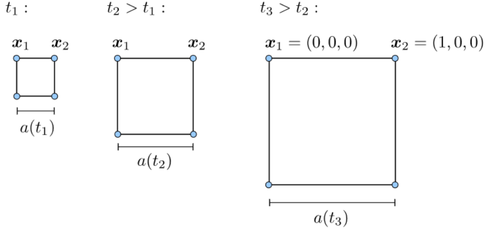
Figure 1.1. Expansion of the Universe. The comoving distance between points x_1, x_2 on a grid remains constant as the Universe expands. The physical distance is proportional to the comoving distance times the scale factor a(t) . Figure taken from [62].
