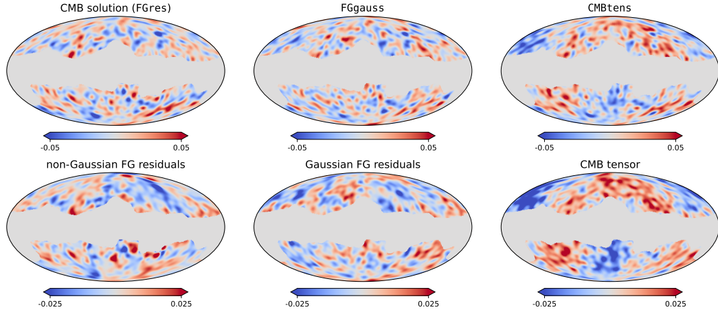
Figure 9.13. Same maps as figure 9.12, but filtered with the first needlet band b_0 to retain only the largest scales, at multipoles \ell \lesssim 60 .
