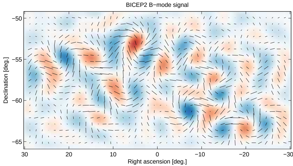
Figure 8.1. B -mode signal reported by the BICEP2 collaboration in 2014, with the black rods indicating the polarisation amplitude in different spots of the sky region observed by the telescope. Figure taken from the BICEP2 2014 Release Image Gallery, realised using data from [4].
