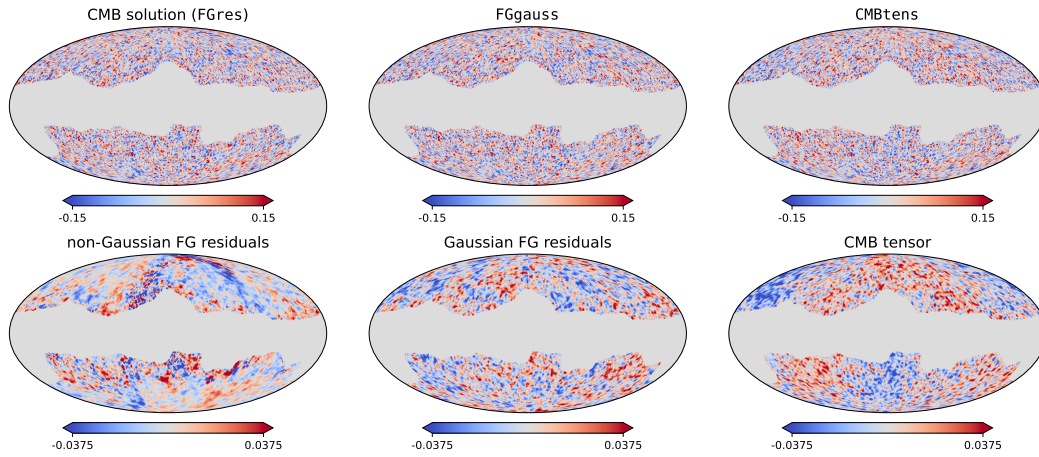
Figure 9.12. An example of the maps considered for the robustness tests, for the MC-NILC - d10s5 case. Upper row, from left to right: CMB solution (CMB so1 ), Gaussian simulations FG gauss and CMB tens . Lower row, from left to right: as upper row, but without CMB lensing and noise, with non-Gaussian and Gaussian foreground residuals, and tensor perturbations.
