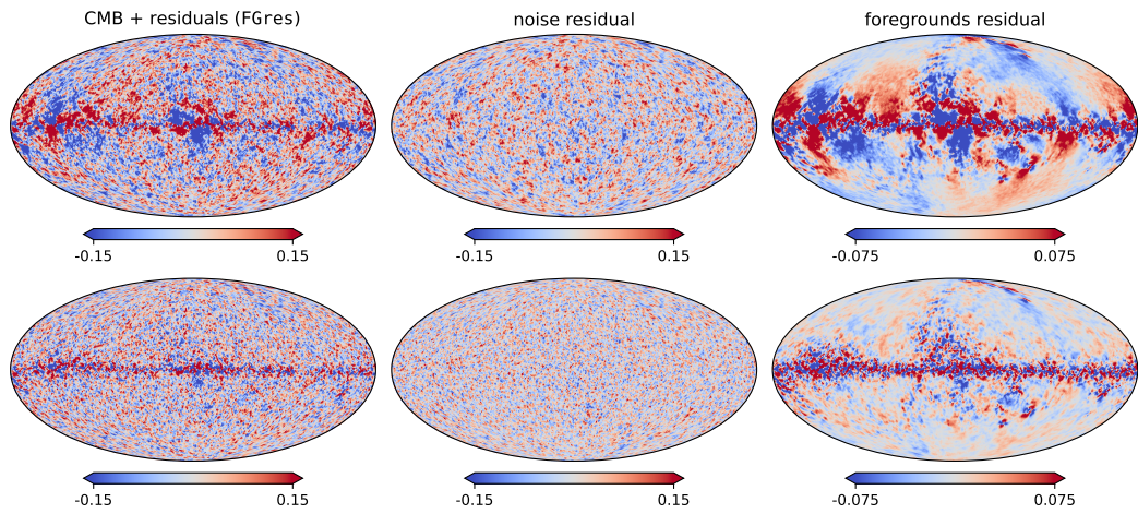
Figure 9.7. An example of the component separation outputs, for one simulation. Left column: reconstructed CMB B -mode signal (CMB solution), containing the CMB field, and noise and foreground residuals. Middle column: noise residuals. Right column: foreground residuals. Outputs are shown for NILC ( upper row ) and MC-NILC ( lower row ) methods, applied on the d10s5 model with r_{\text{in}} = 0 . Units are \mu K_{\text{CMB}} .
