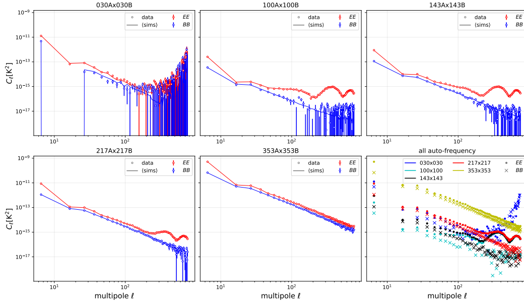
Figure 6.6. EE and BB auto-frequency angular power spectra of Planck NPIPE data, evaluated adopting the mask covering the Galactic plane, point sources, and other polarised structures (right panel of figure 6.5). At each frequency, cross-splits ( A \times B ) spectra are computed to avoid noise correlation bias.
