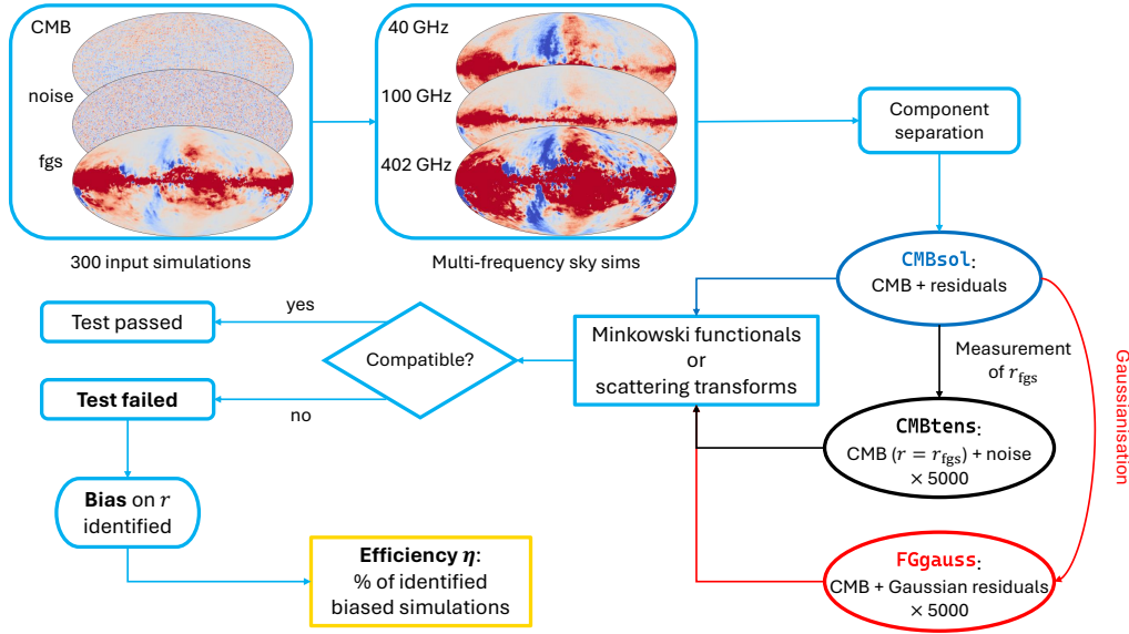
Figure 9.2. Flowchart illustrating the robustness test methodology and showing the various steps followed for the test characterisation and validation.
