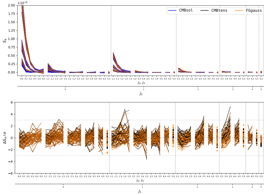
Figure 9.16. S_4 auto-coefficient for the MC-NILC - d10s5 - r_{\text{in}} = 0 scenario. Colour code is the same as figure 9.15. Lower plot shows the difference between CMBsol and Gaussian simulations, in standard deviation units, with the dotted lines indicating the \pm 3\sigma region.
