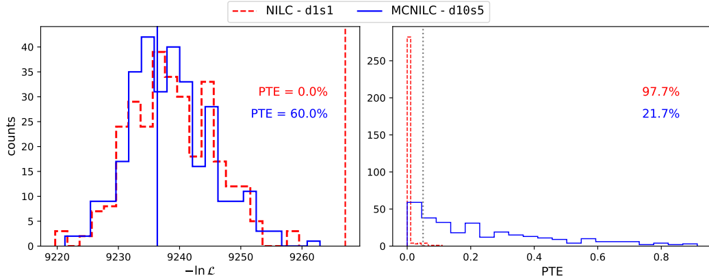
Figure 9.11. Results of the goodness-of-fit analysis for the NILC - d1s1 (red dashed lines) and MC-NILC - d10s5 (blue solid lines) cases. Left panel: one realisation of the -\ln \mathcal{L} distribution of the 300 tensor simulations, compared against the value given by the best-fit on the CMB solution (vertical lines); the corresponding PTE is also indicated. Right panel: PTE distribution for the 300 simulations, with the percentage of incompatible simulations shown on the right.
