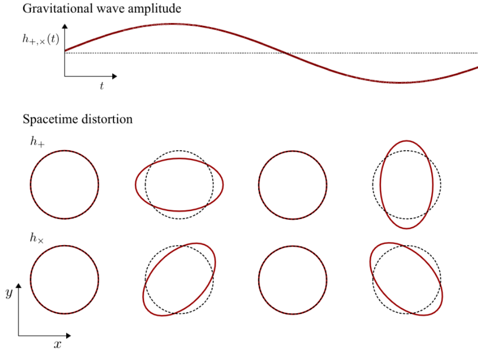
Figure 1.5. Illustration of a propagating gravitational wave (tensor mode), perturbing the spacetime. The k -vector is along the z axis, coming out of the page. The upper panel shows the time evolution of the wave amplitude (neglecting the damping due to the expansion), while the lower panel shows the stretching and compression of spacetime perpendicular to the wave's direction of propagation at the different points in time during a single wave cycle. Figure from [62].
