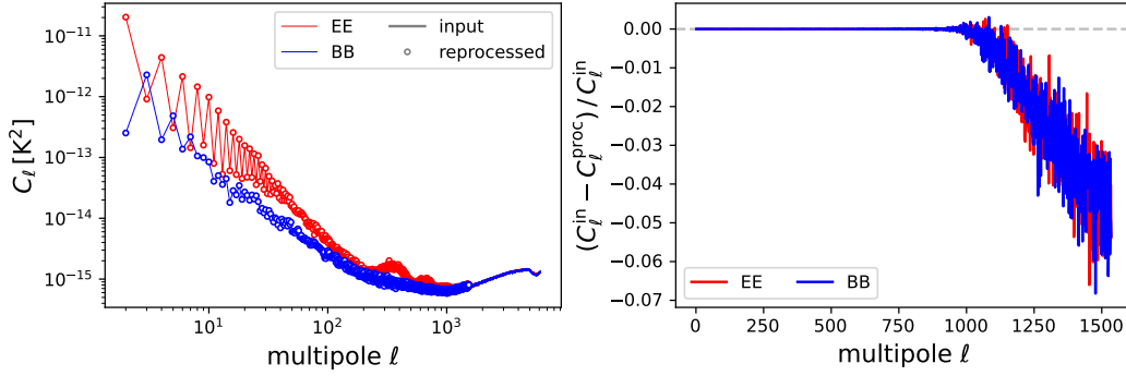
Figure 6.4. Validation of the external data pre-processing, comparing angular power spectra before (solid lines) and after (circles) the downgrading and rotation steps carried out in harmonic space ( left panel ). The spectral features are preserved, with differences ( right panel ) being at the 5% level at very small scales \ell > 1200 . Data shown are from the Planck 100 GHz channel, in EE (red) and BB (blue).
