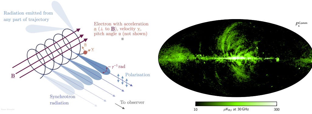
Figure 4.2. Left: diagram showing the mechanism of synchrotron radiation emitted by an electron moving along a helical path around an ordered magnetic field. The Lorentz force is perpendicular to the magnetic field. Picture taken from [9]. Right: polarised synchrotron amplitude map by Planck , obtained with the Commander algorithm, at 40' resolution, and evaluated at the reference frequency of 30 GHz. From [169].
