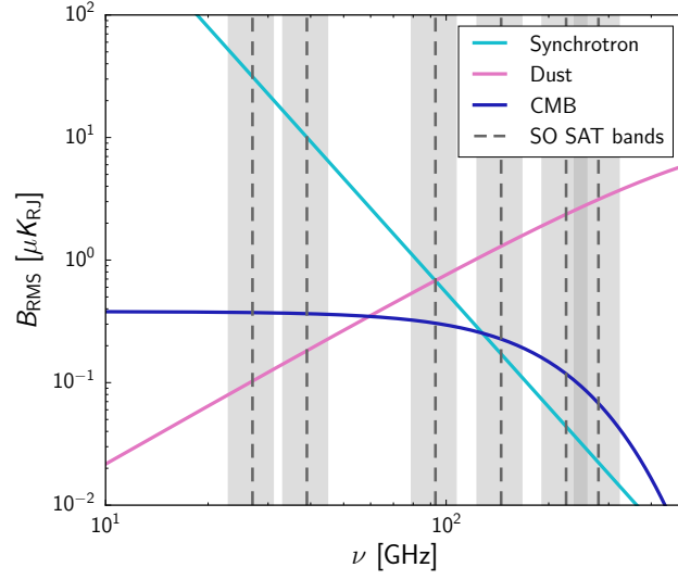
Figure 6.1. Frequency dependence, in Rayleigh-Jeans (RJ) brightness temperature, of the synchrotron and thermal dust emission at degree scales within the SATs footprint, compared to the CMB lensing B -mode signal. The turnover of the modified blackbody law for dust lies above this frequency range. The SATs channels are shown as vertical bands. Figure from [6].
