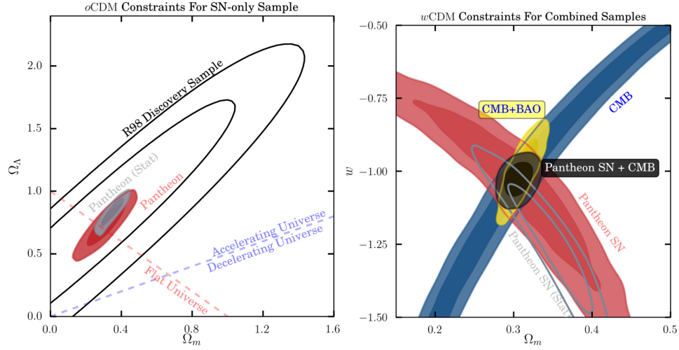
Figure 1.2. Constraints on the energy densities of matter ( \Omega_m ) and dark energy ( \Omega_\Lambda ), and the dark energy equation of state parameter ( w ). Left: constraint contours for \Omega_m and \Omega_\Lambda , from a recent analysis of type Ia supernovae distances, allowing for an open Universe. Filled contours are the more recent results, while the black lines show constraints from the original 1998 sample of [183]. Dashed lines indicate the parameters combination to have a flat Universe and the separation between an accelerating or decelerating one. Data clearly prefer a flat, accelerating scenario. Right: contours for w and \Omega_m , using type Ia supernovae, CMB, and BAO measurements, and assuming a flat Universe. The combination of different probes points to the cosmological constant ( w = -1 ). Both figures are from [189].
