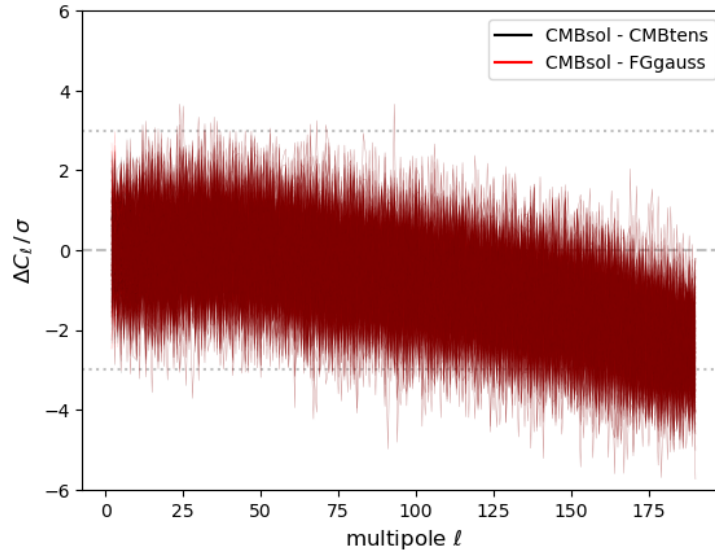
Figure 10.6. Weighted difference between the cross-40 GHz angular power spectrum of \text{CMB}_{\text{sol}} maps and of Gaussian simulations, in units of the standard deviation of the simulations \sigma . The foregrounds model under study is \text{d0s0} , and the input tensor-to-scalar ratio r_{\text{in}} = 0 is correctly recovered without bias. The observed negative trend is due to noise correlation between residuals and input data. See text for details.
