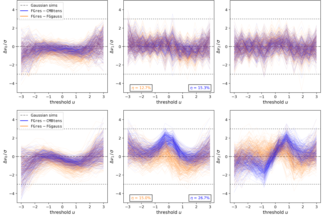
Figure 10.1. MFs weighted difference for the MC-NILC - d10s5 scenario. Each line is one of the 300 input realisations. Blue (orange) lines indicate CMBtens (FGgauss) as the reference Gaussian simulations. Plots are shown for all multipoles ( upper row ) and for large scales only ( lower row ) analysis. Dotted lines delimit the \pm 3\sigma region. Efficiencies are reported in the lower corners of the middle panels.
