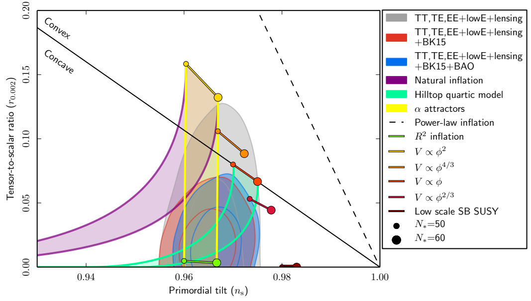
Figure 2.3. Marginalized joint 68% and 95% CL regions for n_s and r at k_p = 0.002 \text{ Mpc}^{-1} from Planck data alone and in combination with BICEP/Keck and BAO data, compared to the theoretical predictions of some inflationary models. Figure from [167].
