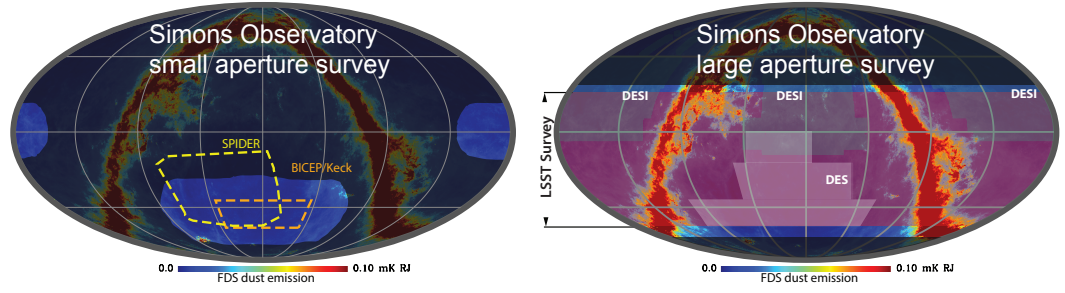
Figure 5.1. Anticipated coverage (lighter region) of the SATs ( left ) and LAT ( right ) in equatorial coordinates, overlaid on a map of Galactic dust emission. The survey regions of other experiments are also indicated. Figure from [6].
