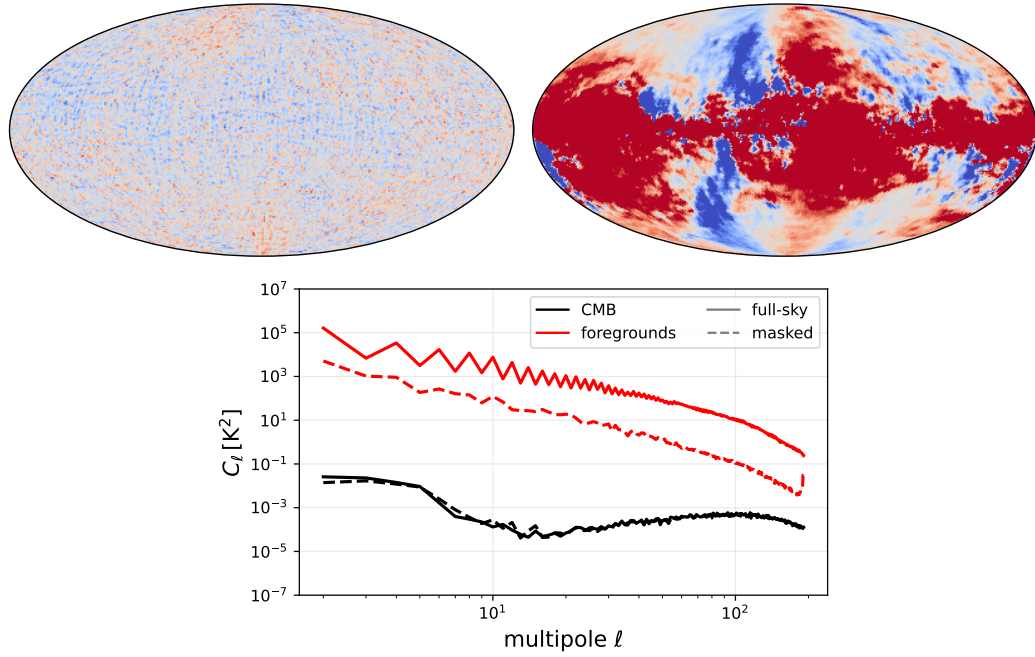
Figure 9.1. Top panels: Gaussian CMB field on the left, foregrounds map on the right, both in Stokes parameter Q . Visually, they clearly have a different morphology. Bottom panel: EE angular power spectrum of the above maps, over the full-sky or adopting a mask covering the Galactic plane. For a Gaussian field, the statistics is the same, when corrected for the sky fraction.
