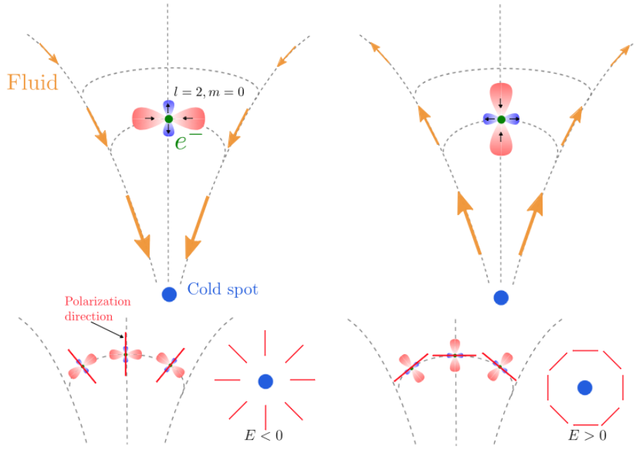
Figure 3.6. Generation of E -mode polarisation from density perturbations. The fluid either falls into the potential well while accelerating, or climbs up while decelerating (yellow arrows), creating quadrupole anisotropy in the radiation. Black arrows show the fluid motion in the electron rest frame; red lines trace the electric field direction of the radiation scattered by the electrons, resulting in positive or negative E -mode polarisation patterns. Figure from [147].
