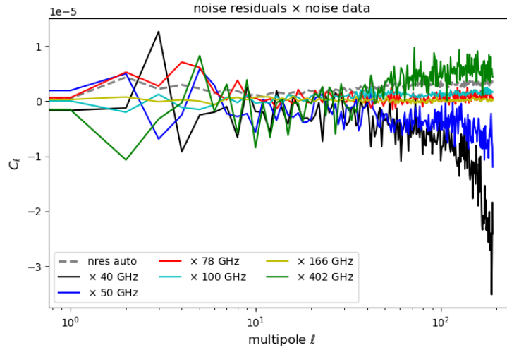
Figure 10.4. Cross angular power spectrum between noise residuals and noise maps, for different input frequency channels (in different colours), one simulation. The dashed line indicates the noise residuals auto spectrum. The considered scenario here is MC-NILC applied on the \Lambda CDM model. We notice the strong negative correlation for the 40 GHz channel.
