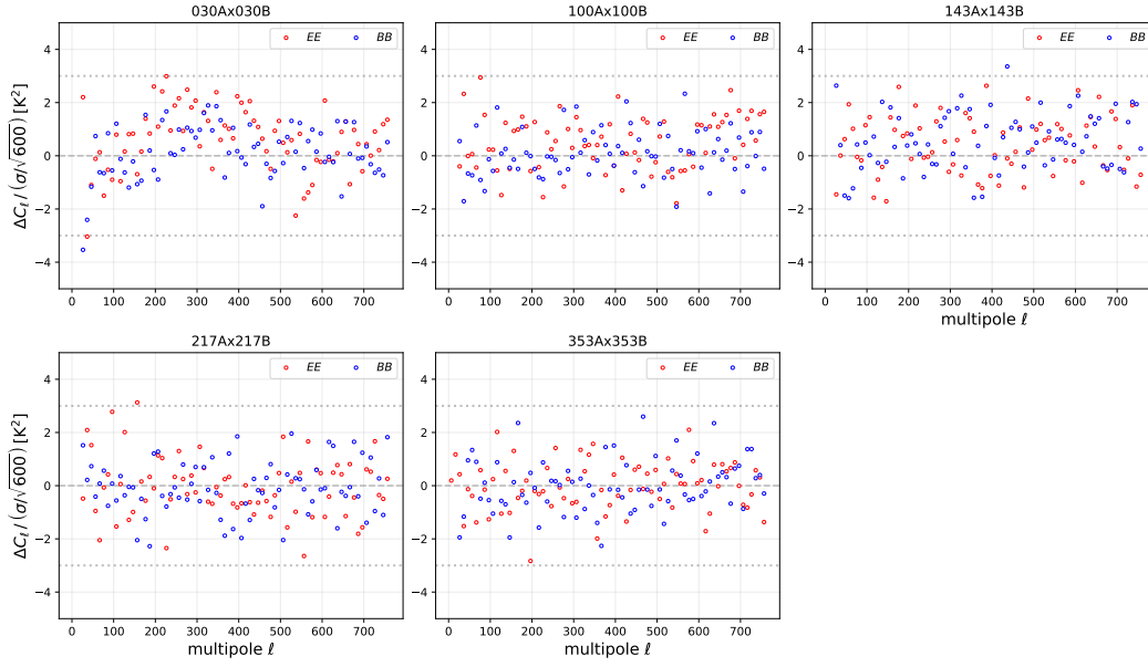
Figure 6.8. EE and BB auto-frequency angular power spectra of Planck NPIPE residuals simulation, evaluated adopting the mask covering the Galactic plane (left panel of figure 6.5). At each frequency, cross-splits ( A \times B ) spectra are computed to avoid noise correlation bias. Results are reported normalised by the error on the simulations.
