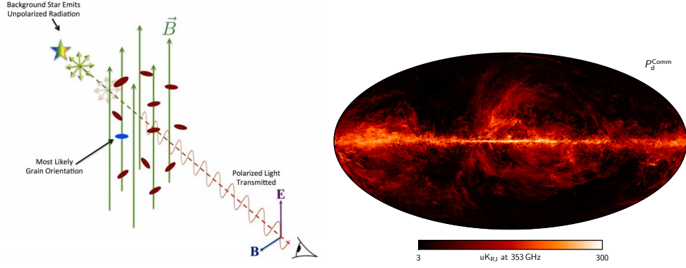
Figure 4.3. Left: diagram showing how dust clouds are able to polarise background starlight. Asymmetric and elongated grains tend to align with the direction of the magnetic field, emitting polarised radiation along the big axis of the grain. Picture from the Pasiphae website. Right: polarised thermal dust amplitude map by Planck , obtained with Commander algorithm, at 5' resolution, and evaluated at the reference frequency of 353 GHz. From [169].
