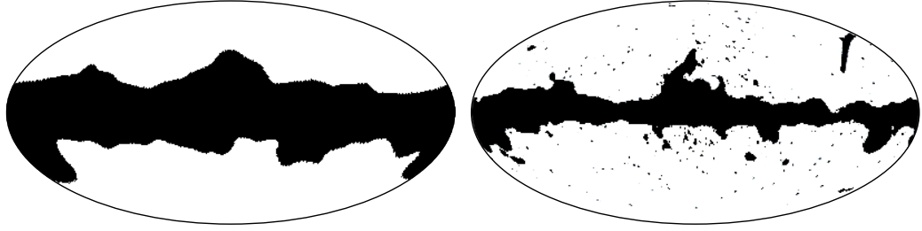
Figure 6.5. Binary version of the masks adopted for the characterisation of external data, in galactic coordinates. Left: mask covering the Galactic plane. Right: official mask used for the Planck analysis of polarised data, covering the Galactic plane, extra-galactic point sources, and other polarised structures.
