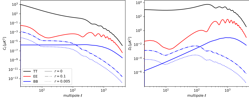
Figure 9.3. Input angular power spectra used to generate the Gaussian CMB simulations, in C_\ell (left) and D_\ell (right), adopting the best-fitting Planck 2018 parameters [166]. TT in black, EE in red, BB in blue. Solid lines represents spectra where B -modes arise from lensing only ( r_{\text{in}} = 0 ), while the dashed line show the contribution due to primordial gravitational waves for r_{\text{in}} = 5 \times 10^{-3} .
