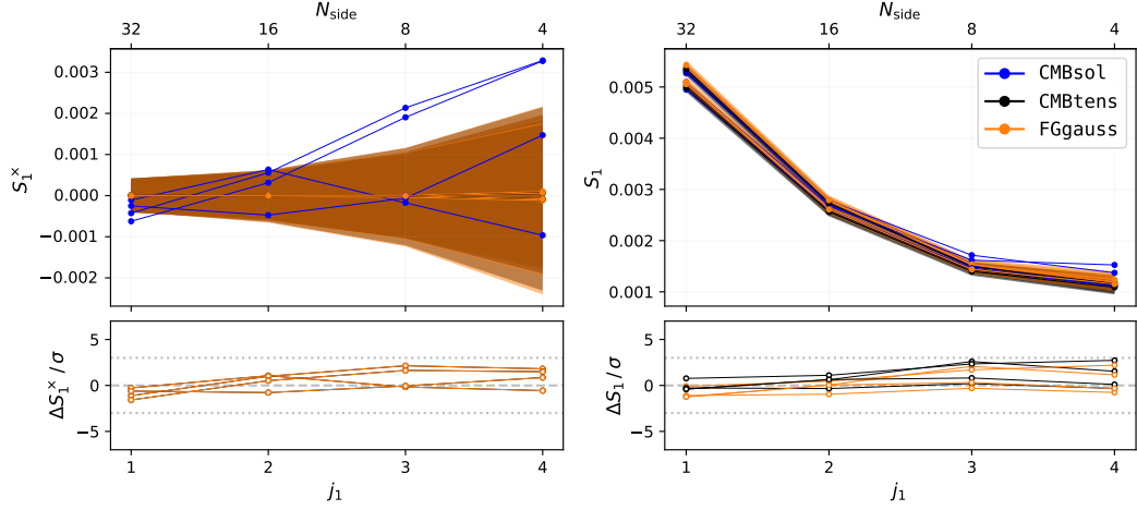
Figure 10.3. ST S_1 coefficient for two validation cases, with the same colour code of figure 9.15. Left: cross-coefficients correlating with synchrotron-dominated input data, for the MC-NILC - d0s0 - r_{\text{in}} = 0 case. Right: auto-coefficients, for the NILC - d0s0 - r_{\text{in}} = 5 \times 10^{-3} scenario. In both plots, the tensor-to-scalar ratio estimate is not biased, coefficients are compatible, and the robustness test raises no strong warnings.
