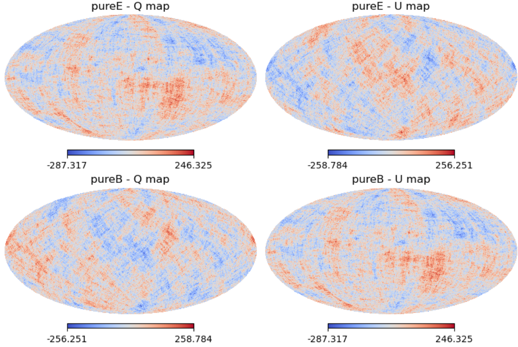
Figure 7.2. An example of Q and U maps containing E - and B -modes only. The characteristic + and \times patterns in the Q_E and Q_B maps indicate the dominance of E - and B -modes, respectively.
