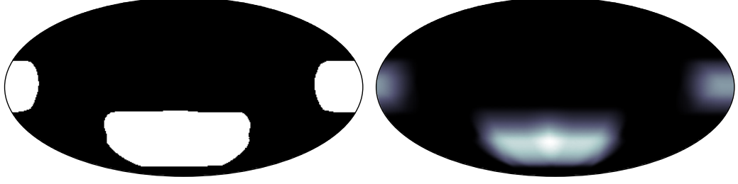
Figure 6.3. Nominal sky regions observed by the SO SATs [218], in equatorial coordinates. Unobserved pixels are in black. Left: binary mask, covering f_{\text{sky}} = 10\% of the sky. Right: apodised mask weighted by the forecasted pixel observing time. Mask edges are apodised using a C1-type kernel with an 10 degrees apodisation scale.
