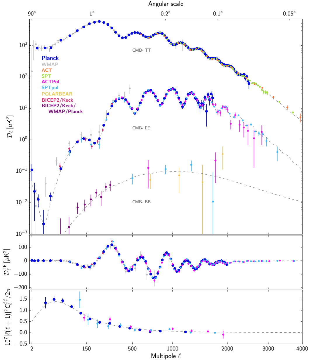
Figure 3.7. Compilation of recent CMB angular power spectrum measurements. Upper: temperature, E - and B -mode polarisation. Middle: TE cross-correlation. Lower: lensing deflection power spectrum. Different colours correspond to different experiments. The dashed line indicates the best-fit \Lambda\text{CDM} model to the Planck temperature, polarisation, and lensing data. Figure from [168].
