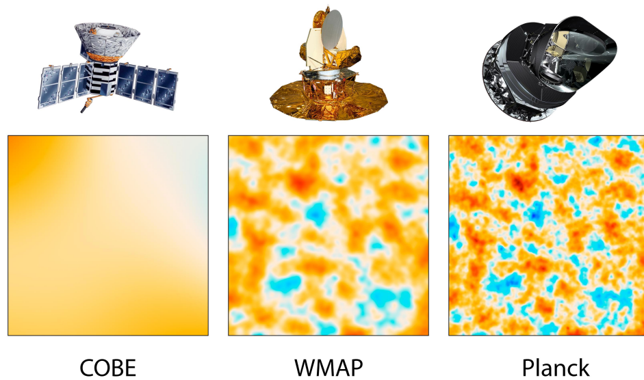
Figure 3.8. Comparison between the CMB anisotropies observed by the three satellites COBE (left), WMAP (middle), and Planck (right), showing the amazing improvement in sensitivity and resolution. The three panels show 10-square-degree patches of all-sky microwave maps. Source: link . Courtesy NASA/JPL-Caltech.
