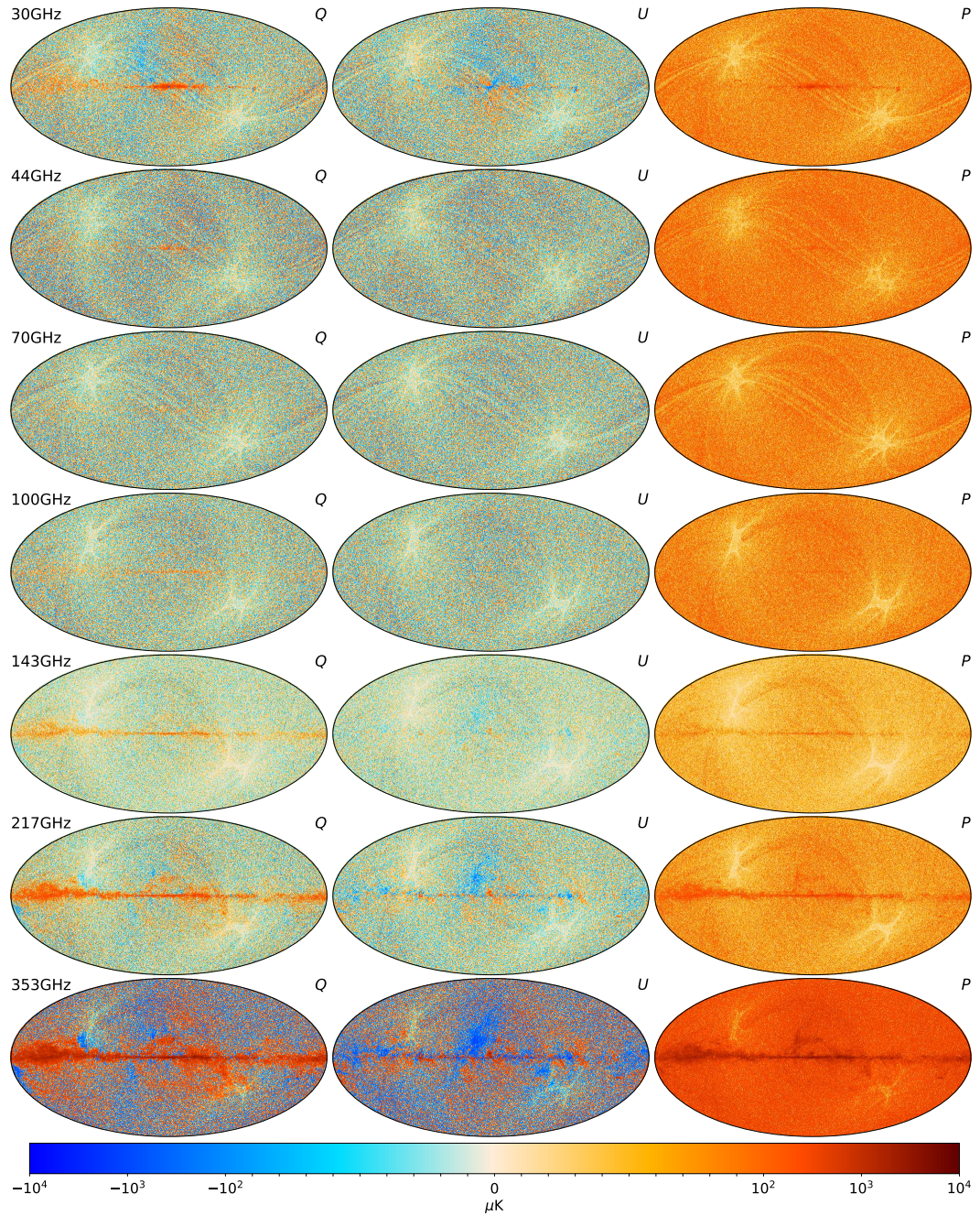
Figure 3.4. Polarised microwave sky as observed by the seven frequency bands of the Planck satellite. The first two columns show the Q and U Stokes parameters; the last column shows the polarised intensity, P = \sqrt{Q^2 + U^2} . Figure from [173].
