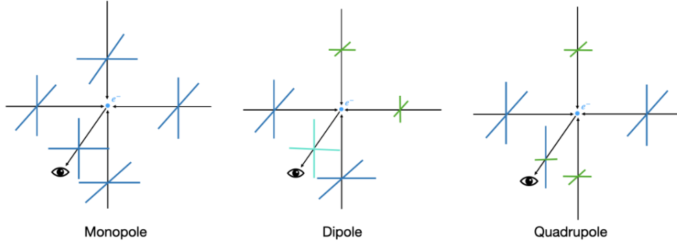
Figure 3.3. Caricature of the Thomson scattering, comparing the output linear polarisation generated by monopole, dipole and quadrupole configurations. The monopole and dipole generate unpolarised light, while the quadrupole leaves a net linear polarisation on the outgoing photons. Figure from [207].
