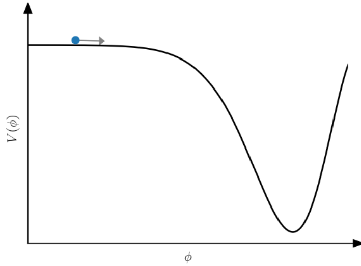
Figure 2.1. A scalar field slowly rolling down a potential V(\phi) . Since it rolls slowly, it has little kinetic energy. The potential energy is non-zero, however, so the pressure is negative. The inflationary epoch ends once the field has reached the minimum of the potential. Figure taken from [62].
