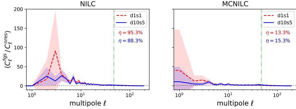
Figure 10.2. Average ratio between spectra of foreground and noise residuals. Dashed red lines indicate the d1s1 model, while blue solid lines are for d10s5. Shaded areas represent the standard deviation across 300 simulations. MFs test efficiencies are also reported for comparison. The vertical line indicates the smallest scale included in the first needlet band b_0 .
