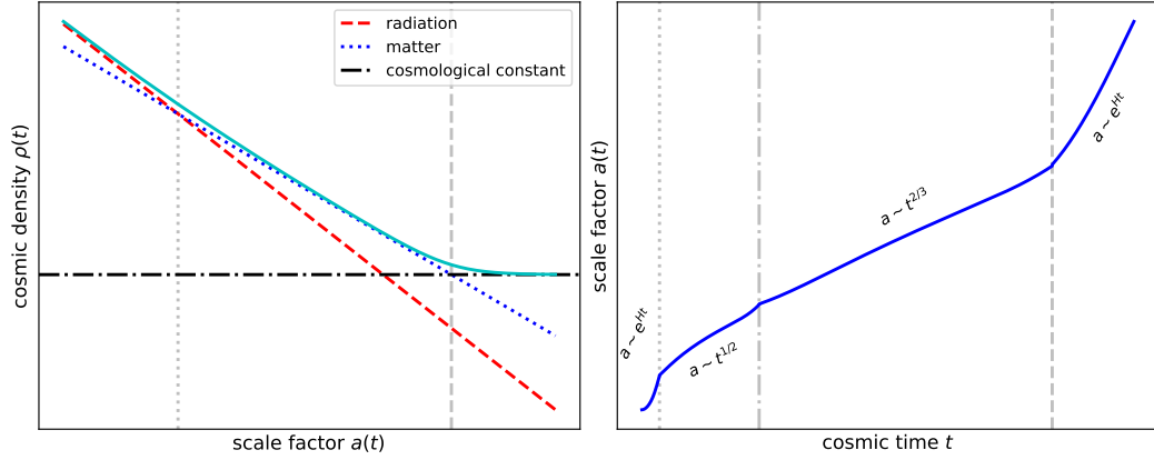
Figure 1.3. Dynamics of the Universe provided by the Friedmann equations. Left: energy density \rho as a function of the scale factor a . Different constituents of the universe dominates at different time of the history: radiation (red dashed), non-relativistic matter (blue dotted) and a cosmological constant (black dash-dotted). Right: behaviour of the scale factor a as a function of the cosmic time t , in the frame of the \Lambda CDM model.
