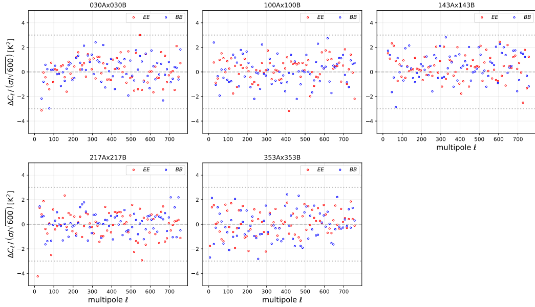
Figure 6.9. Same as figure 6.8, but here spectra are evaluated on the SO SATs sky patch of figure 6.3.
