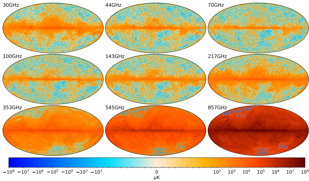
Figure 3.2. Sky emission fluctuations in each of the nine Planck frequency bands, after removal of the common dipole component. The fluctuations are expressed as equivalent temperature variations (in K_{\text{CMB}} units), so that CMB fluctuations will appear the same in each map. Figure from [173].
