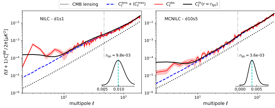
Figure 9.10. Same as figure 9.9, but considering only the largest scales in the likelihood evaluation. The maximum multipole included ( \ell = 48 ) is indicated by the vertical dash-dotted line.
