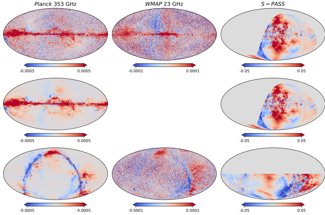
Figure 6.2. Examples of the external datasets adopted to integrate SO SATs observations, in Stokes Q maps. Units are \mu\text{K}_{\text{CMB}} . From left to right: Planck NPIPE 353 GHz channel, WMAP 23 GHz channel, and S-PASS 2.3 GHz. From top to bottom: input maps, then downgraded to N_{\text{side}} = 512 , and rotated from galactic to equatorial coordinates. WMAP data have not been downgraded as their are natively at the same resolution of the SATs.
