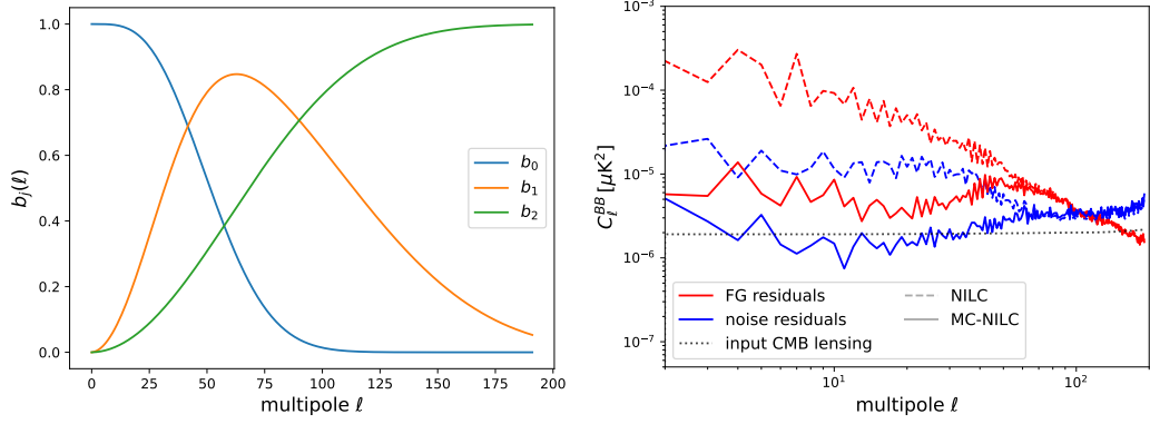
Figure 9.8. Left panel: needlet bands Mexican configuration adopted in this work for component separation, where the first bands have been merged. Right panel: full-sky angular power spectra evaluated on foreground (red) and noise (blue) residuals, for NILC (dashed lines) and MC-NILC (solid lines), applied to the d10s5 model. Black dotted line is the input CMB spectrum (lensing-only).
