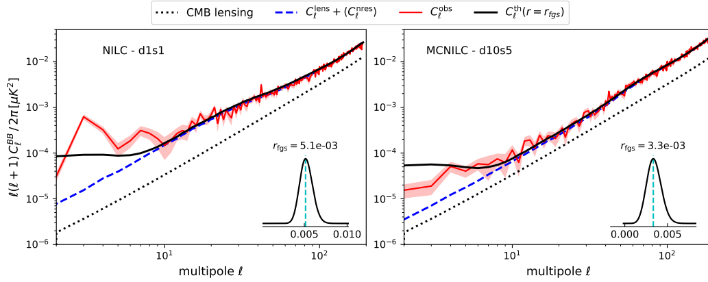
Figure 9.9. Angular power spectra going into the likelihood evaluation for a single simulation, for the NILC - d1s1 ( left ) and MC-NILC - d10s5 ( right ) scenarios. Main plot: spectra, with C_\ell^{\text{th}}(r = 0) in dashed blue, C_\ell^{\text{obs}} in solid red, C_\ell^{\text{lensing}} in dotted black, and the best-fit in solid black. The shaded area represents the standard deviation of C_\ell^{\text{obs}} across 300 realisations. Inset: normalised likelihood on the tensor-to-scalar ratio; the peak value is indicated by the dashed line.
