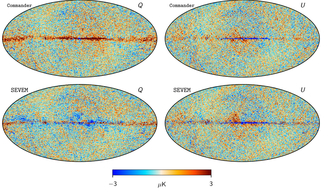
Figure 4.5. Foreground-cleaned CMB Q and U maps derived from the Planck NPIPE data set with Commander (top row) and SEVEM (bottom row), plotted with an angular resolution of 40' . From [173].
