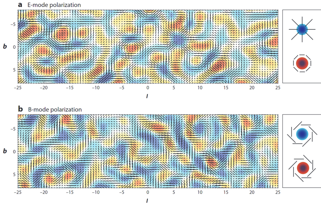
Figure 3.5. Upper panel: polarisation pattern composed only of E -modes. Lower panel: polarisation pattern composed only of B -modes. As indicated on the right, the E -mode pattern is tangential around hot spots (red) and radial around cold spots (blue). B -mode polarisation show instead a characteristic swirling pattern (with different orientations around hot and cold spots). Figure taken from [111].
