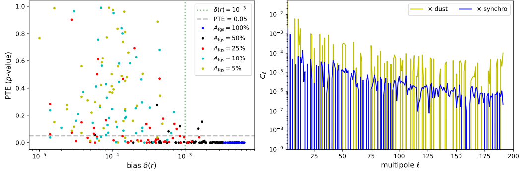
Figure 10.5. The considered scenario is MC-NILC - d10s5 - r_{\text{in}} = 0 . Left: probability-to-exceed (PTE, or p -value) given by the compatibility analysis for the cross-synchrotron test using the S_1 and S_2 coefficients, as a function of the bias on the tensor-to-scalar ratio r . Results are shown for 50 simulations and for different values of foregrounds rescaling A_{\text{fgs}} . The dotted vertical line is a reference value of \delta(r) = 10^{-3} , while the horizontal dashed line is the PTE threshold for incompatibility: ST coefficients are compatible above 0.05, and incompatible below, when foreground contamination is detected. Right: cross-angular power spectrum between CMB s01 and foreground maps; cross-correlation with dust is indicated in yellow, while blue is for synchrotron. See text for discussion.
