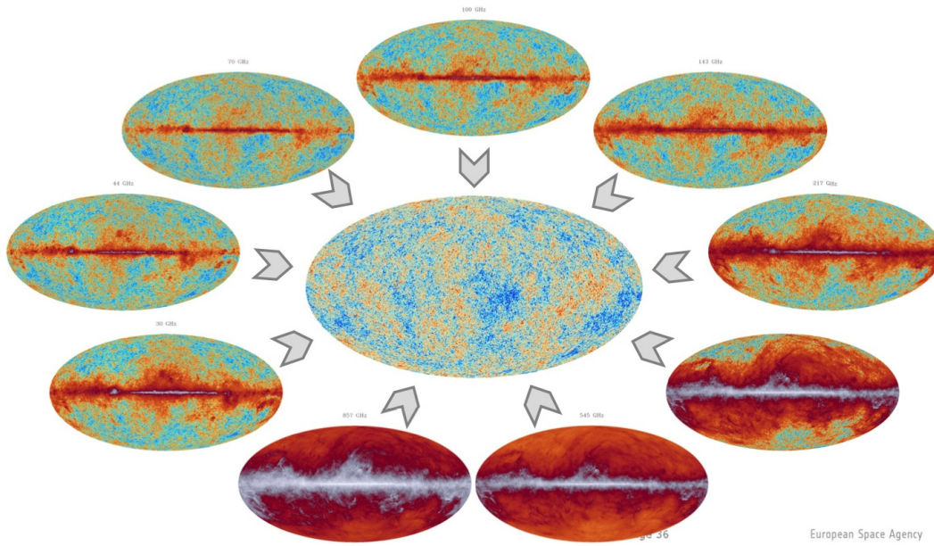
Figure 4.4. Diagram illustrating the component separation principle, combining Planck multi-frequency sky maps (in temperature) to obtain a foreground-cleaned CMB reconstruction. From this website.
