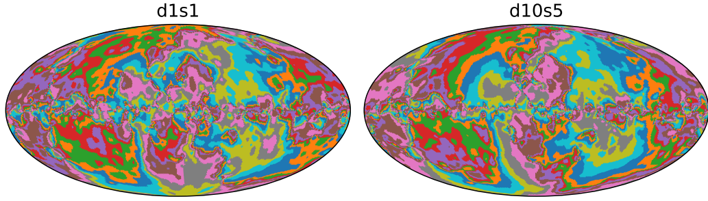
Figure 9.6. Sky partitions adopted in the MC-NILC component separation for d1s1 ( left ) and d10s5 ( right ) foreground models.
