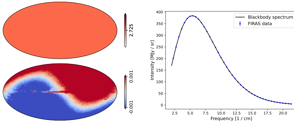
Figure 3.1. Left: monopole and dipole maps of the CMB intensity. Upper panel illustrate the smooth isotropic CMB temperature T_{\text{CMB}} \simeq 2.725 K, almost the same in every pixel. The lower panel shows a Planck intensity map at a frequency of 100 GHz [173], after removal of the monopole, in \text{K}_{\text{CMB}} units. The dipole anisotropy is evident in the hotter and colder regions, typical of a Doppler shift. Right: the monopole spectrum of the CMB, from the original data by the FIRAS instrument of the COBE experiment [140, 219, 78], available at this link. The vertical axis is in surface intensity units, while the horizontal axis is the reciprocal of the microwave wavelength, proportional to the frequency. The black curve shows the expected intensity from a single temperature blackbody spectrum at T = 2.725 K. The error bars are there in the plot, smaller than the line width (!).
