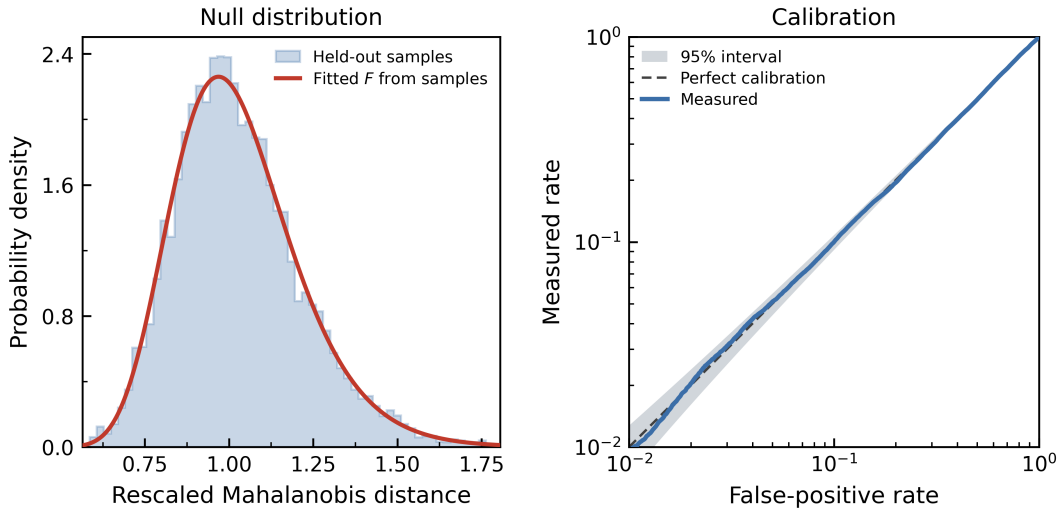
Figure 9.17. Check of the calibration of the compatibility analysis for the ST-based test, on held-out reference simulations not used in the fit. The considered foreground model is d0s0 , with r_{in} = 0 , using the S_1 and S_2 coefficients combined together. Left: rescaled Mahalanobis distances against the fitted F distribution. Right: measured rejection rate versus theoretical false-positive rate (blue), with the perfect-calibration diagonal (dashed) and its 95% interval (grey).
