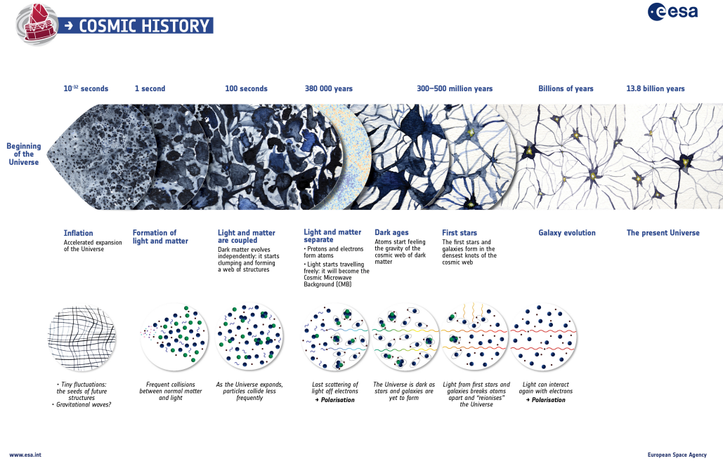
Figure 1.4. Simplified chronology of the Universe, as per the \Lambda CDM concordance model. The timeline in the upper part shows an artistic view of the evolution of the cosmos on large scales, passing through inflation, CMB emission, "Dark Ages", birth of the first stars and galaxies, and until present time. The inserts below show some of the microscopic processes taking place during cosmic history. Credit: ESA.
