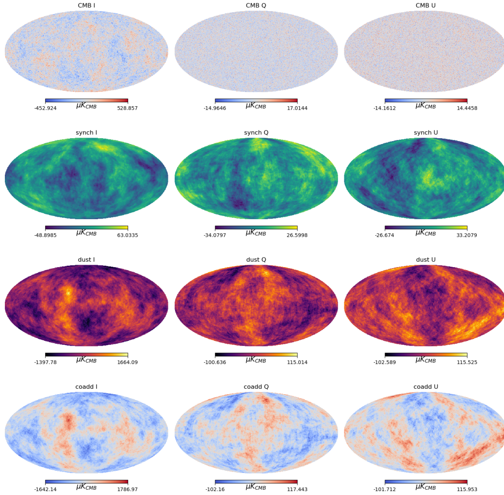
Figure 7.1. Example of sky maps simulated for the purpose of covariance matrix estimation, at a frequency of 353 GHz. From left to right : total intensity I , and Stokes Q and U maps. From top to bottom : CMB, synchrotron radiation, dust emission, and all the above co-added maps. At the selected frequency, thermal dust is the dominant component. Units are \mu K_{CMB} .
