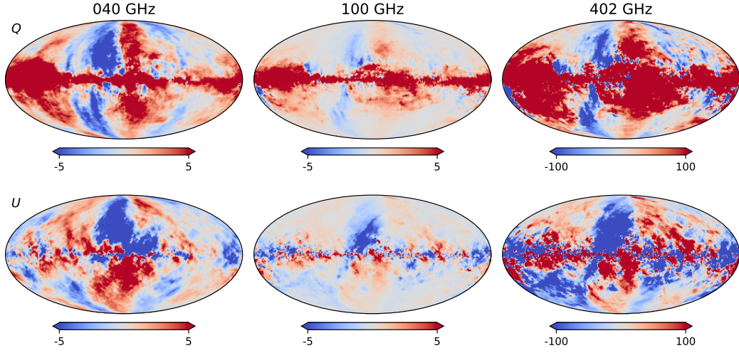
Figure 9.5. Simulated polarised foreground emission maps, in Q (top row) and U (bottom row) Stokes parameters, for the \mathbf{d10s5} model, at synchrotron-dominated (40 GHz, left column ), foregrounds-minimum (100 GHz, middle column ), and dust-dominated (402 GHz, right column ) frequencies. All maps are smoothed to 70.5 arcmin, and reported in \mu\text{K}_{\text{CMB}} units.
