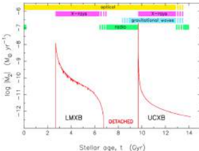
Fig. 8 Evolutionary sequence showing how ultra-compact X-ray binaries (prime LISA source candidates) are formed from merging NS+WD binaries, descending from LMXBs. Plotted here is mass-transfer rate of the donor star as a function of stellar age. The initial MS star + NS binary has components of 1.40 M_{\odot} and 1.30 M_{\odot} , respectively. The system evolves through two observable stages of mass transfer: an LMXB for 4 Gyr, followed by a detached phase lasting about 3 Gyr where the system is detectable as a radio millisecond pulsar orbiting the helium WD remnant of the donor star, until GW radiation brings the system into contact again, producing a UCXB. The colour bars indicate detectability in different regimes resulting in synergies between LISA and EM detectors. Image reproduced with permission from Tauris (2018), copyright by APS
