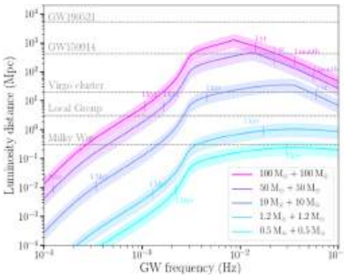
Fig. 1 Distance to which LISA binaries can be detected as a function of GW frequency. The coloured lines represent the SNR threshold of 7 (here computed assuming a mission duration of 4 year with 100% duty cycle) for (quasi-)stationary equal-mass circular binaries of different total masses in the distance–GW frequency parameter space. The shaded range represents angle-averaged curve limits for the optimal and worst binary orientation. The ticks on the curves represent binary merger times: for merger times \gg 4 year the binary will be seen by LISA as a monochromatic GW source, whereas for merger times < 4 year the binary will be seen as evolving. Note in particular that evolving sources like GW190521 and GW150914 remain within the LISA band for less than the mission lifetime. Image credit: Antoine Klein & Valeriya Korol
